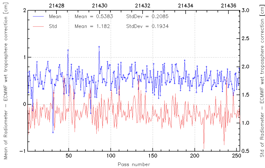
FIG. 11 – Pass monitoring of wet troposphere differences between radiometer and ECMWF model for Jason-2 cycle 006.
