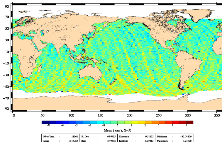
FIG. 20 – Jason-1 – Jason-2 SLA differences (without corrections) for cycle 006.
