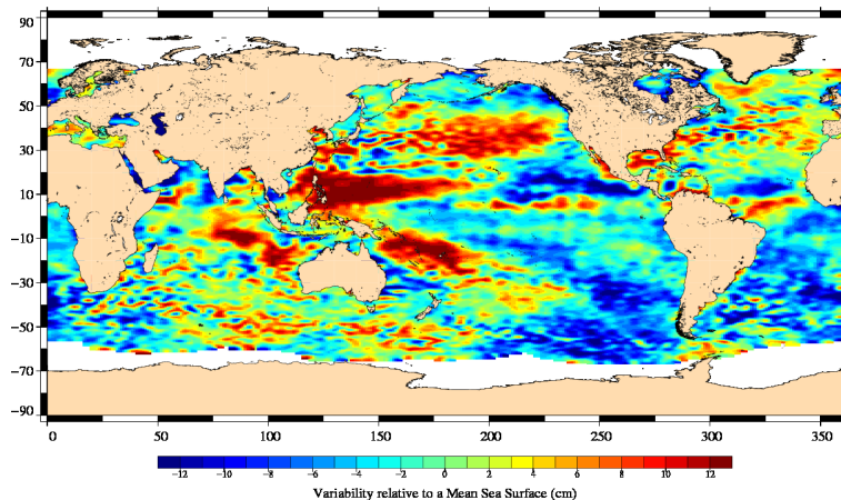
FIG. 18 – Sea level anomaly relative to MSS for cycle 006.
