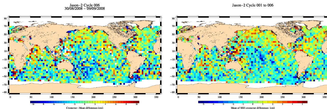
FIG. 13 – Mean SSH at crossovers for cycle 006 (left) and over the whole Jason-2 period (right).
