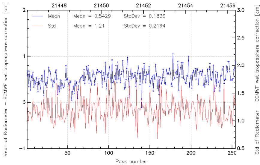
FIG. 11 – Pass monitoring of wet troposphere differences between radiometer and ECMWF model for Jason-2 cycle 008.
