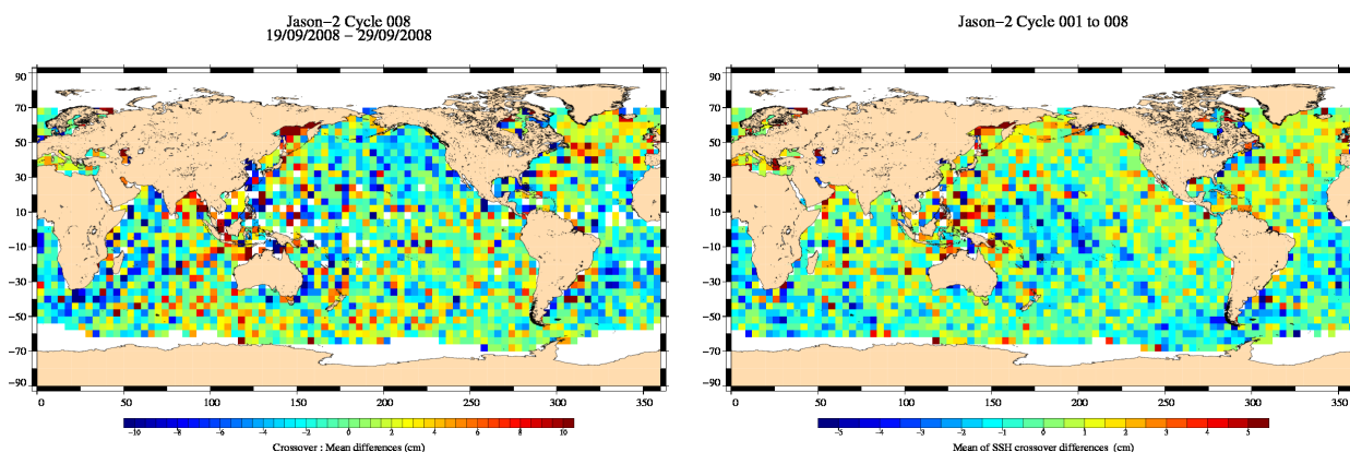
FIG. 13 – Mean SSH at crossovers for cycle 008 (left) and over the whole Jason-2 period (right).
