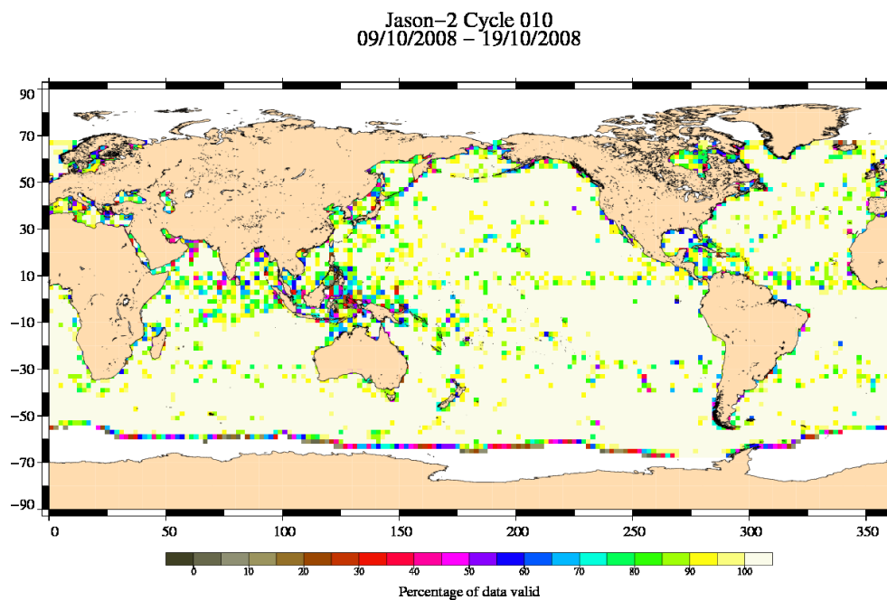
FIG. 3 – Percentage of valid measurements for cycle 010.
