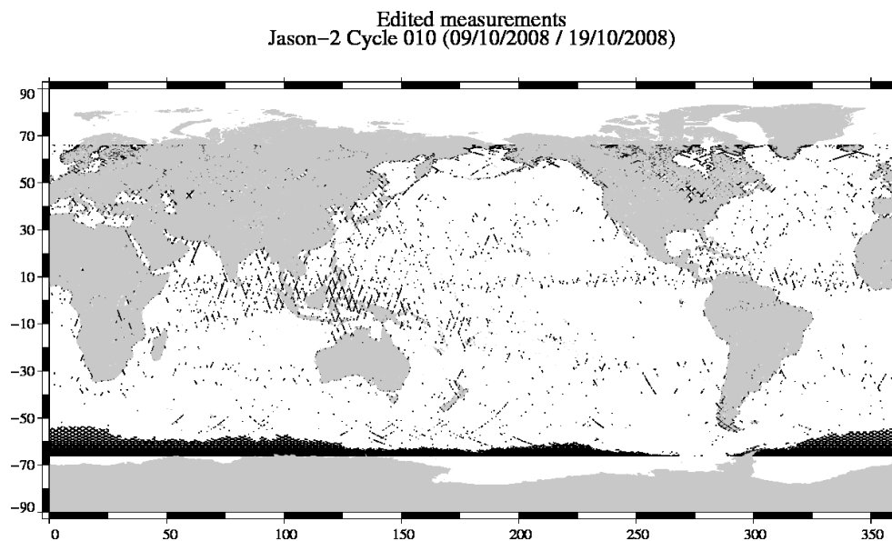
FIG. 2 – Edited measurements for cycle 010.
