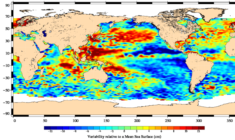
FIG. 18 – Sea level anomaly relative to MSS for cycle 010.
