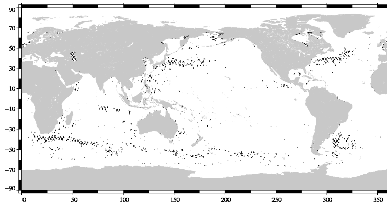
FIG. 19 – Differences higher than a 30 cm threshold for cycle 010.
