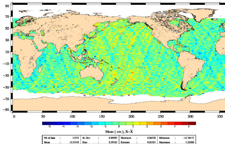
FIG. 20 – Jason-1 – Jason-2 SLA differences (without corrections) for cycle 010.
