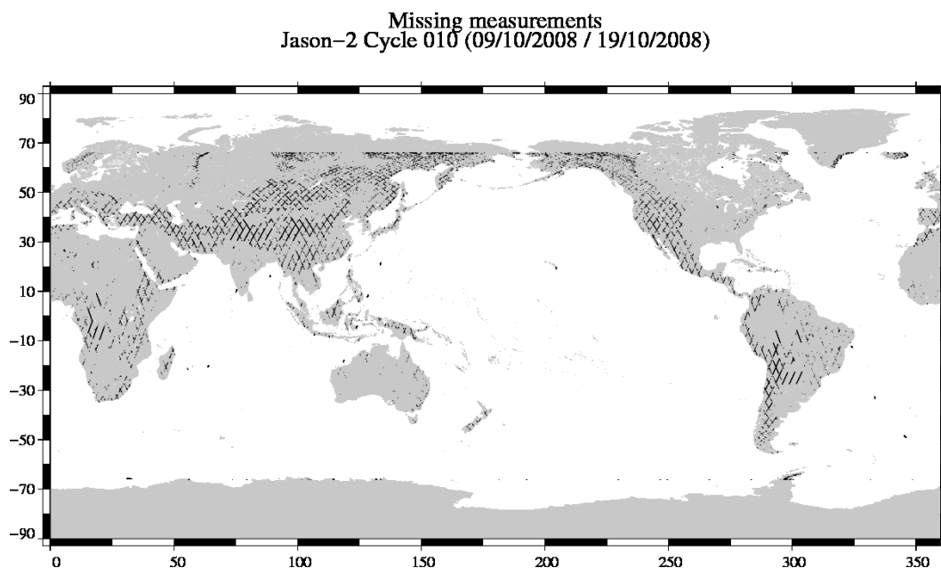
FIG. 1 – Missing measurements for cycle 010.
