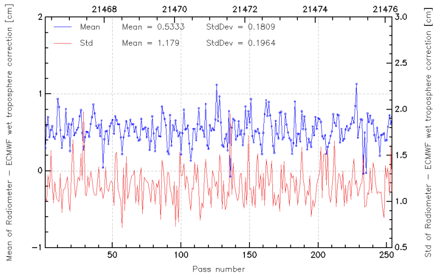
FIG. 11 – Pass monitoring of wet troposphere differences between radiometer and ECMWF model for Jason-2 cycle 010.
