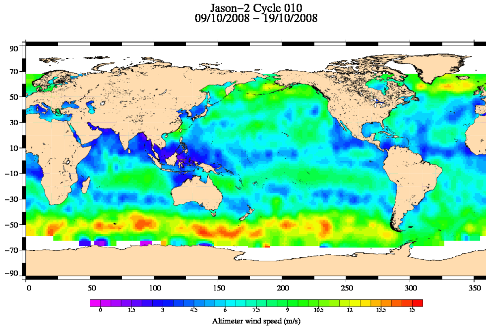
FIG. 9 – Altimeter wind speed for cycle 010.
