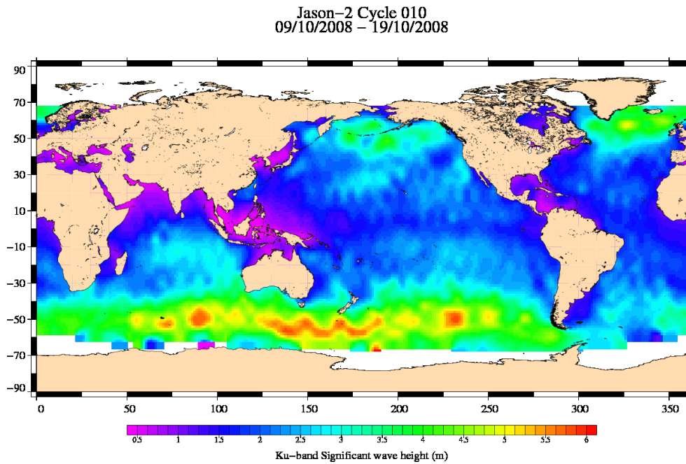
FIG. 5 – Significant wave height for cycle 010.
