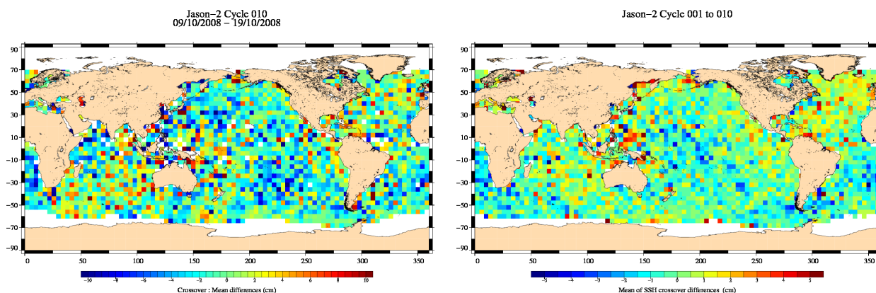
FIG. 13 – Mean SSH at crossovers for cycle 010 (left) and over the whole Jason-2 period (right).
