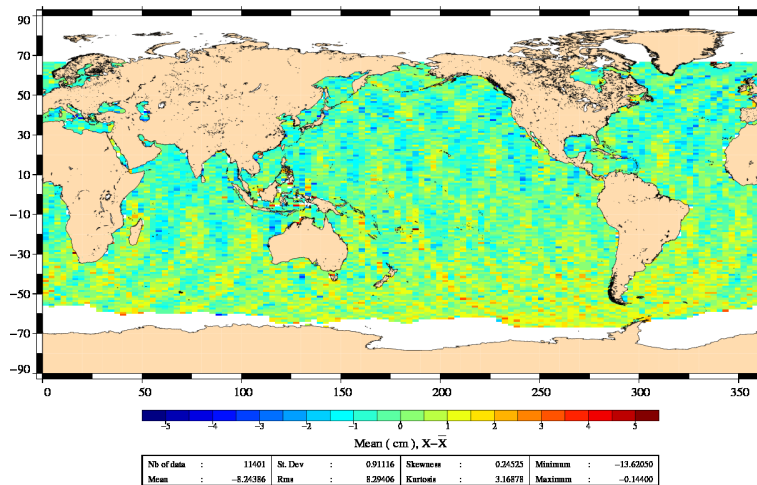
FIG. 20 – Jason-1 – Jason-2 SLA differences (without corrections) for cycle 013.
