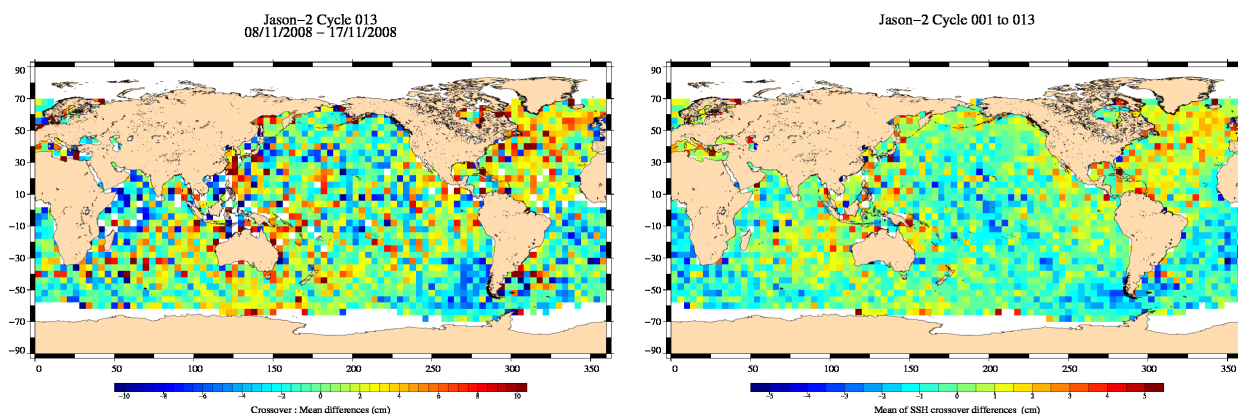
FIG. 13 – Mean SSH at crossovers for cycle 013 (left) and over the whole Jason-2 period (right).
