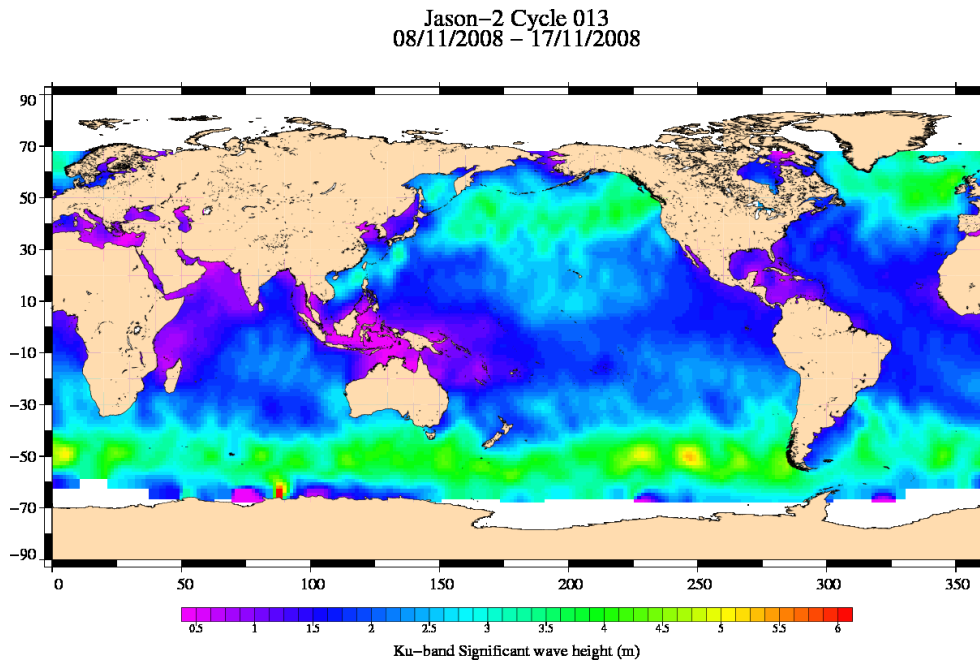
FIG. 5 – Significant wave height for cycle 013.
