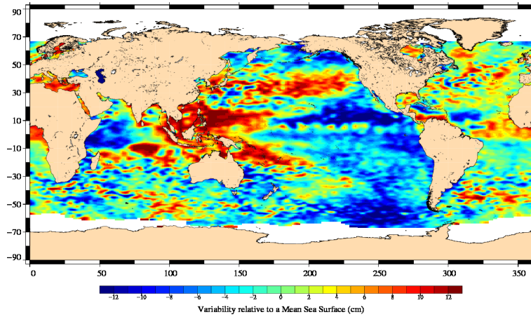
FIG. 18 – Sea level anomaly relative to MSS for cycle 013.
