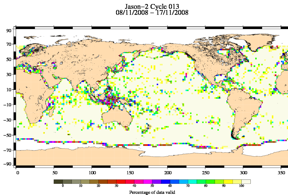
FIG. 3 – Percentage of valid measurements for cycle 013.
