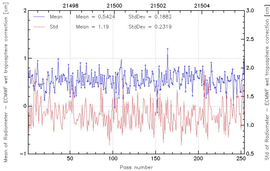
FIG. 11 – Pass monitoring of wet troposphere differences between radiometer and ECMWF model for Jason-2 cycle 013.
