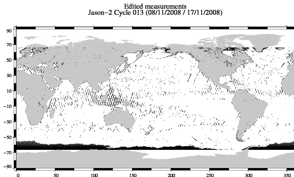
FIG. 2 – Edited measurements for cycle 013.
