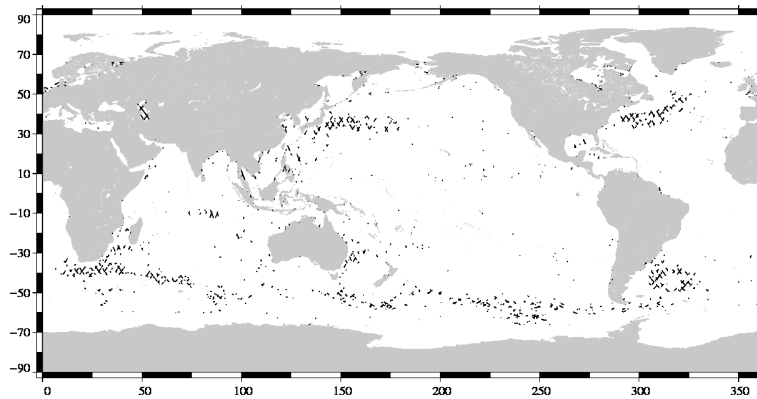
FIG. 19 – Differences higher than a 30 cm threshold for cycle 013.
