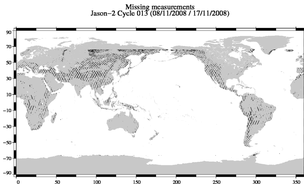
FIG. 1 – Missing measurements for cycle 013.
