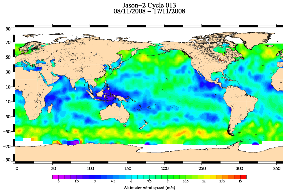
FIG. 9 – Altimeter wind speed for cycle 013.
