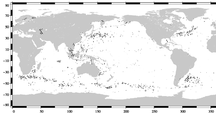
FIG. 19 – Differences higher than a 30 cm threshold for cycle 015.
