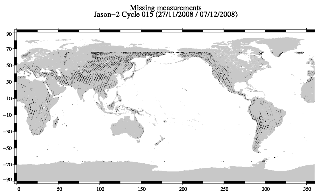
FIG. 1 – Missing measurements for cycle 015.
