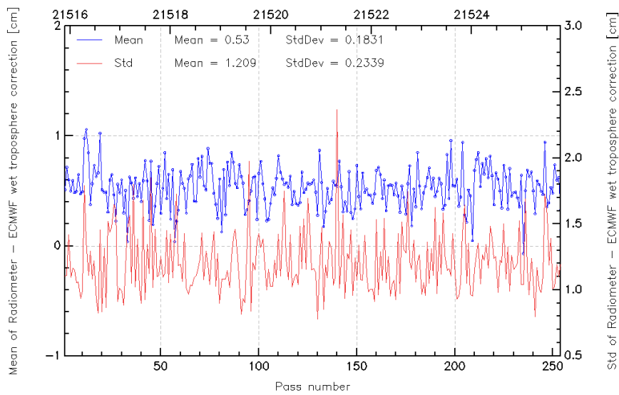
FIG. 11 – Pass monitoring of wet troposphere differences between radiometer and ECMWF model for Jason-2 cycle 015.
