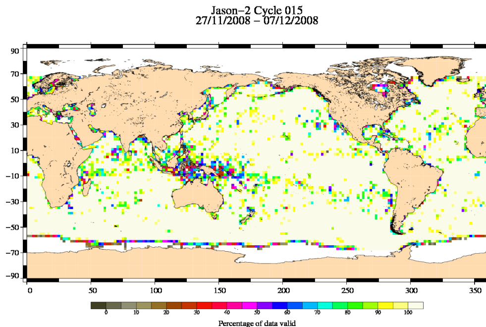
FIG. 3 – Percentage of valid measurements for cycle 015.
