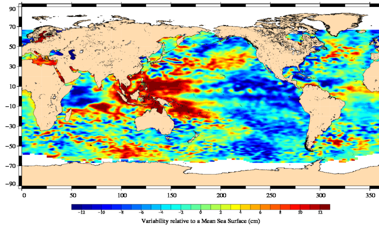
FIG. 18 – Sea level anomaly relative to MSS for cycle 015.
