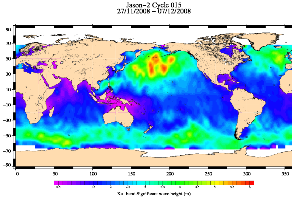
FIG. 5 – Significant wave height for cycle 015.
