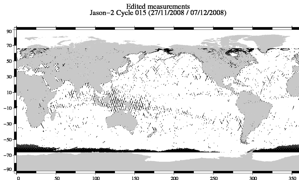
FIG. 2 – Edited measurements for cycle 015.
