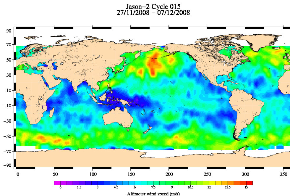
FIG. 9 – Altimeter wind speed for cycle 015.
