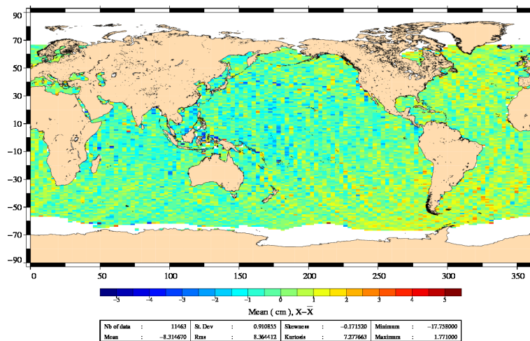
FIG. 20 – Jason-1 – Jason-2 SLA differences (without corrections) for cycle 015.
