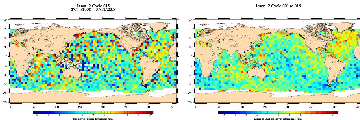
FIG. 13 – Mean SSH at crossovers for cycle 015 (left) and over the whole Jason-2 period (right).
