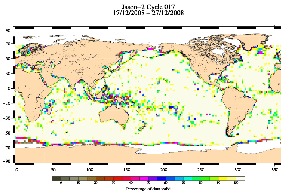
FIG. 3 – Percentage of valid measurements for cycle 017.
