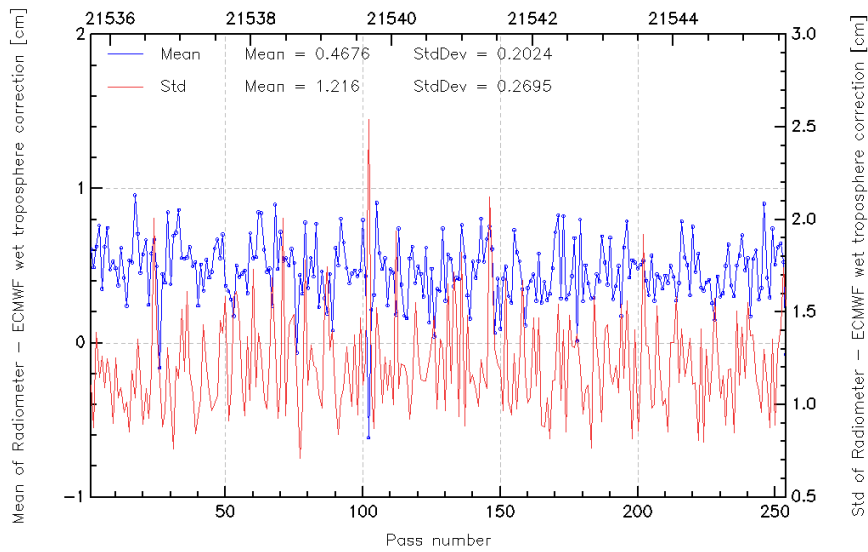
FIG. 11 – Pass monitoring of wet troposphere differences between radiometer and ECMWF model for Jason-2 cycle 017.
