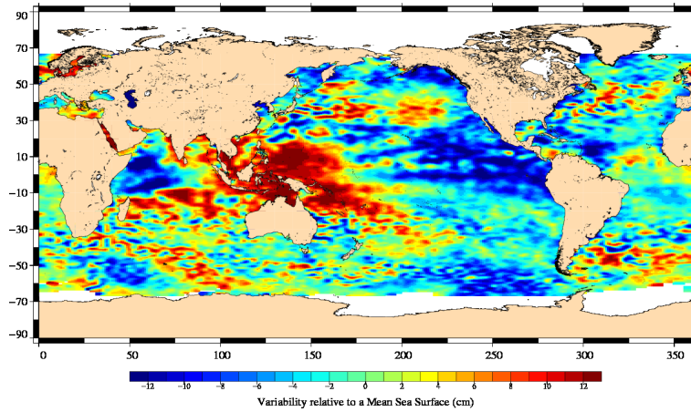
FIG. 18 – Sea level anomaly relative to MSS for cycle 017.
