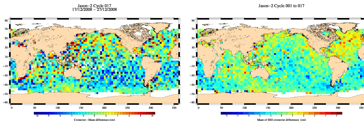
FIG. 13 – Mean SSH at crossovers for cycle 017 (left) and over the whole Jason-2 period (right).
