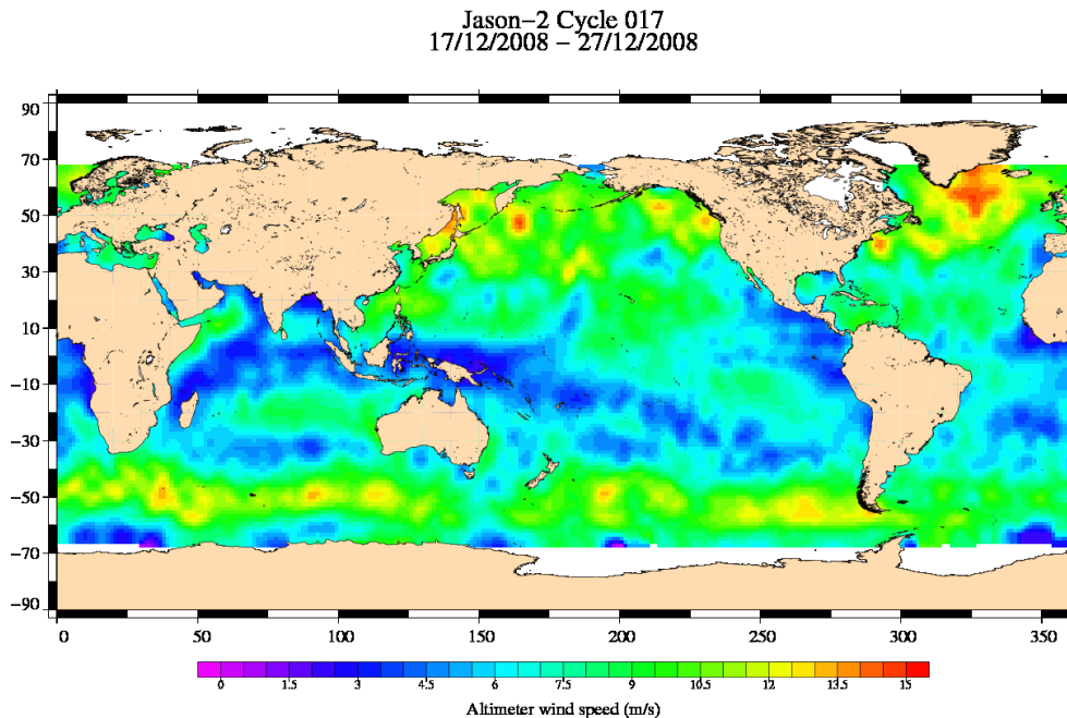
FIG. 9 – Altimeter wind speed for cycle 017.
