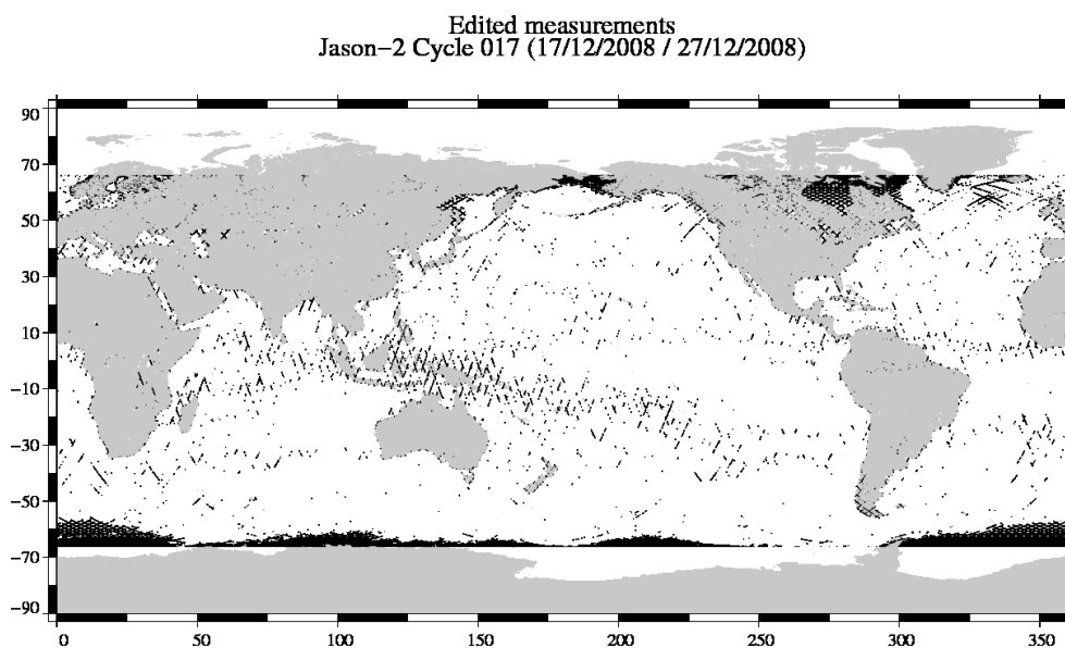
FIG. 2 – Edited measurements for cycle 017.
