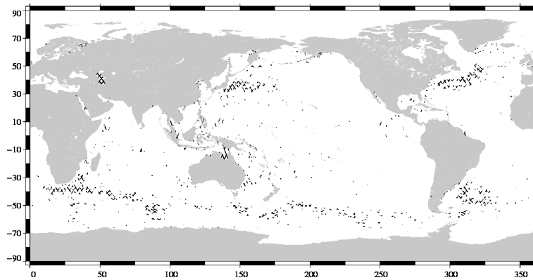
FIG. 19 – Differences higher than a 30 cm threshold for cycle 017.
