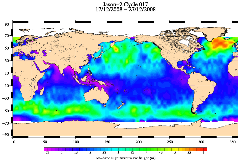
FIG. 5 – Significant wave height for cycle 017.
