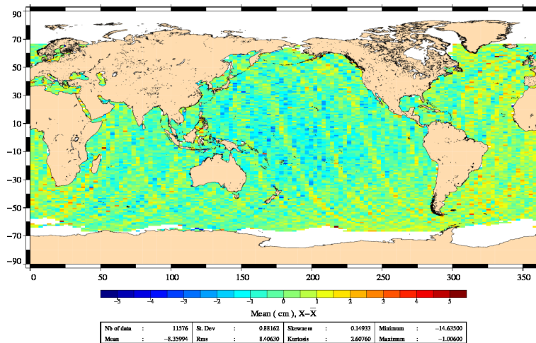
FIG. 20 – Jason-1 – Jason-2 SLA differences (without corrections) for cycle 017.
