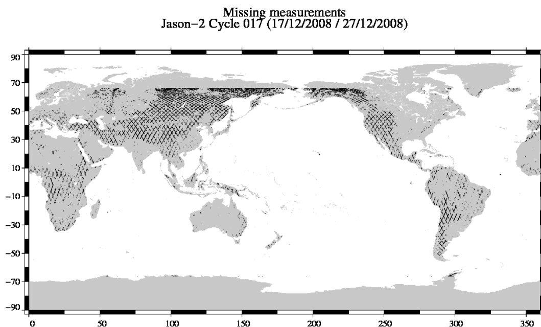
FIG. 1 – Missing measurements for cycle 017.
