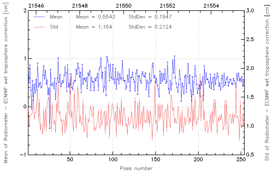
FIG. 11 – Pass monitoring of wet troposphere differences between radiometer and ECMWF model for Jason-2 cycle 018.
