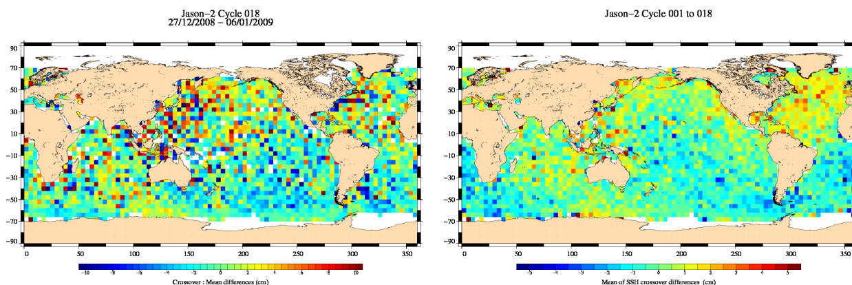
FIG. 13 – Mean SSH at crossovers for cycle 018 (left) and over the whole Jason-2 period (right).
