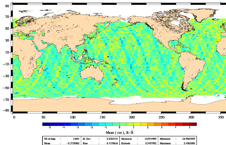
FIG. 20 – Jason-1 – Jason-2 SLA differences (without corrections) for cycle 018.
