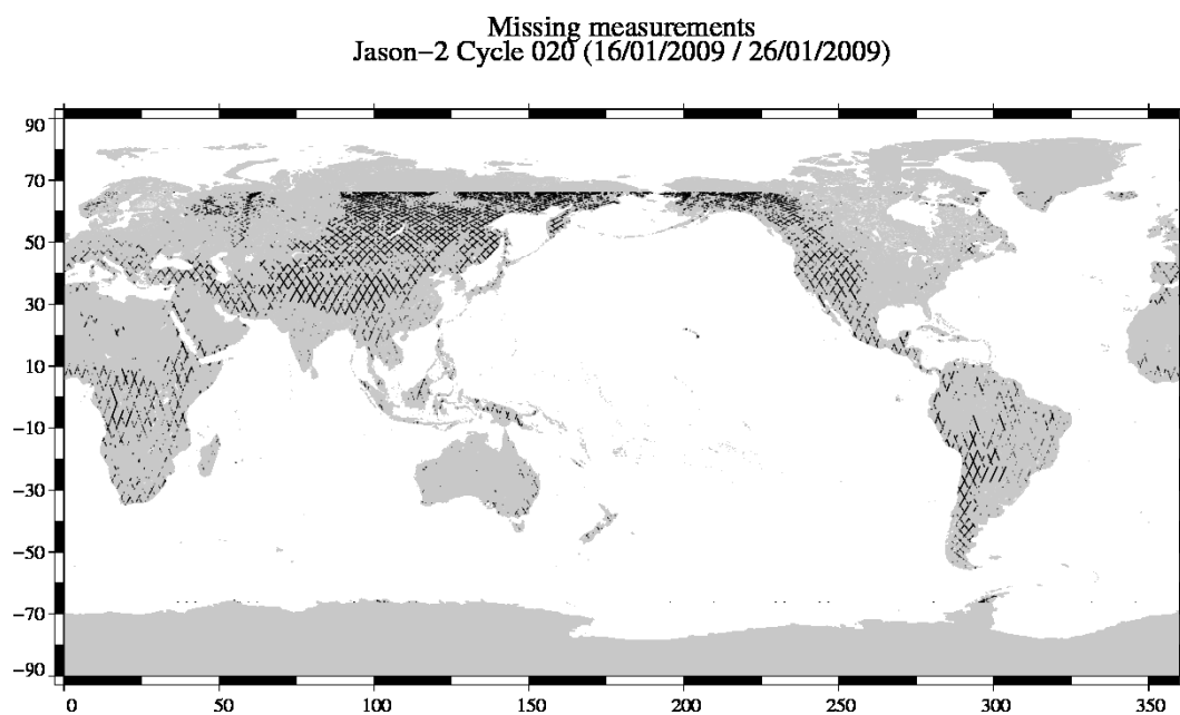
FIG. 1 – Missing measurements for cycle 020.
