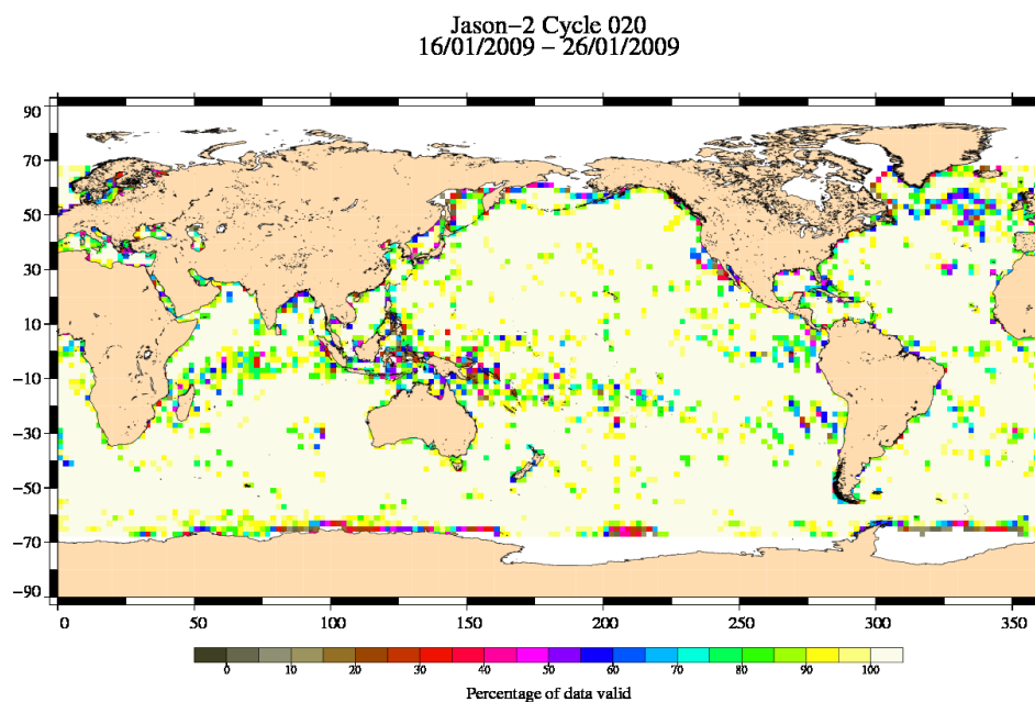
FIG. 3 – Percentage of valid measurements for cycle 020.
