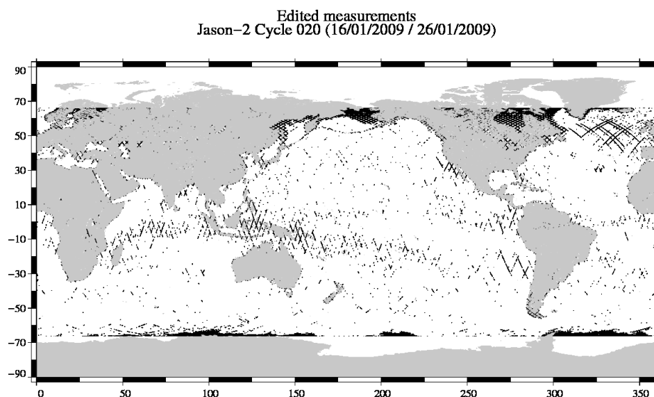
FIG. 2 – Edited measurements for cycle 020.
