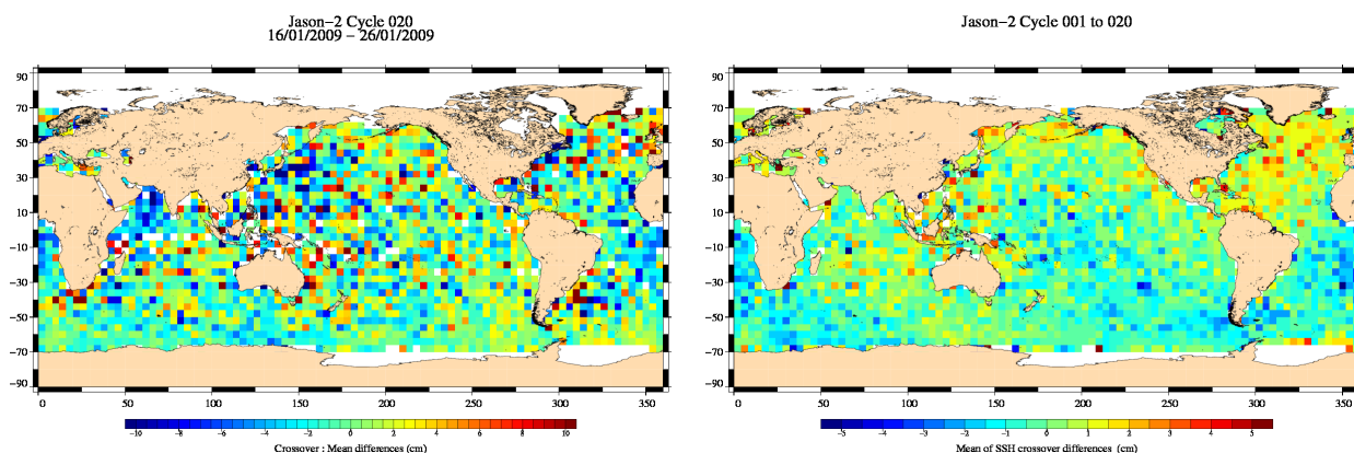
FIG. 13 – Mean SSH at crossovers for cycle 020 (left) and over the whole Jason-2 period (right).
