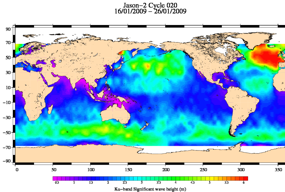
FIG. 5 – Significant wave height for cycle 020.
