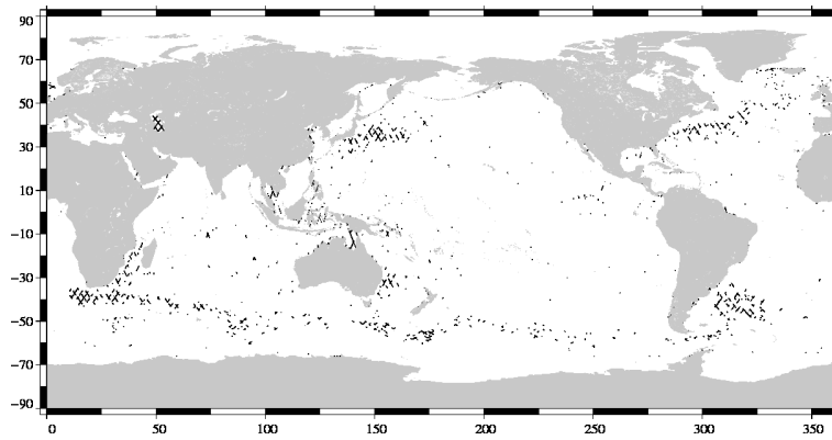
FIG. 19 – Differences higher than a 30 cm threshold for cycle 020.
