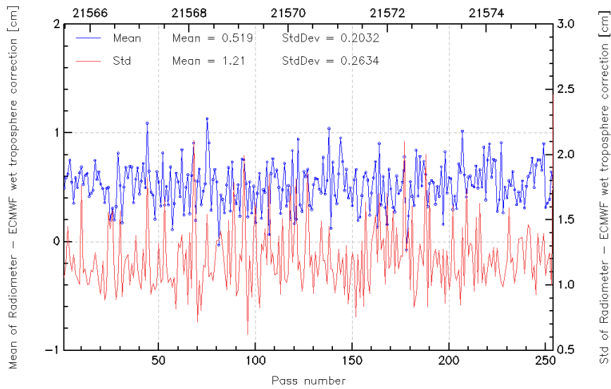
FIG. 11 – Pass monitoring of wet troposphere differences between radiometer and ECMWF model for Jason-2 cycle 020.
