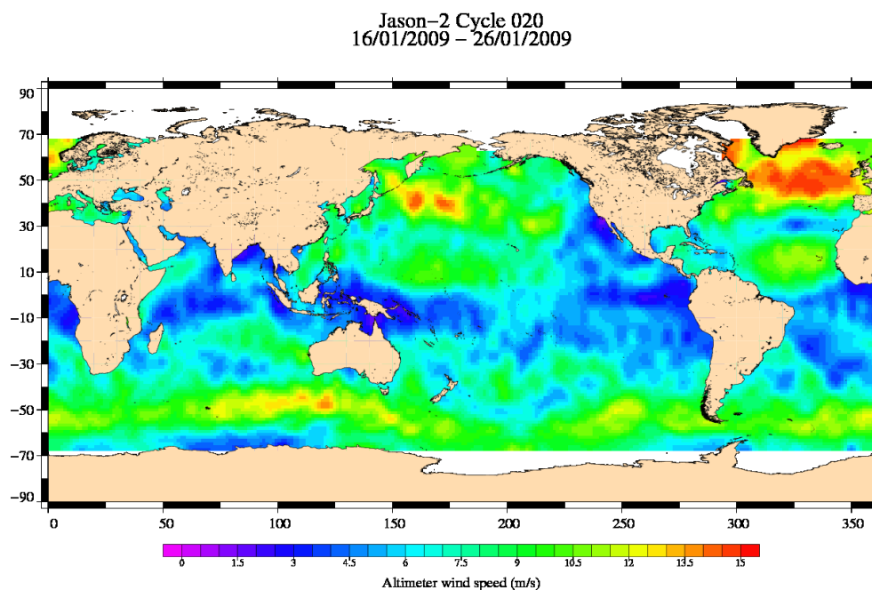
FIG. 9 – Altimeter wind speed for cycle 020.
