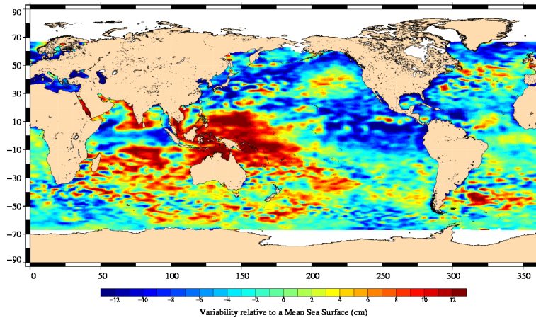
FIG. 18 – Sea level anomaly relative to MSS for cycle 020.
