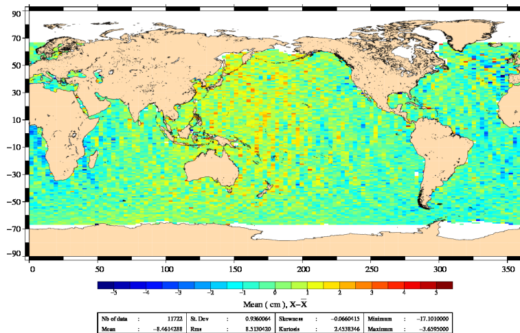
FIG. 20 – Jason-1 – Jason-2 SLA differences (without corrections) for cycle 020.
