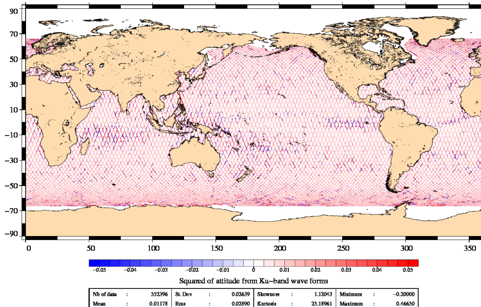
FIG. 4 – Apparent squared mispointing from waveforms for cycle 022.
