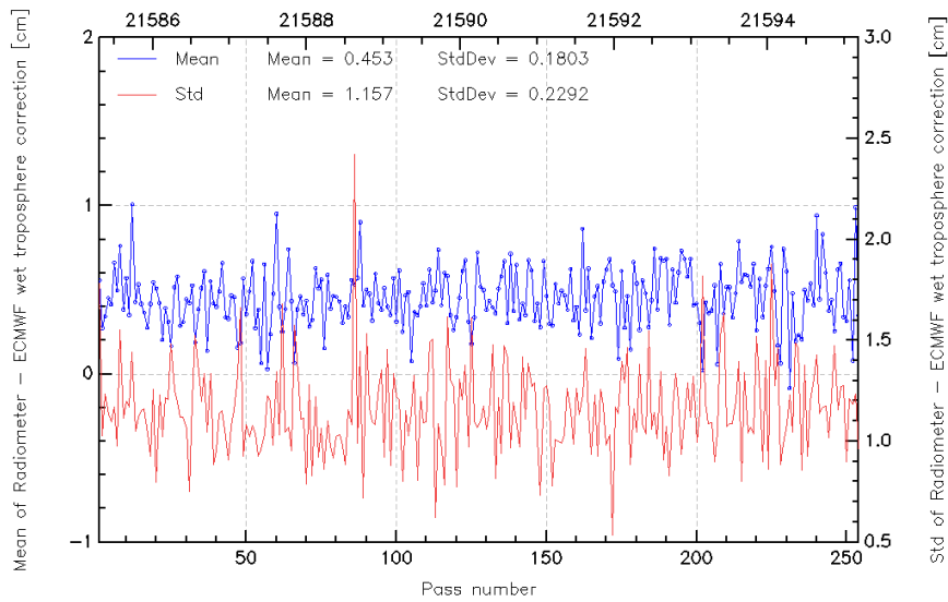
FIG. 12 – Pass monitoring of wet troposphere differences between radiometer and ECMWF model for Jason-2 cycle 022.
