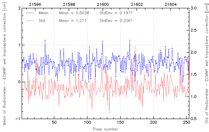
FIG. 12 – Pass monitoring of wet troposphere differences between radiometer and ECMWF model for Jason-2 cycle 023.
