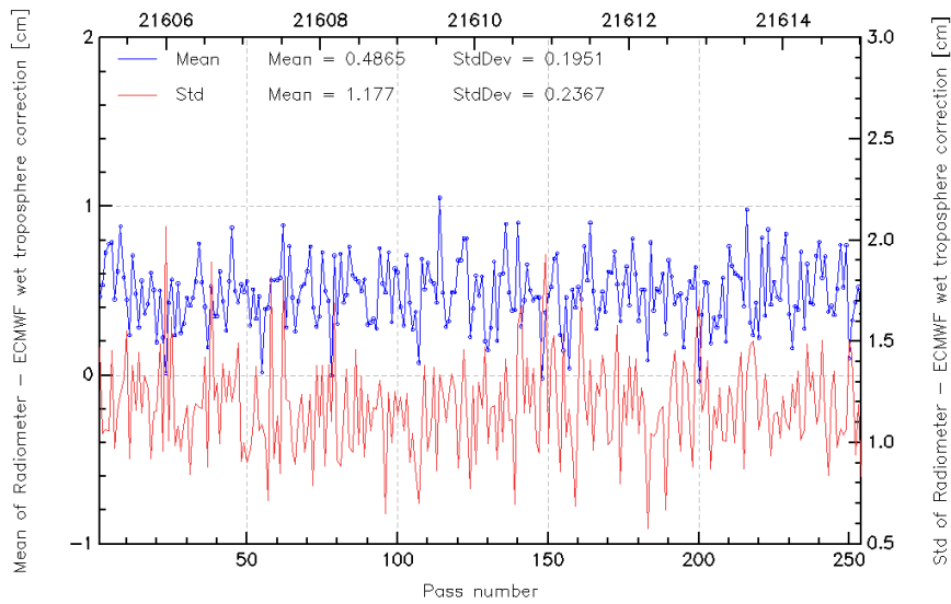
FIG. 11 – Pass monitoring of wet troposphere differences between radiometer and ECMWF model for Jason-2 cycle 024.
