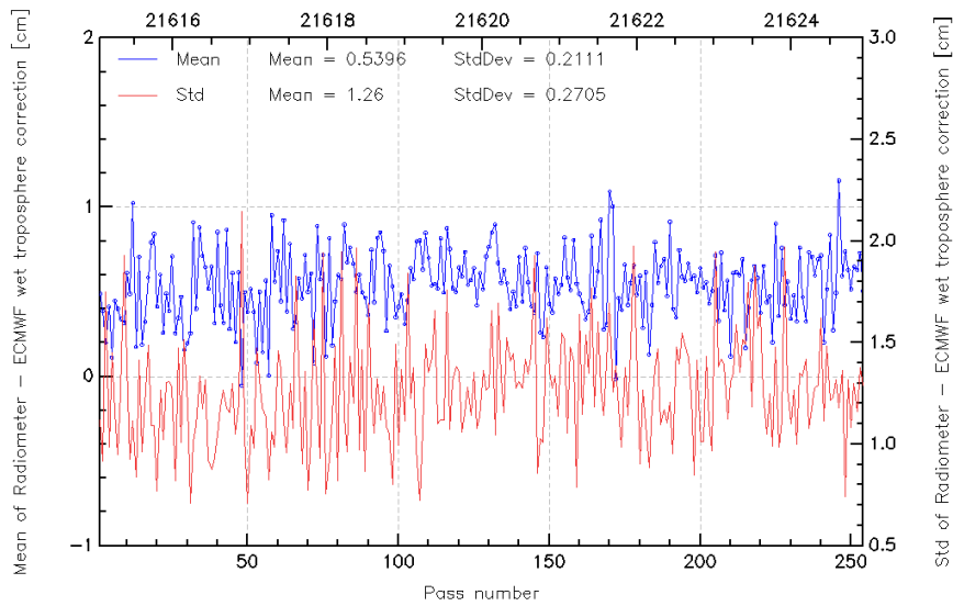
FIG. 11 – Pass monitoring of wet troposphere differences between radiometer and ECMWF model for Jason-2 cycle 025.
