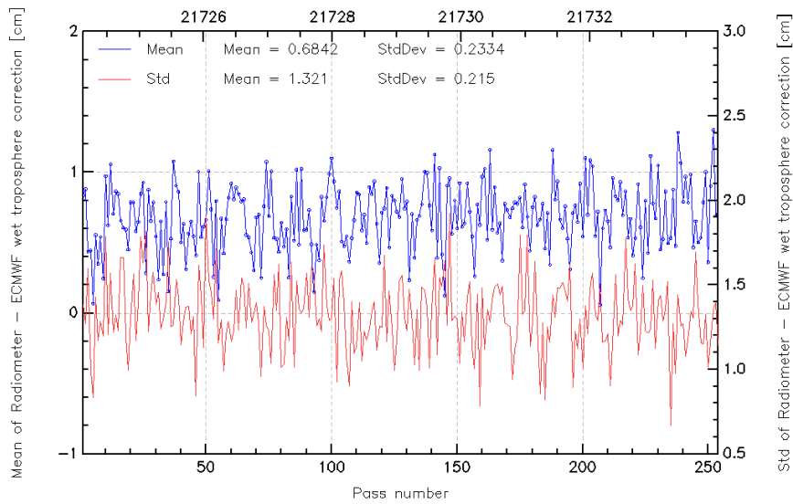
FIG. 11 – Pass monitoring of wet troposphere differences between radiometer and ECMWF model for Jason-2 cycle 036.
