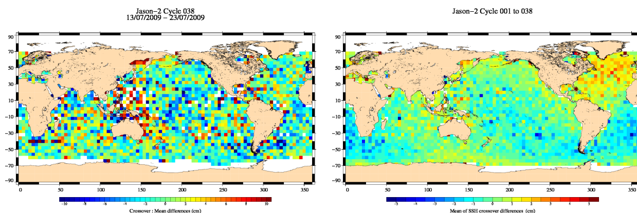
FIG. 13 – Mean SSH at crossovers for cycle 038 (left) and over the whole Jason-2 period (right).
