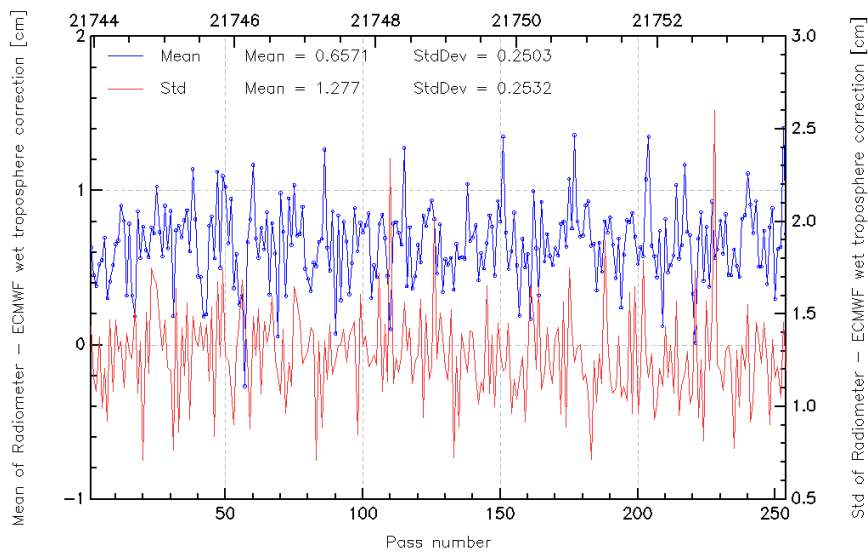
FIG. 11 – Pass monitoring of wet troposphere differences between radiometer and ECMWF model for Jason-2 cycle 038.
