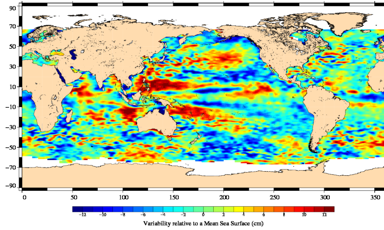
FIG. 18 – Sea level anomaly relative to MSS for cycle 038.
