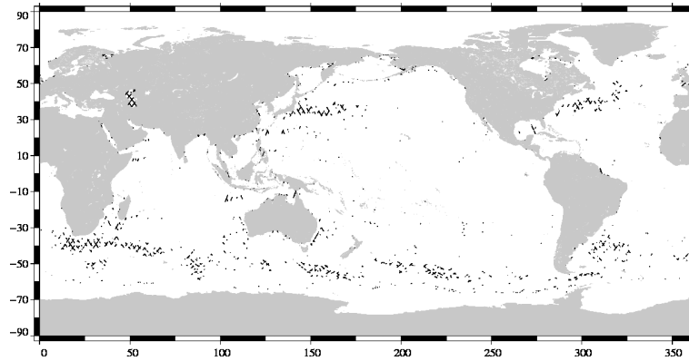
FIG. 19 – Differences higher than a 30 cm threshold for cycle 038.
