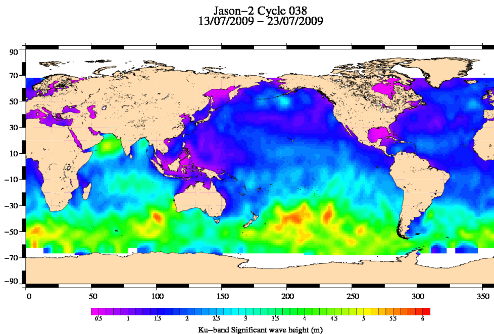
FIG. 5 – Significant wave height for cycle 038.
