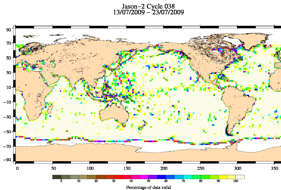
FIG. 3 – Percentage of valid measurements for cycle 038.
