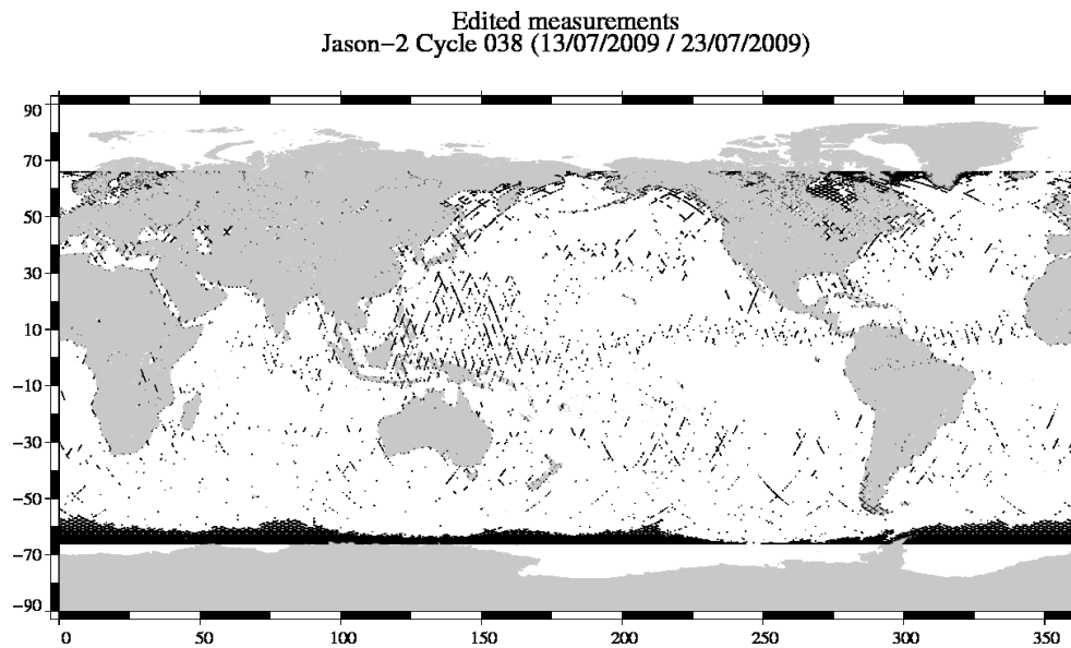
FIG. 2 – Edited measurements for cycle 038.
