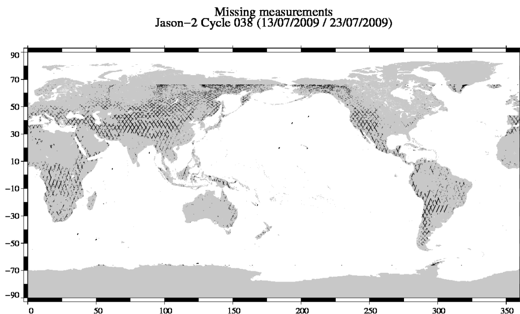
FIG. 1 – Missing measurements for cycle 038.
