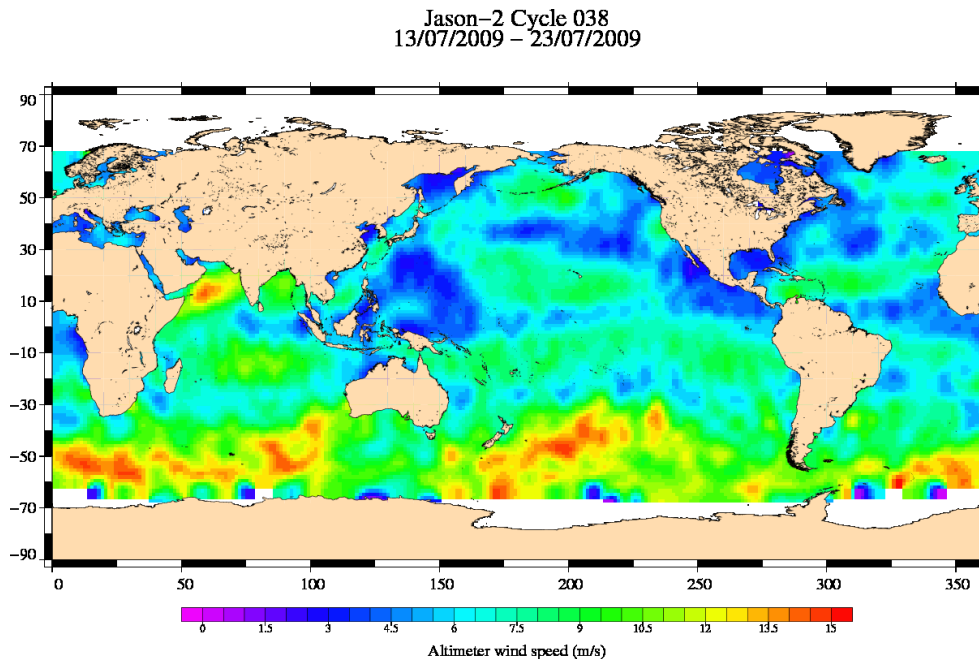
FIG. 9 – Altimeter wind speed for cycle 038.
