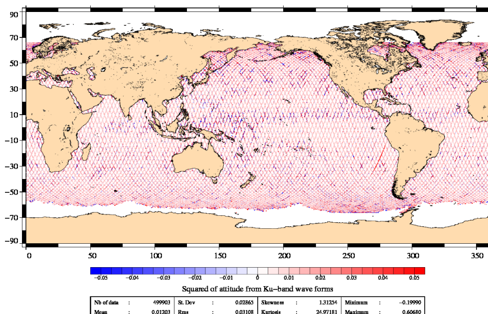
FIG. 4 – Apparent squared mispointing from waveforms for cycle 040.
