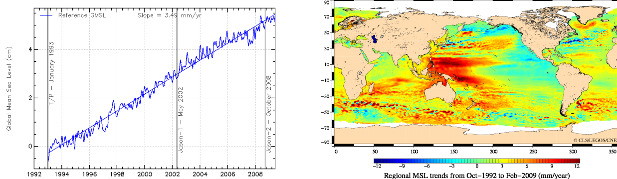
FIG. 23 – Global (left) and regional (right) MSL trends from 1993 onwards.
