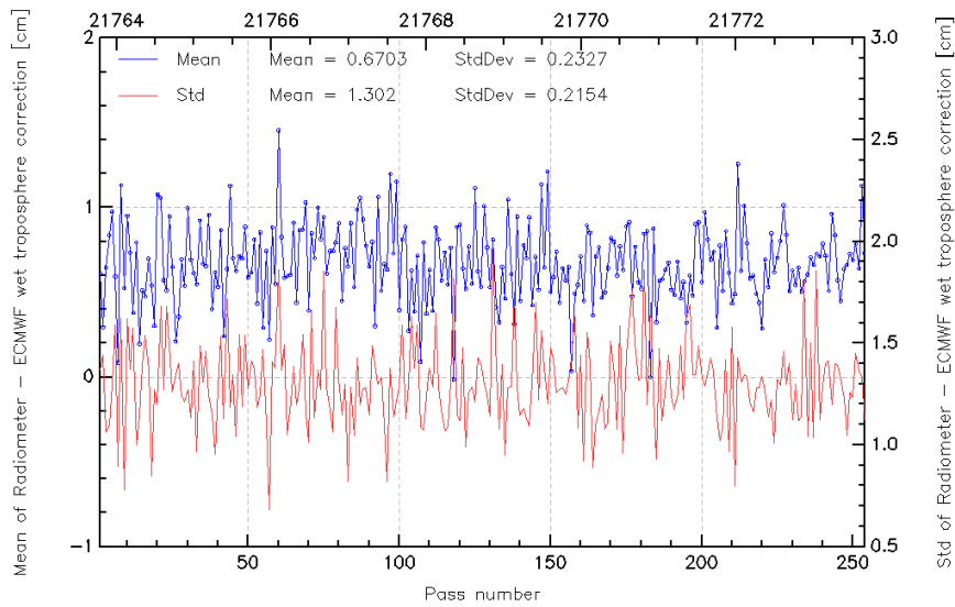
FIG. 12 – Pass monitoring of wet troposphere differences between radiometer and ECMWF model for Jason-2 cycle 040.
