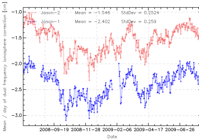
FIG. 9 – Daily monitoring of dual-frequency ionosphere correction for Jason-2 and Jason-1.
