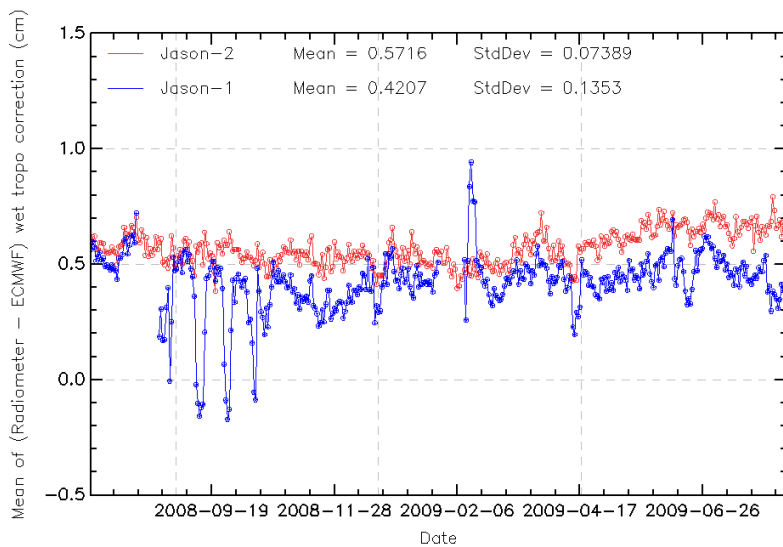
FIG. 13 – Daily monitoring of wet troposphere differences between radiometer and ECMWF model
