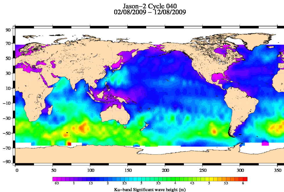
FIG. 6 – Significant wave height for cycle 040.
