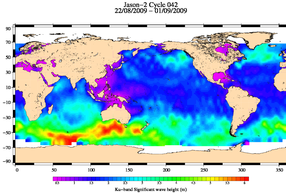
FIG. 5 – Significant wave height for cycle 042.
