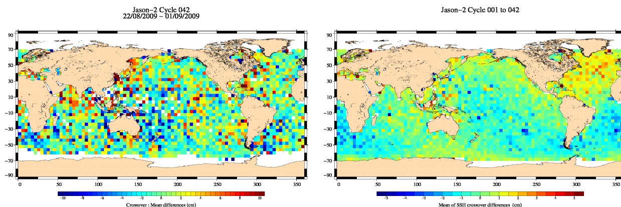
FIG. 13 – Mean SSH at crossovers for cycle 042 (left) and over the whole Jason-2 period (right).
