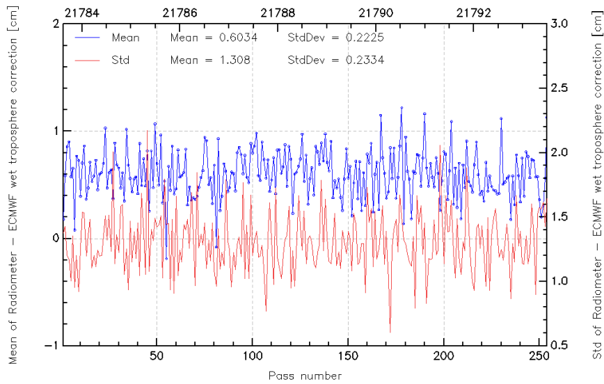
FIG. 11 – Pass monitoring of wet troposphere differences between radiometer and ECMWF model for Jason-2 cycle 042.
