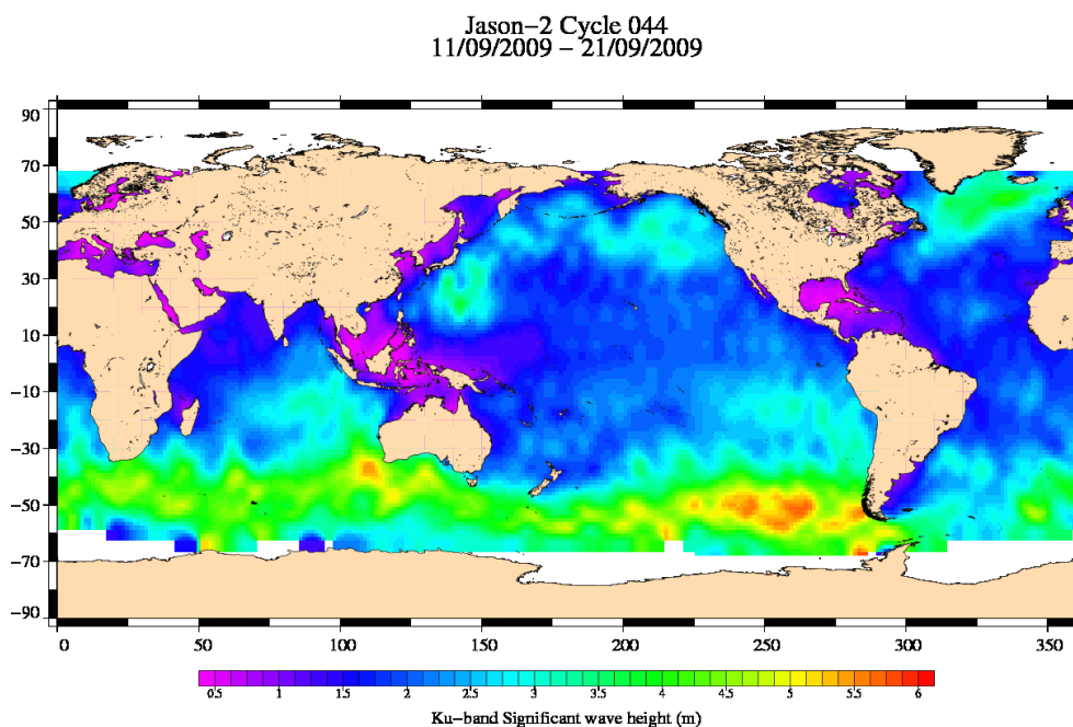
FIG. 5 – Significant wave height for cycle 044.
