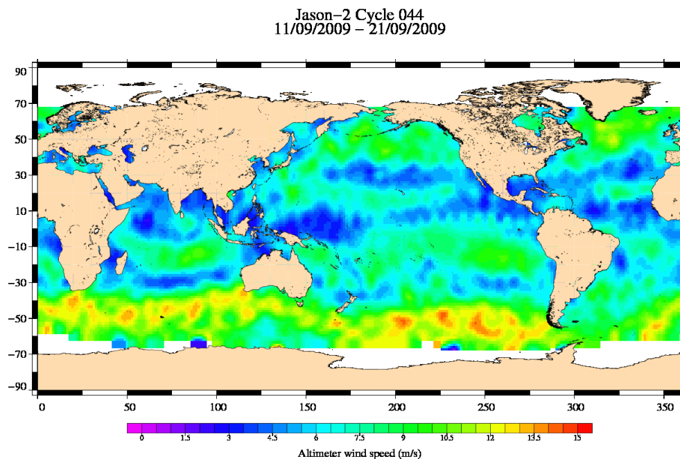
FIG. 9 – Altimeter wind speed for cycle 044.
