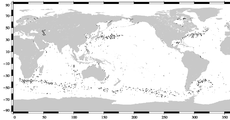
FIG. 19 – Differences higher than a 30 cm threshold for cycle 044.
