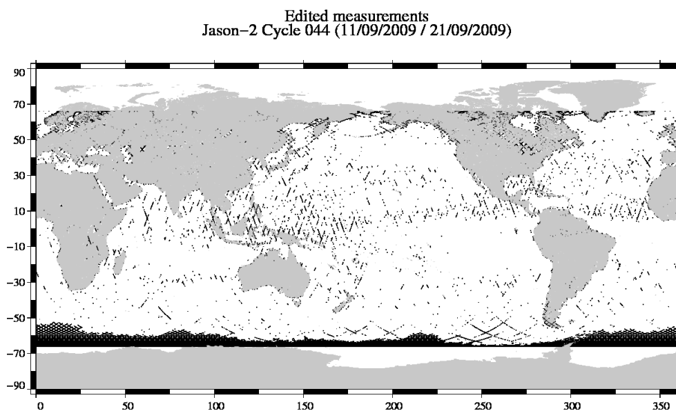
FIG. 2 – Edited measurements for cycle 044.
