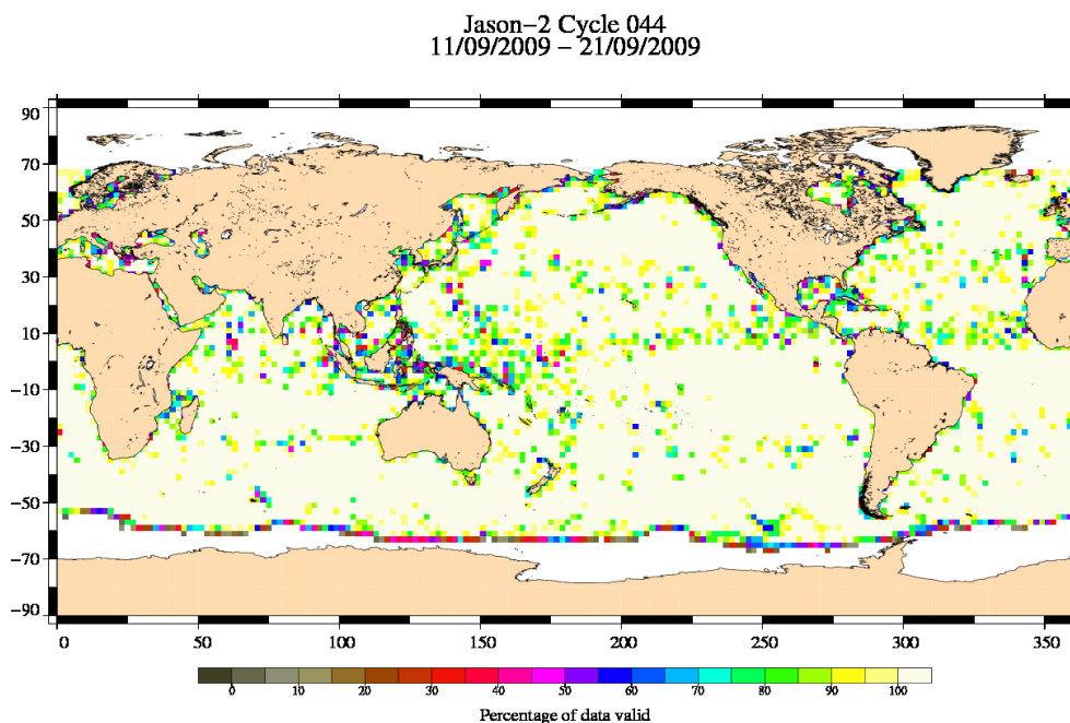
FIG. 3 – Percentage of valid measurements for cycle 044.
