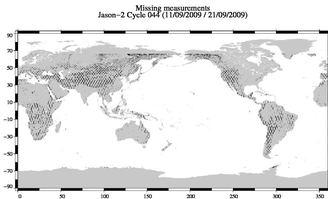
FIG. 1 – Missing measurements for cycle 044.
