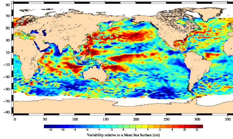
FIG. 18 – Sea level anomaly relative to MSS for cycle 044.
