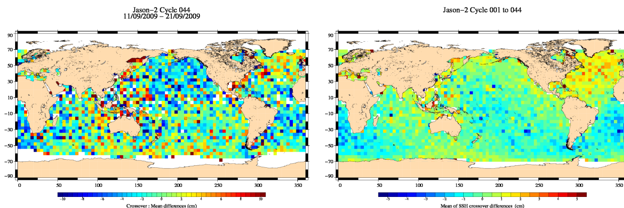
FIG. 13 – Mean SSH at crossovers for cycle 044 (left) and over the whole Jason-2 period (right).
