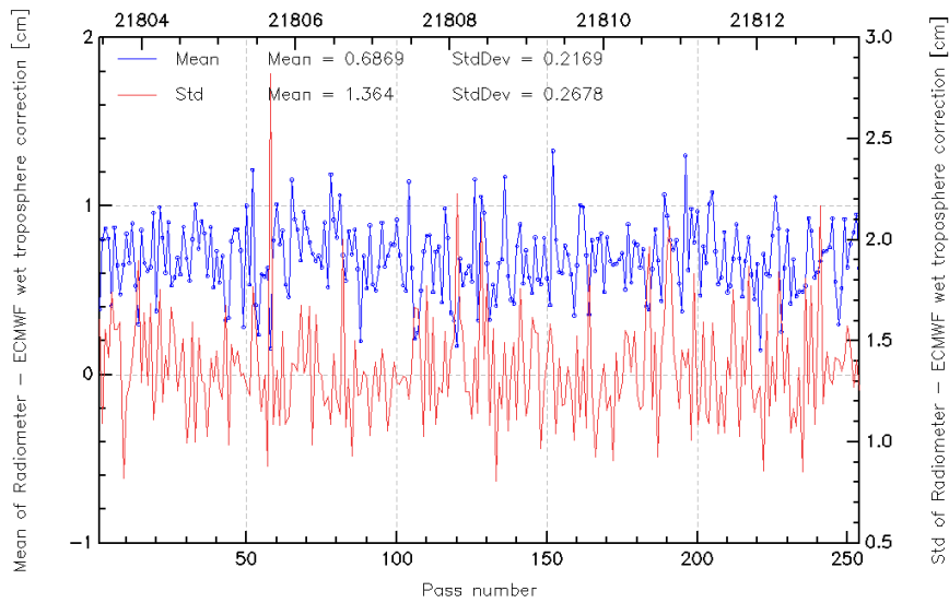
FIG. 11 – Pass monitoring of wet troposphere differences between radiometer and ECMWF model for Jason-2 cycle 044.
