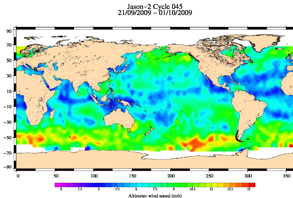
FIG. 9 – Altimeter wind speed for cycle 045.
