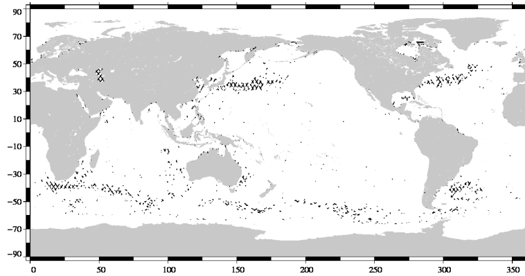
FIG. 19 – Differences higher than a 30 cm threshold for cycle 045.
