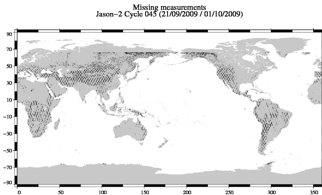
FIG. 1 – Missing measurements for cycle 045.
