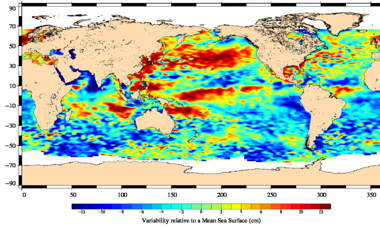
FIG. 18 – Sea level anomaly relative to MSS for cycle 045.
