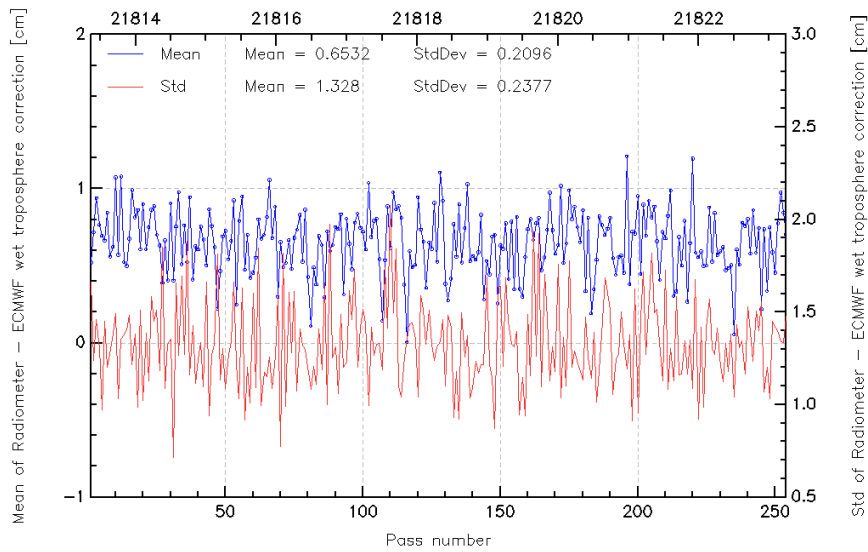
FIG. 11 – Pass monitoring of wet troposphere differences between radiometer and ECMWF model for Jason-2 cycle 045.
