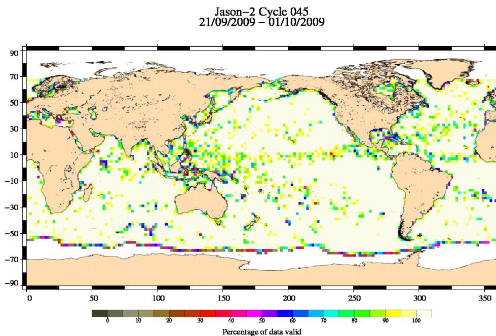
FIG. 3 – Percentage of valid measurements for cycle 045.
