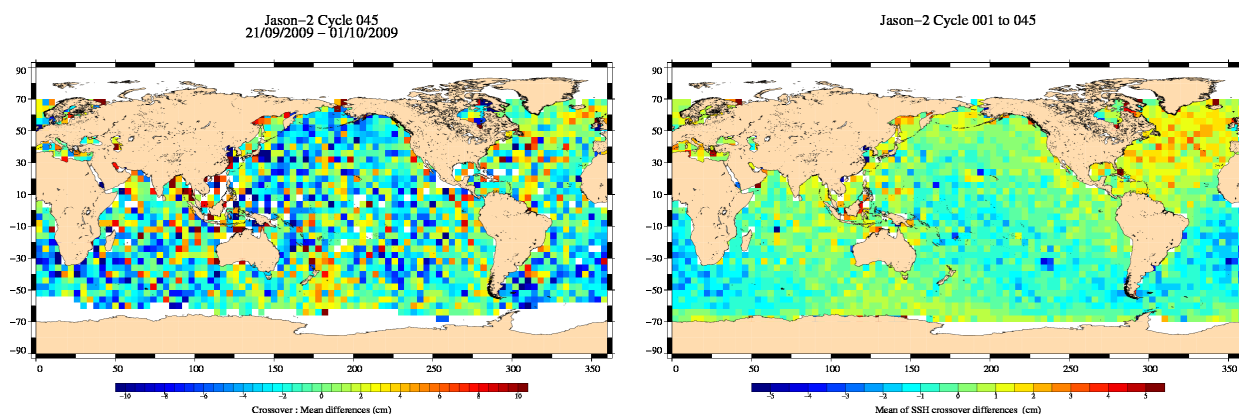
FIG. 13 – Mean SSH at crossovers for cycle 045 (left) and over the whole Jason-2 period (right).
