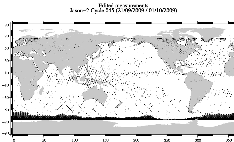
FIG. 2 – Edited measurements for cycle 045.
