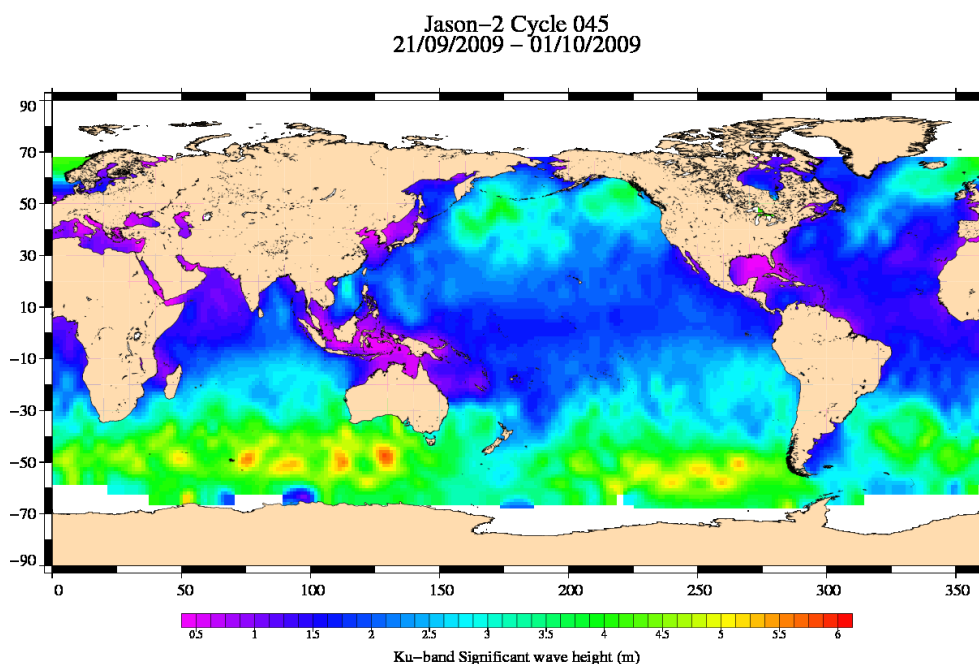
FIG. 5 – Significant wave height for cycle 045.
