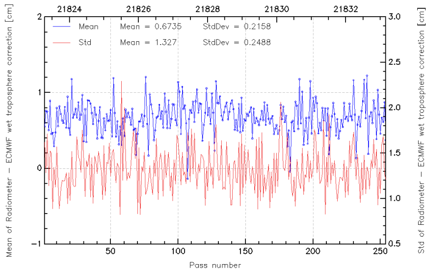
FIG. 12 – Pass monitoring of wet troposphere differences between radiometer and ECMWF model for Jason-2 cycle 046.
