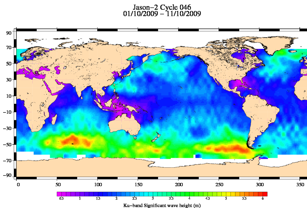
FIG. 6 – Significant wave height for cycle 046.
