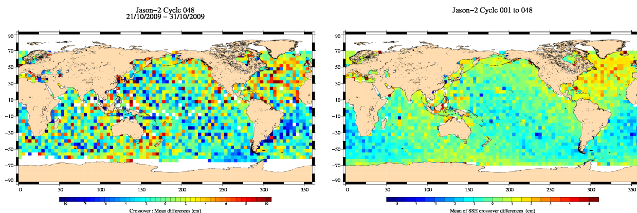
FIG. 13 – Mean SSH at crossovers for cycle 048 (left) and over the whole Jason-2 period (right).
