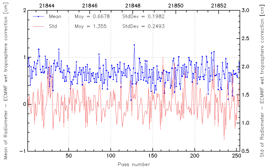
FIG. 11 – Pass monitoring of wet troposphere differences between radiometer and ECMWF model for Jason-2 cycle 048.
