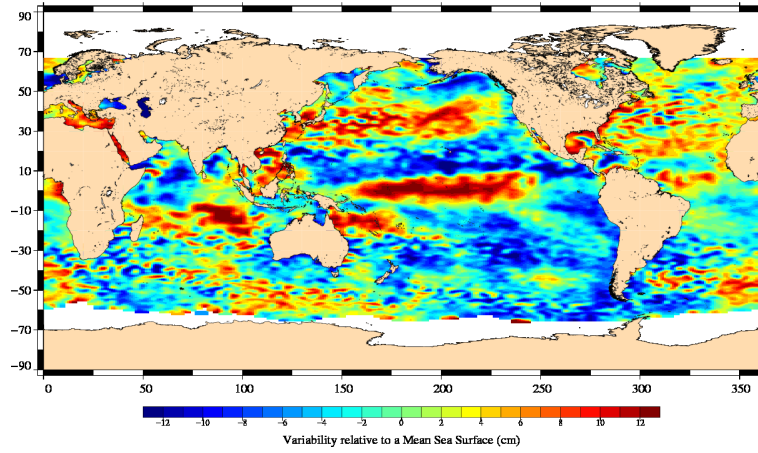
Jason-2 Cycle 048 21/10/2009 – 31/10/2009
