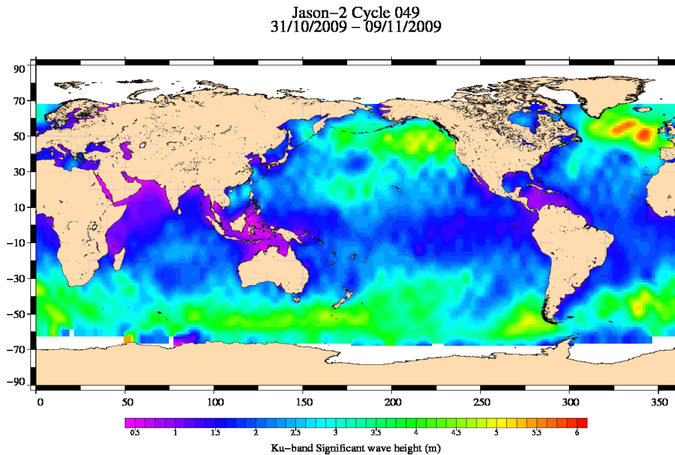
FIG. 5 – Significant wave height for cycle 049.
