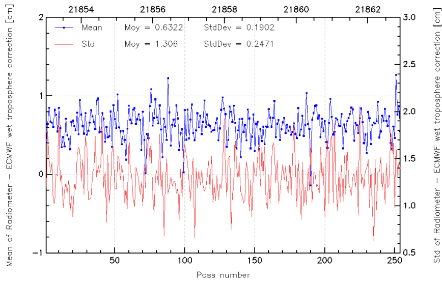
FIG. 11 – Pass monitoring of wet troposphere differences between radiometer and ECMWF model for Jason-2 cycle 049.
