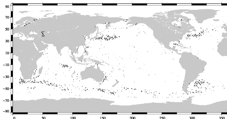
FIG. 19 – Differences higher than a 30 cm threshold for cycle 049.
