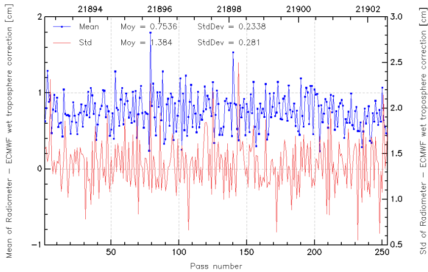
FIG. 11 – Pass monitoring of wet troposphere differences between radiometer and ECMWF model for Jason-2 cycle 053.
