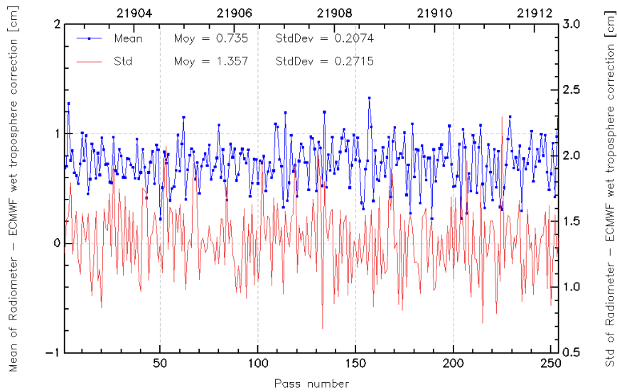
FIG. 11 – Pass monitoring of wet troposphere differences between radiometer and ECMWF model for Jason-2 cycle 054.
