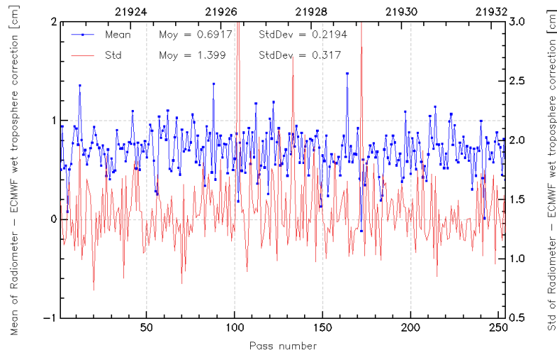
FIG. 11 – Pass monitoring of wet troposphere differences between radiometer and ECMWF model for Jason-2 cycle 056.
