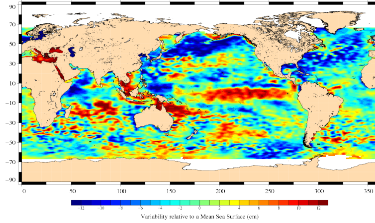
FIG. 18 – Sea level anomaly relative to MSS for cycle 056.
