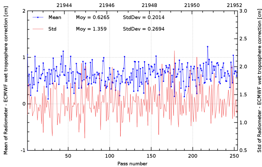
FIG. 11 – Pass monitoring of wet troposphere differences between radiometer and ECMWF model for Jason-2 cycle 058.
