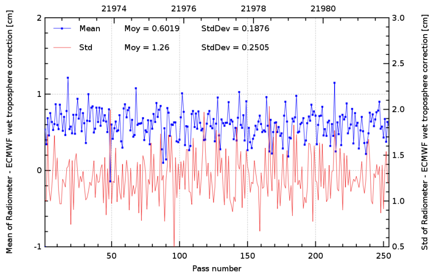
FIG. 11 – Pass monitoring of wet troposphere differences between radiometer and ECMWF model for Jason-2 cycle 061.
