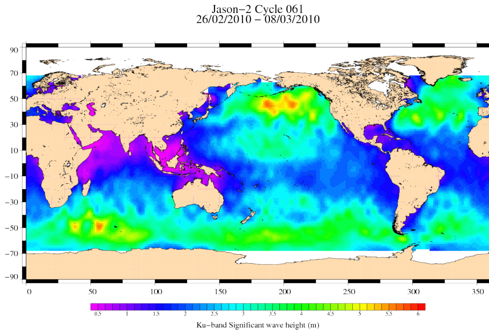
FIG. 5 – Significant wave height for cycle 061.
