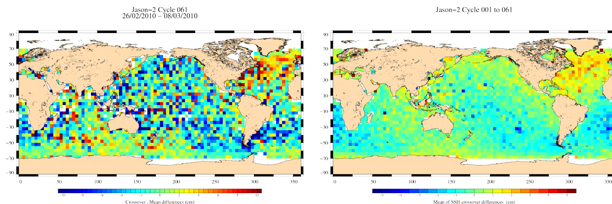
FIG. 13 – Mean SSH at crossovers for cycle 061 (left) and over the whole Jason-2 period (right).
