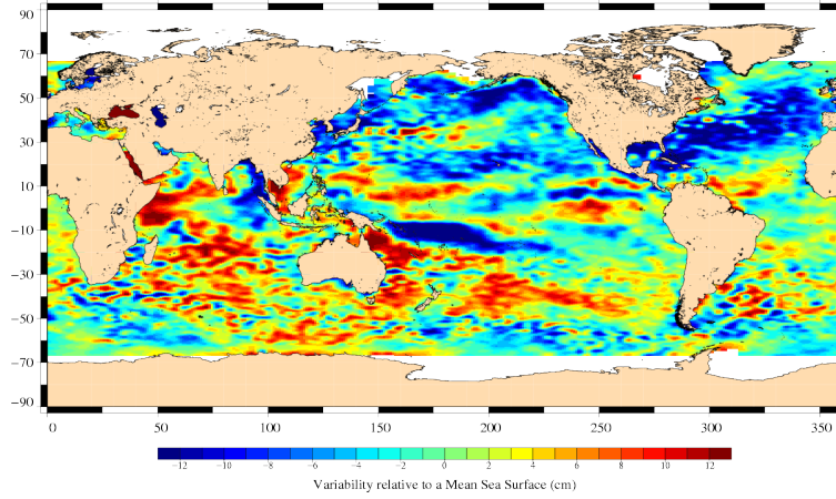
FIG. 18 – Sea level anomaly relative to MSS for cycle 062.
