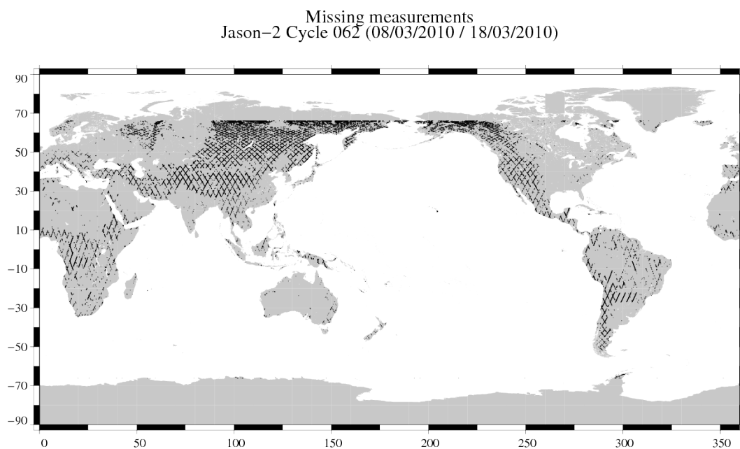
FIG. 1 – Missing measurements for cycle 062.
