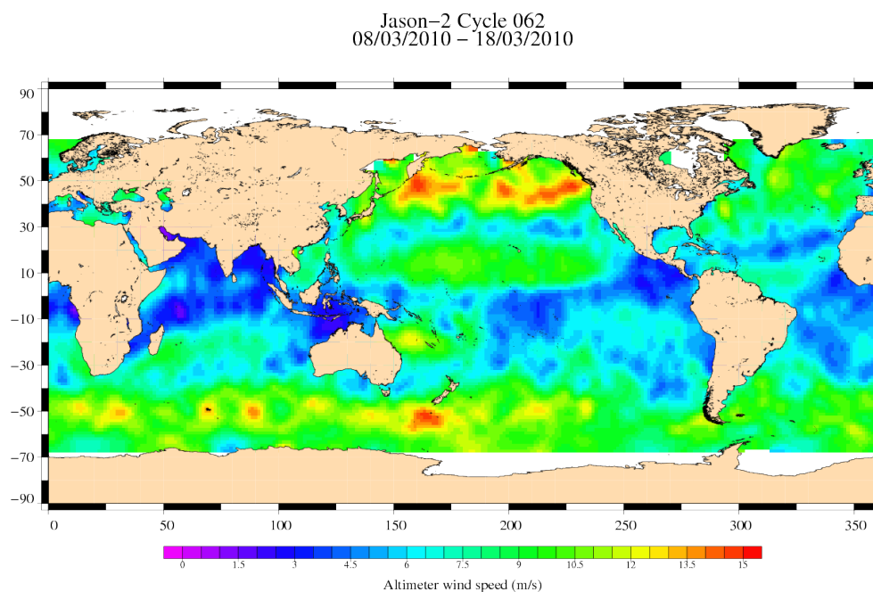
FIG. 9 – Altimeter wind speed for cycle 062.
