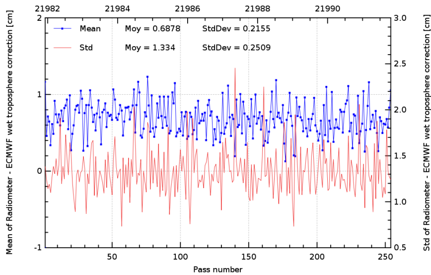
FIG. 11 – Pass monitoring of wet troposphere differences between radiometer and ECMWF model for Jason-2 cycle 062.
