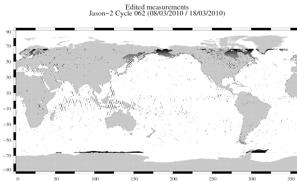
FIG. 2 – Edited measurements for cycle 062.
