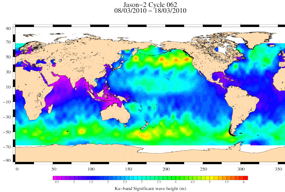
FIG. 5 – Significant wave height for cycle 062.
