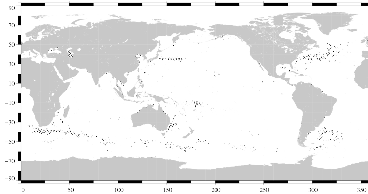
FIG. 19 – Differences higher than a 30 cm threshold for cycle 062.
