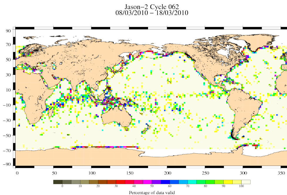
FIG. 3 – Percentage of valid measurements for cycle 062.
