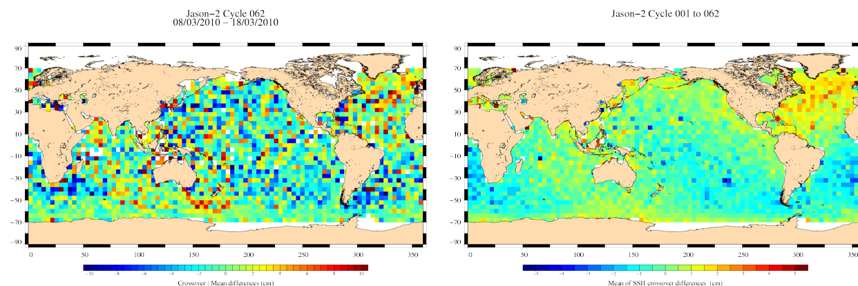
FIG. 13 – Mean SSH at crossovers for cycle 062 (left) and over the whole Jason-2 period (right).
