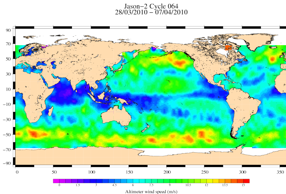
FIG. 9 – Altimeter wind speed for cycle 064.
