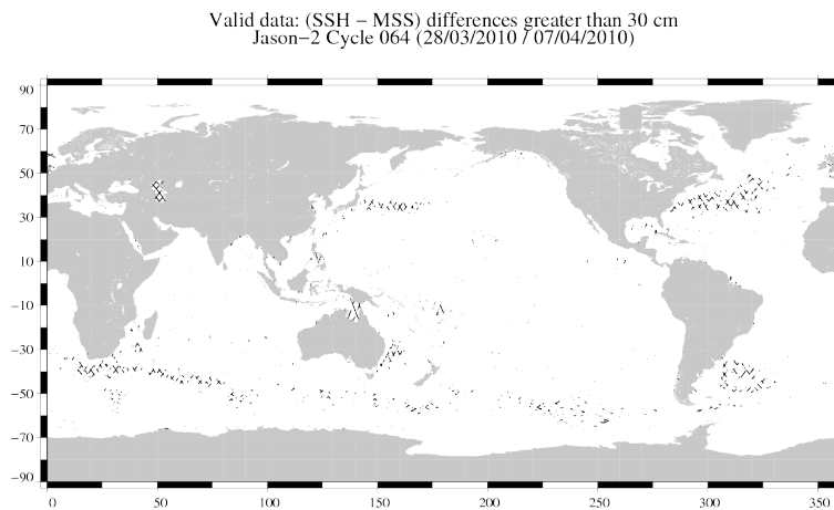
FIG. 19 – Differences higher than a 30 cm threshold for cycle 064.
