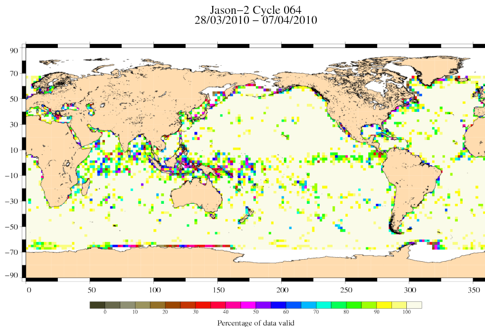
FIG. 3 – Percentage of valid measurements for cycle 064.
