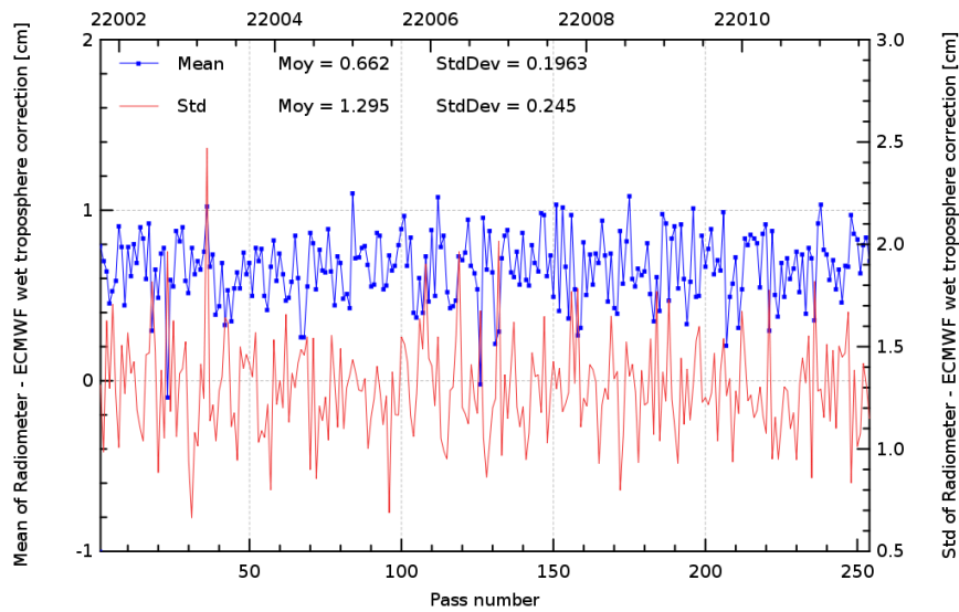
FIG. 11 – Pass monitoring of wet troposphere differences between radiometer and ECMWF model for Jason-2 cycle 064.
