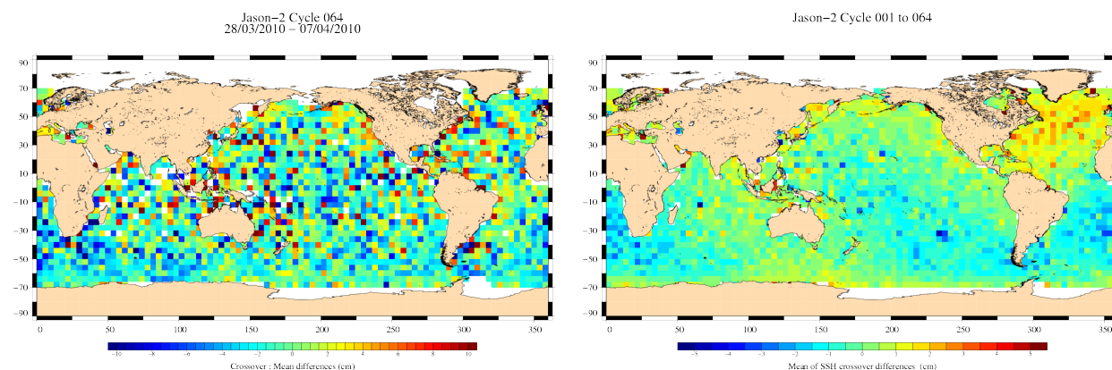
FIG. 13 – Mean SSH at crossovers for cycle 064 (left) and over the whole Jason-2 period (right).
