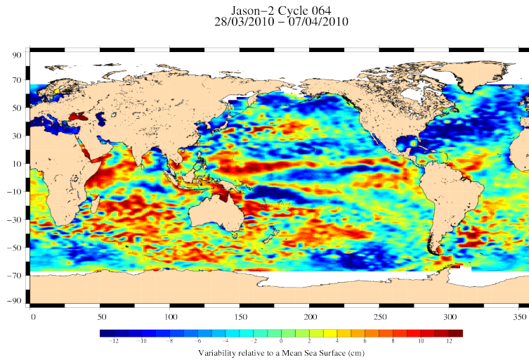
FIG. 18 – Sea level anomaly relative to MSS for cycle 064.
