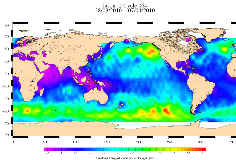
FIG. 5 – Significant wave height for cycle 064.
