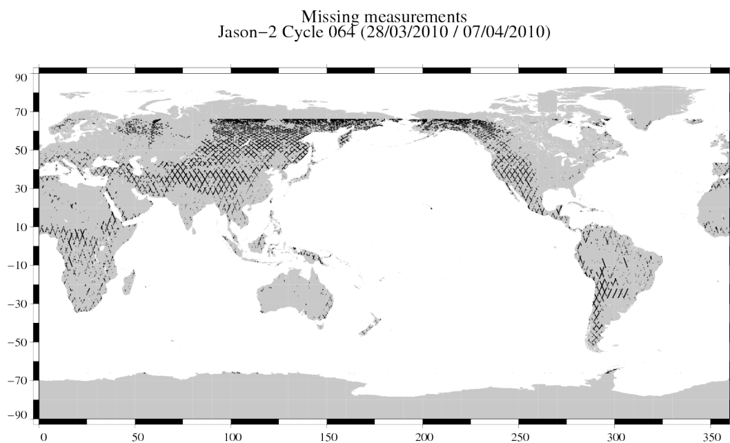
FIG. 1 – Missing measurements for cycle 064.
