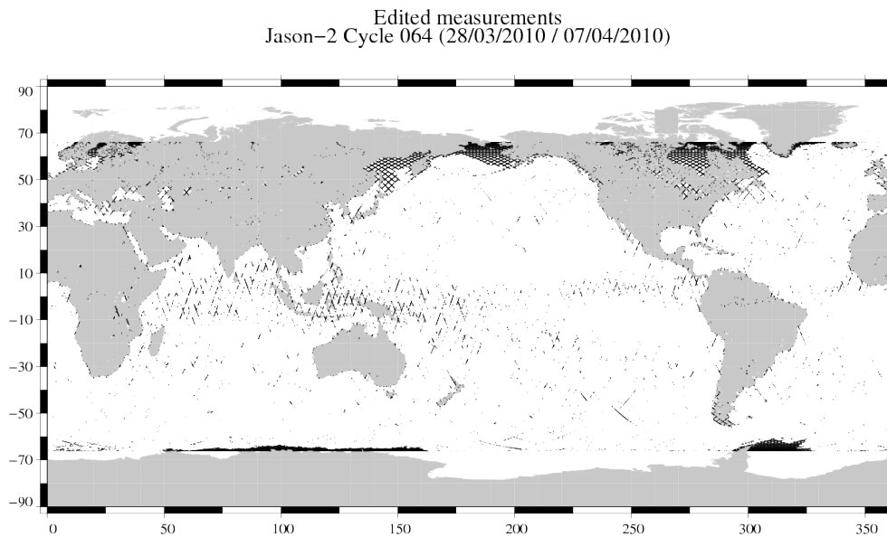
FIG. 2 – Edited measurements for cycle 064.
