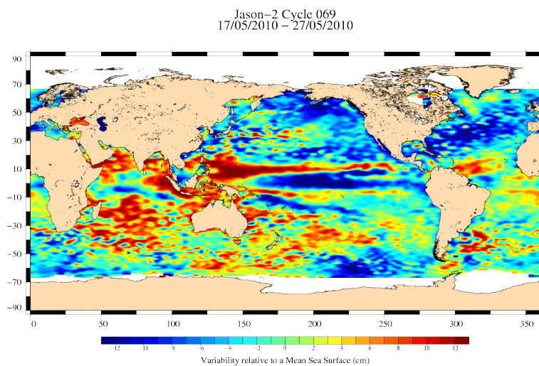
FIG. 18 – Sea level anomaly relative to MSS for cycle 069.
