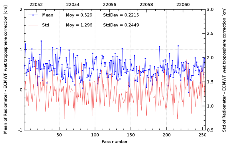
FIG. 11 – Pass monitoring of wet troposphere differences between radiometer and ECMWF model for Jason-2 cycle 069.
