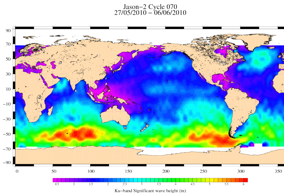
FIG. 5 – Significant wave height for cycle 070.
