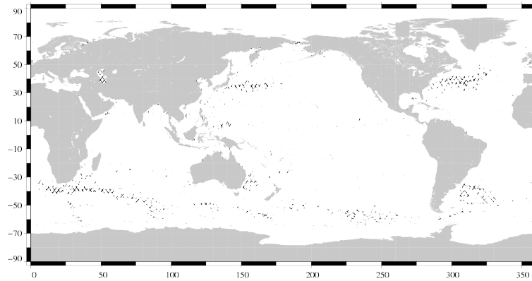
FIG. 19 – Differences higher than a 30 cm threshold for cycle 070.
