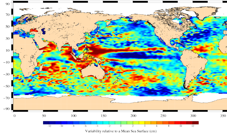
FIG. 18 – Sea level anomaly relative to MSS for cycle 070.
