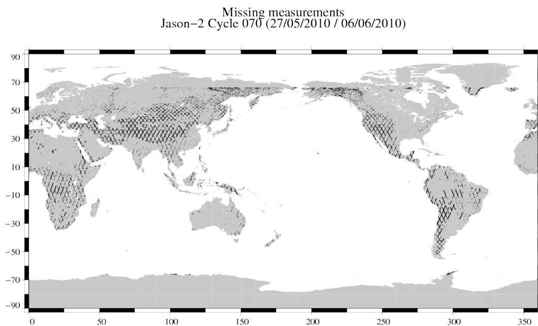
FIG. 1 – Missing measurements for cycle 070.
