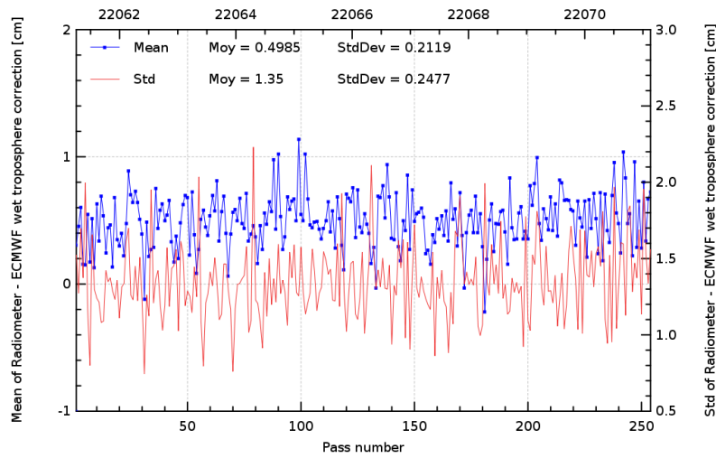
FIG. 11 – Pass monitoring of wet troposphere differences between radiometer and ECMWF model for Jason-2 cycle 070.
