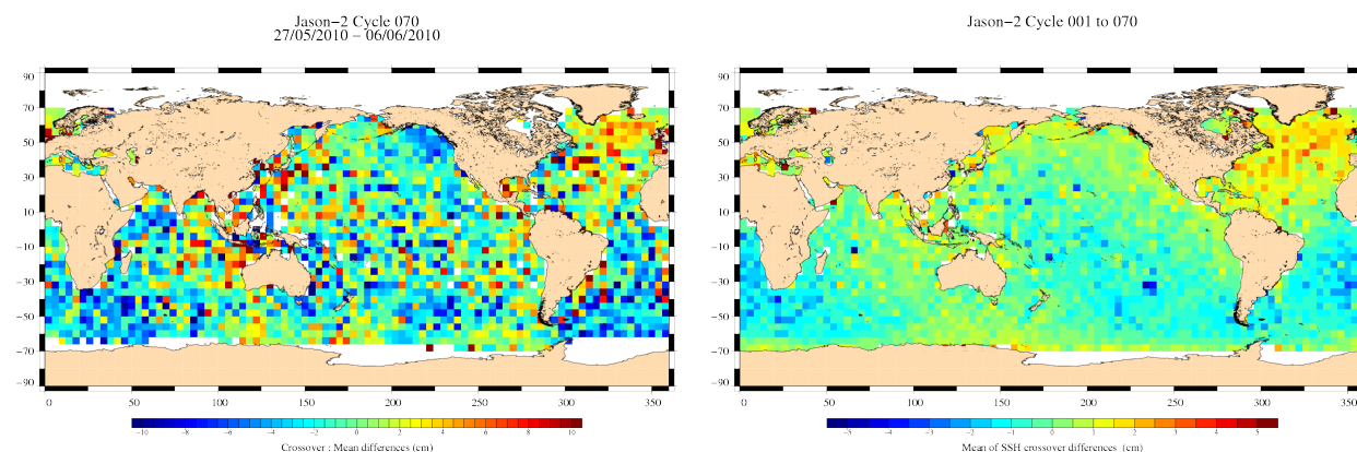
FIG. 13 – Mean SSH at crossovers for cycle 070 (left) and over the whole Jason-2 period (right).
