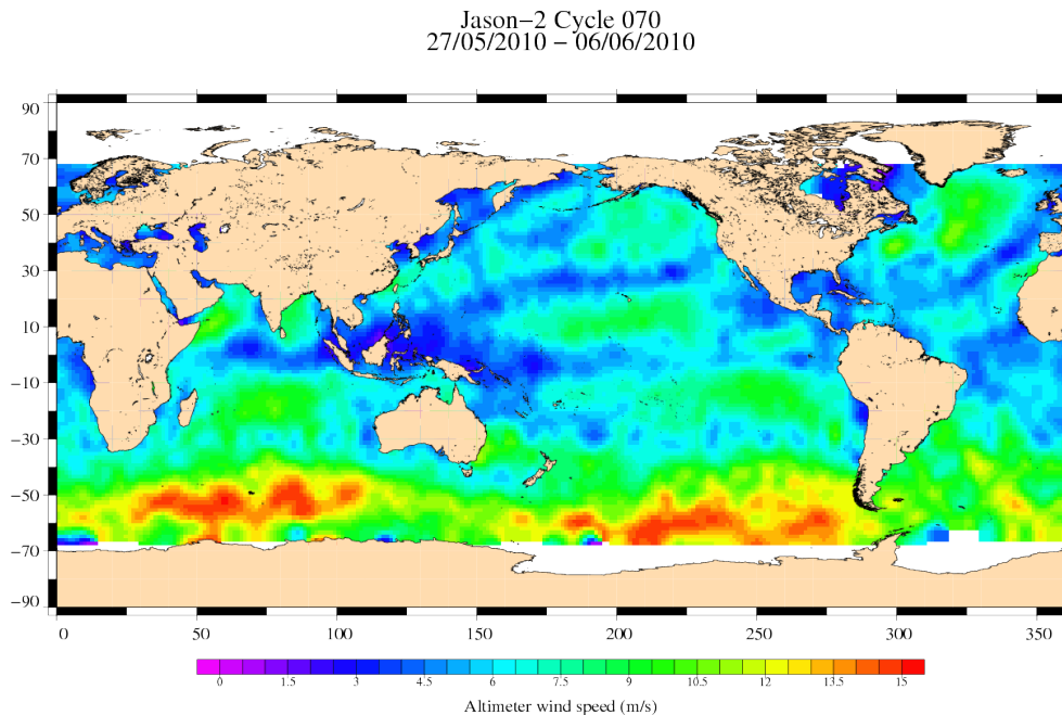
FIG. 9 – Altimeter wind speed for cycle 070.
