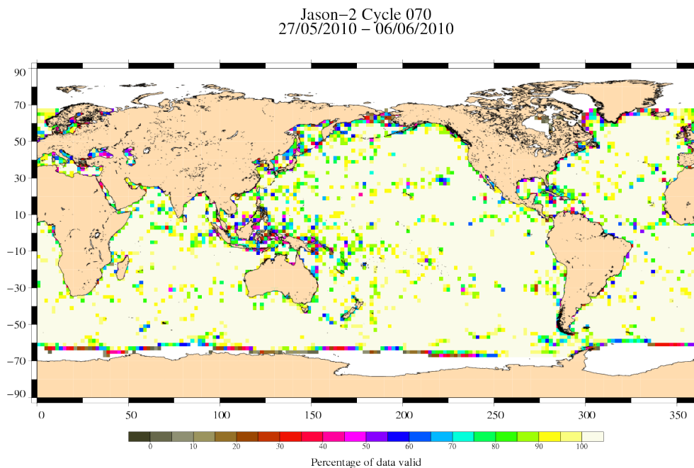
FIG. 3 – Percentage of valid measurements for cycle 070.
