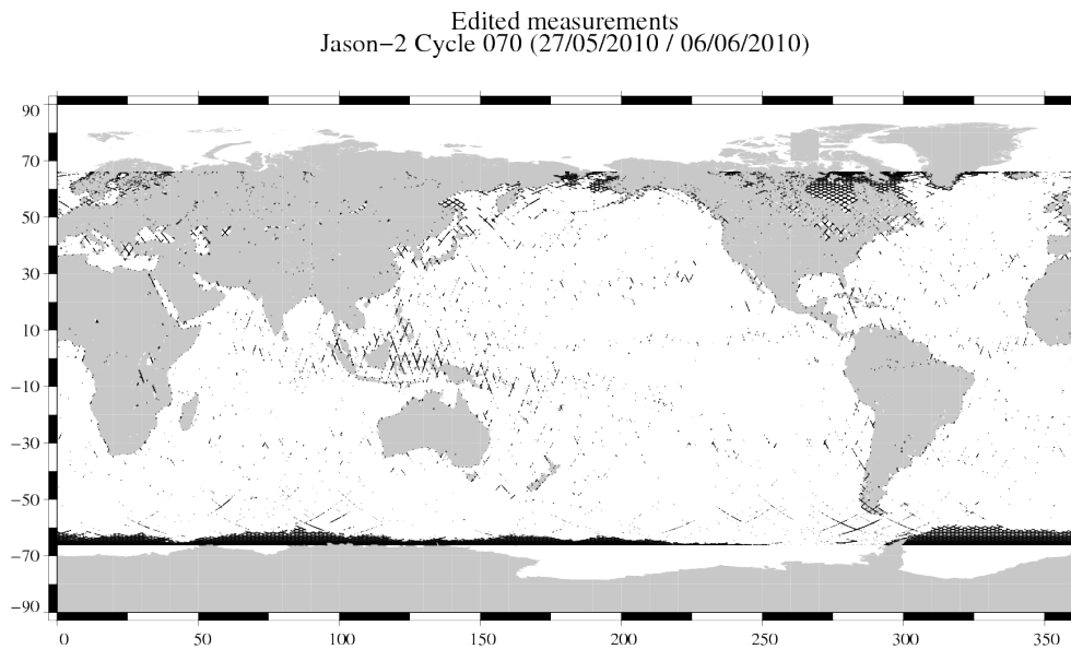
FIG. 2 – Edited measurements for cycle 070.
