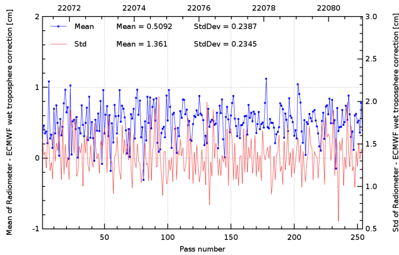
FIG. 11 – Pass monitoring of wet troposphere differences between radiometer and ECMWF model for Jason-2 cycle 071.
