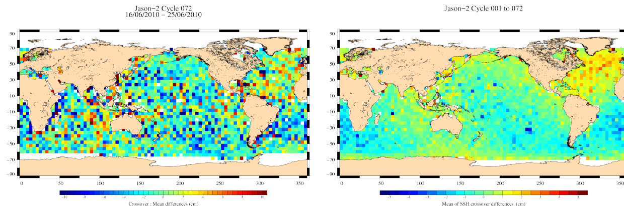
FIG. 13 – Mean SSH at crossovers for cycle 072 (left) and over the whole Jason-2 period (right).
