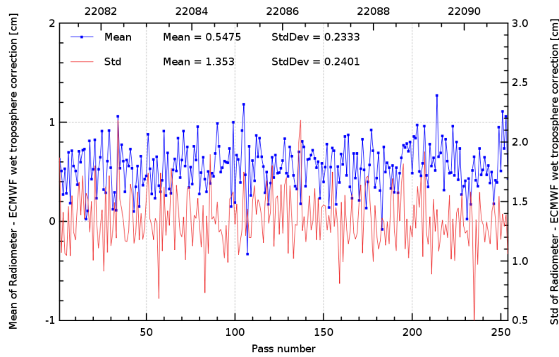
FIG. 11 – Pass monitoring of wet troposphere differences between radiometer and ECMWF model for Jason-2 cycle 072.
