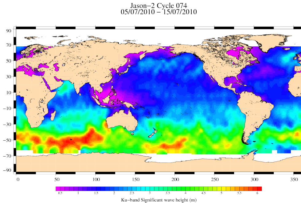
FIG. 5 – Significant wave height for cycle 074.
