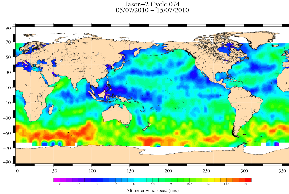
FIG. 9 – Altimeter wind speed for cycle 074.
