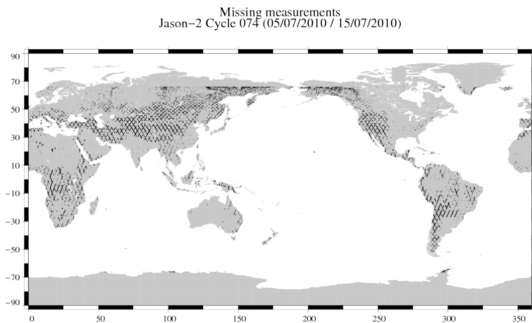
FIG. 1 – Missing measurements for cycle 074.
