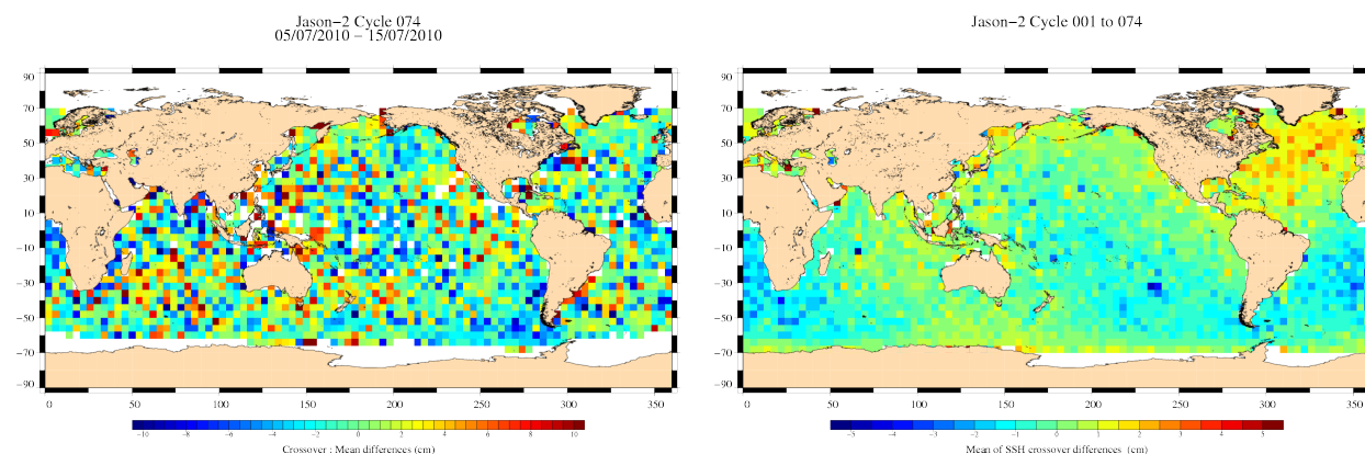
FIG. 13 – Mean SSH at crossovers for cycle 074 (left) and over the whole Jason-2 period (right).
