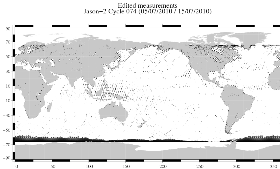
FIG. 2 – Edited measurements for cycle 074.
