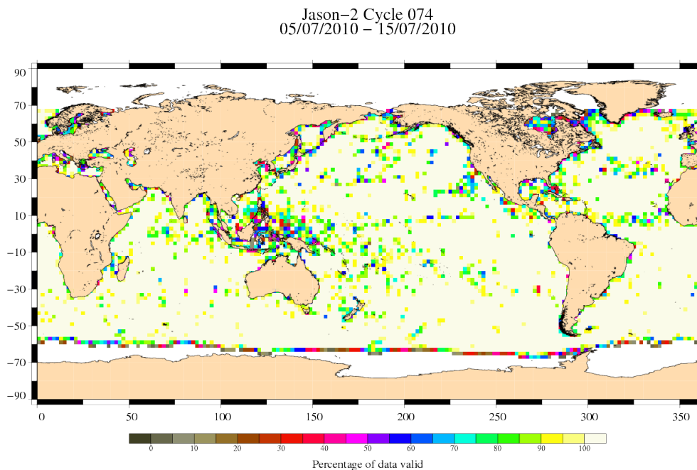
FIG. 3 – Percentage of valid measurements for cycle 074.
