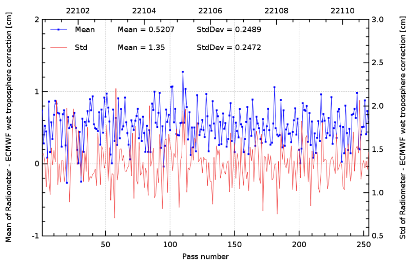
FIG. 11 – Pass monitoring of wet troposphere differences between radiometer and ECMWF model for Jason-2 cycle 074.
