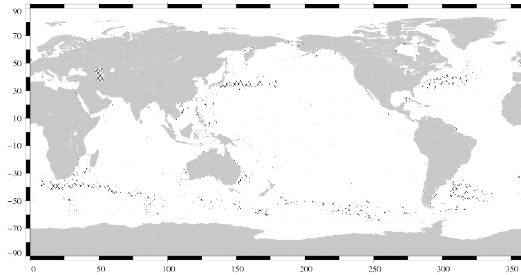
FIG. 19 – Differences higher than a 30 cm threshold for cycle 074.
