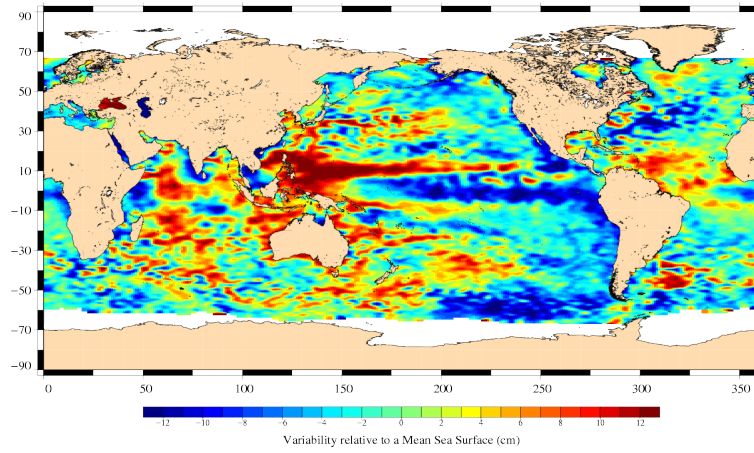
FIG. 18 – Sea level anomaly relative to MSS for cycle 074.
