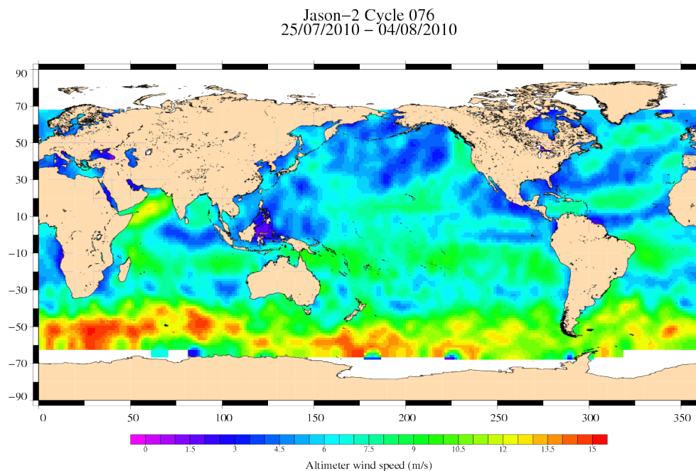
FIG. 9 – Altimeter wind speed for cycle 076.
