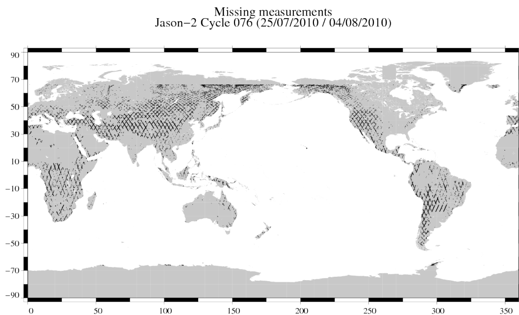
FIG. 1 – Missing measurements for cycle 076.
