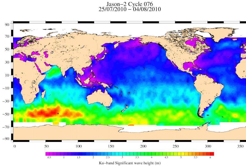
FIG. 5 – Significant wave height for cycle 076.
