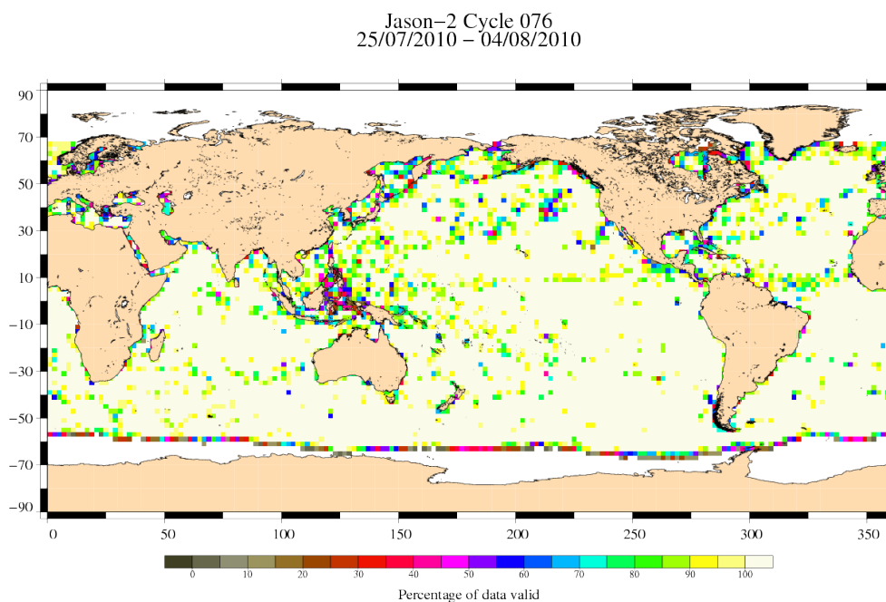
FIG. 3 – Percentage of valid measurements for cycle 076.
