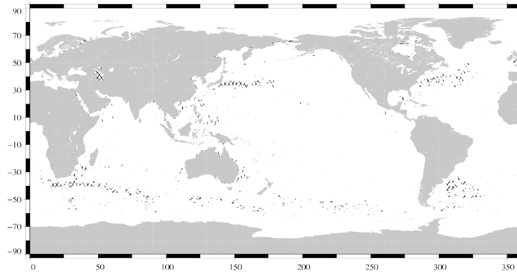
FIG. 19 – Differences higher than a 30 cm threshold for cycle 076.
