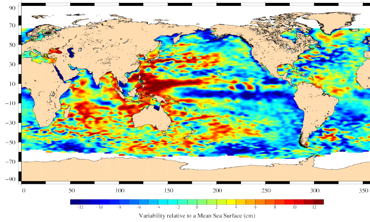
FIG. 18 – Sea level anomaly relative to MSS for cycle 076.
