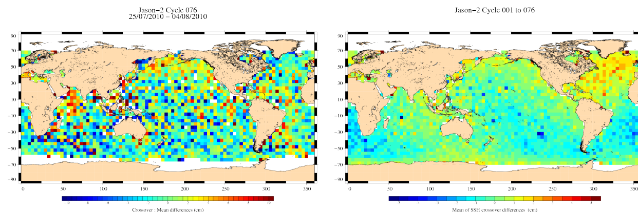
FIG. 13 – Mean SSH at crossovers for cycle 076 (left) and over the whole Jason-2 period (right).
