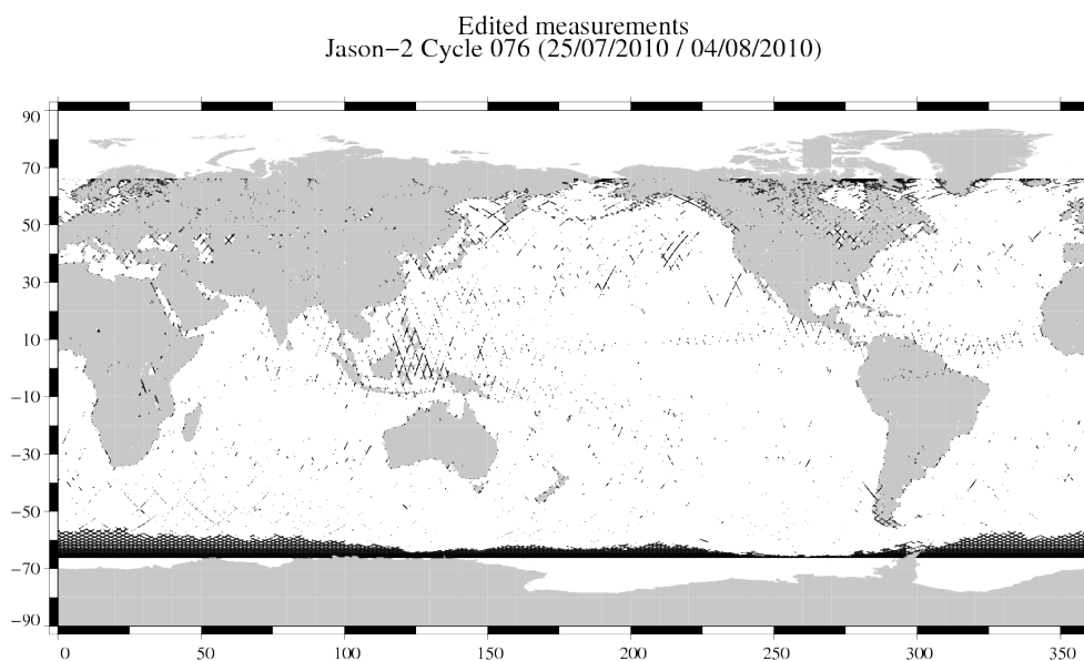
FIG. 2 – Edited measurements for cycle 076.
