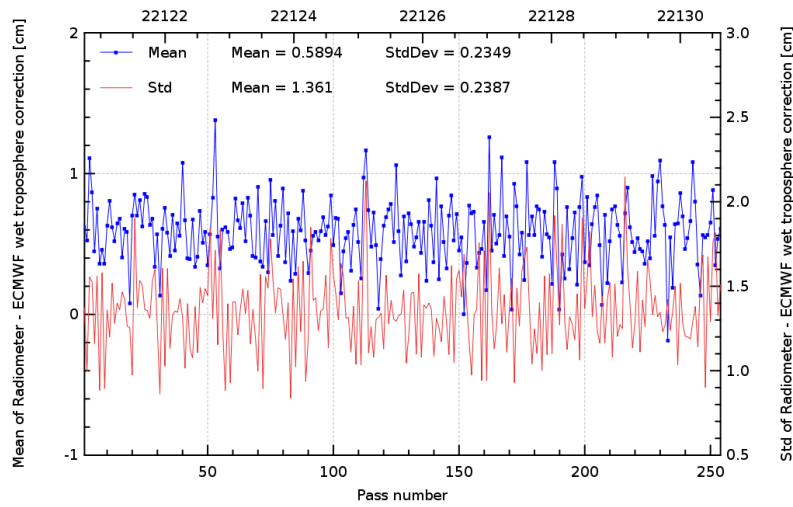
FIG. 11 – Pass monitoring of wet troposphere differences between radiometer and ECMWF model for Jason-2 cycle 076.
