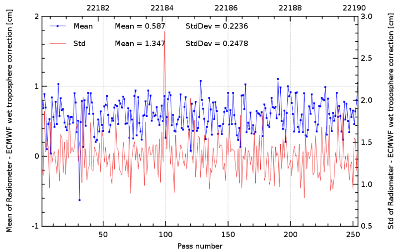
FIG. 12 – Pass monitoring of wet troposphere differences between radiometer and ECMWF model for Jason-2 cycle 082.
