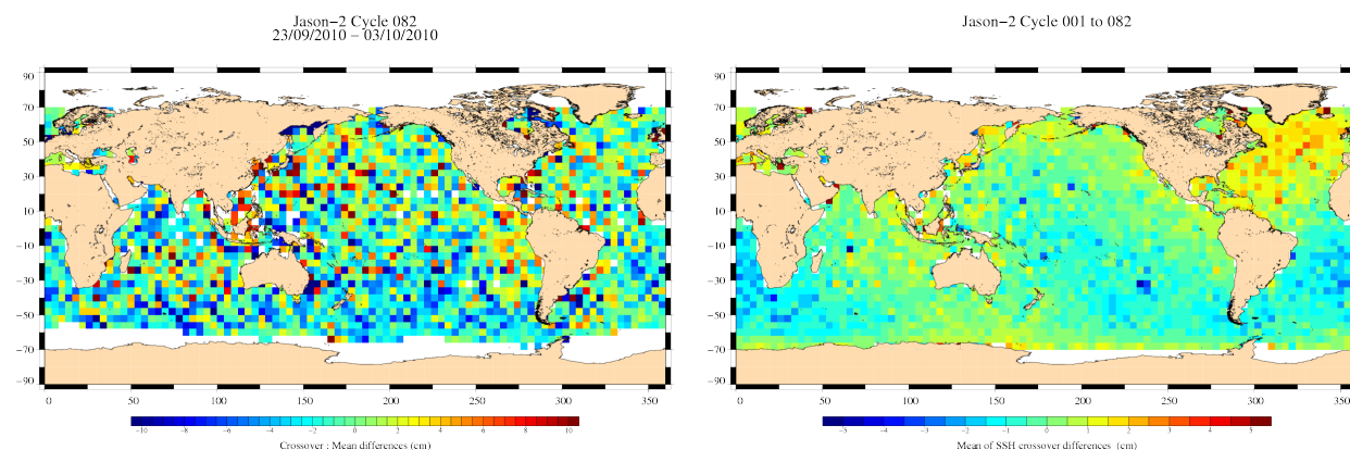
FIG. 14 – Mean SSH at crossovers for cycle 082 (left) and over the whole Jason-2 period (right).
