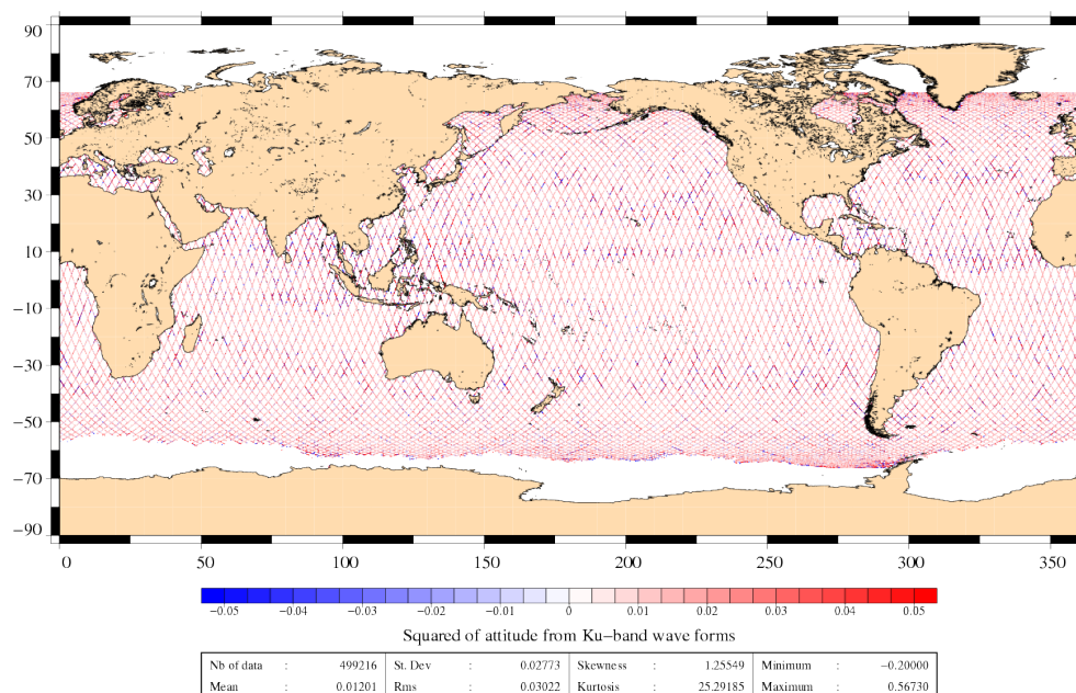
FIG. 4 – Apparent squared mispointing from waveforms for cycle 082.
