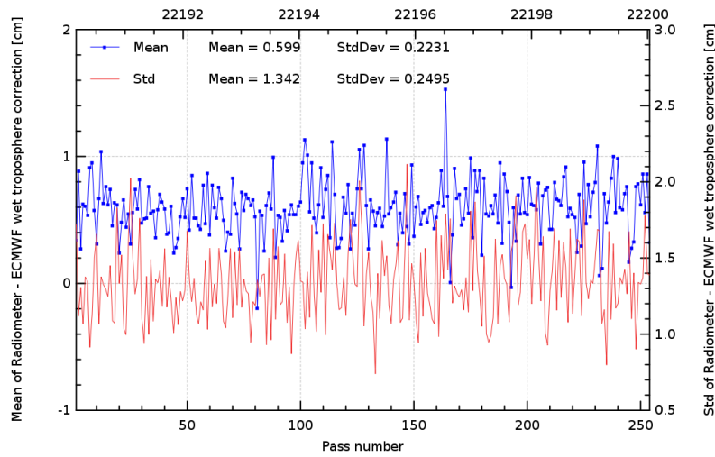
FIG. 11 – Pass monitoring of wet troposphere differences between radiometer and ECMWF model for Jason-2 cycle 083.
