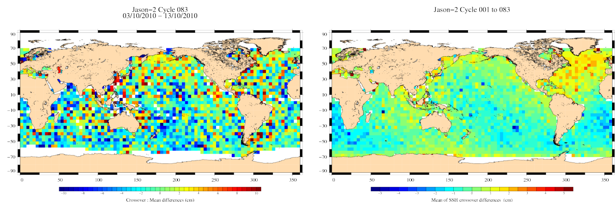
FIG. 13 – Mean SSH at crossovers for cycle 083 (left) and over the whole Jason-2 period (right).
