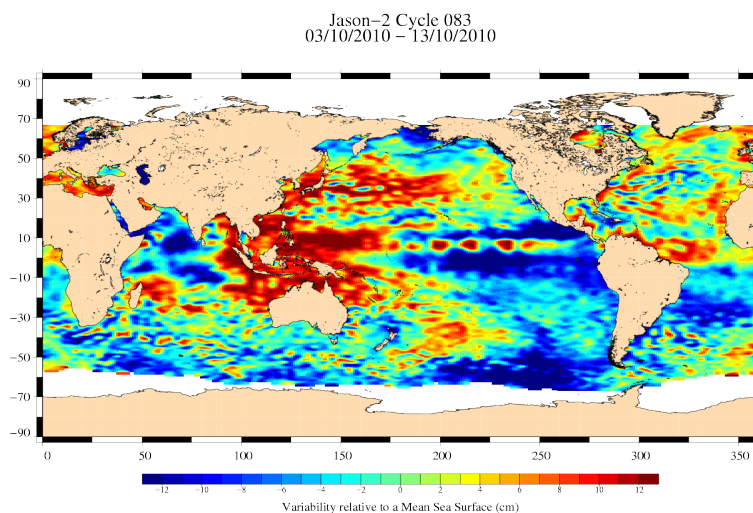
FIG. 18 – Sea level anomaly relative to MSS for cycle 083.
