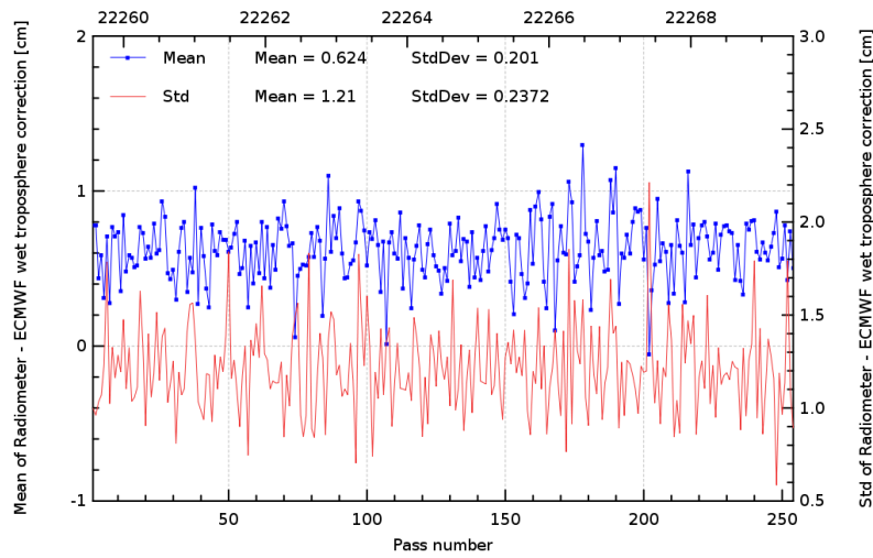
FIG. 11 – Pass monitoring of wet troposphere differences between radiometer and ECMWF model for Jason-2 cycle 090.
