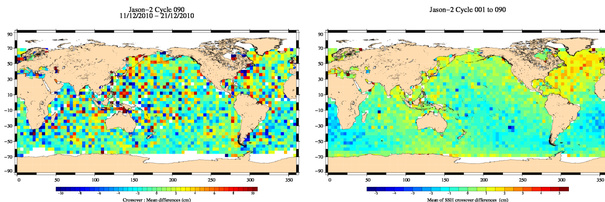
FIG. 13 – Mean SSH at crossovers for cycle 090 (left) and over the whole Jason-2 period (right).
