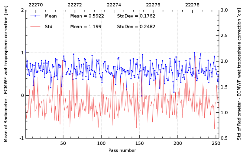
FIG. 11 – Pass monitoring of wet troposphere differences between radiometer and ECMWF model for Jason-2 cycle 091.
