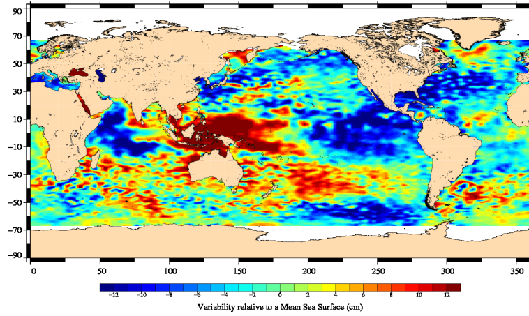
Jason-2 Cycle 094 20/01/2011 – 30/01/2011
