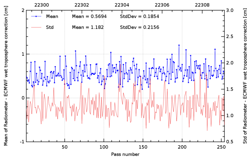
FIG. 11 – Pass monitoring of wet troposphere differences between radiometer and ECMWF model for Jason-2 cycle 094.
