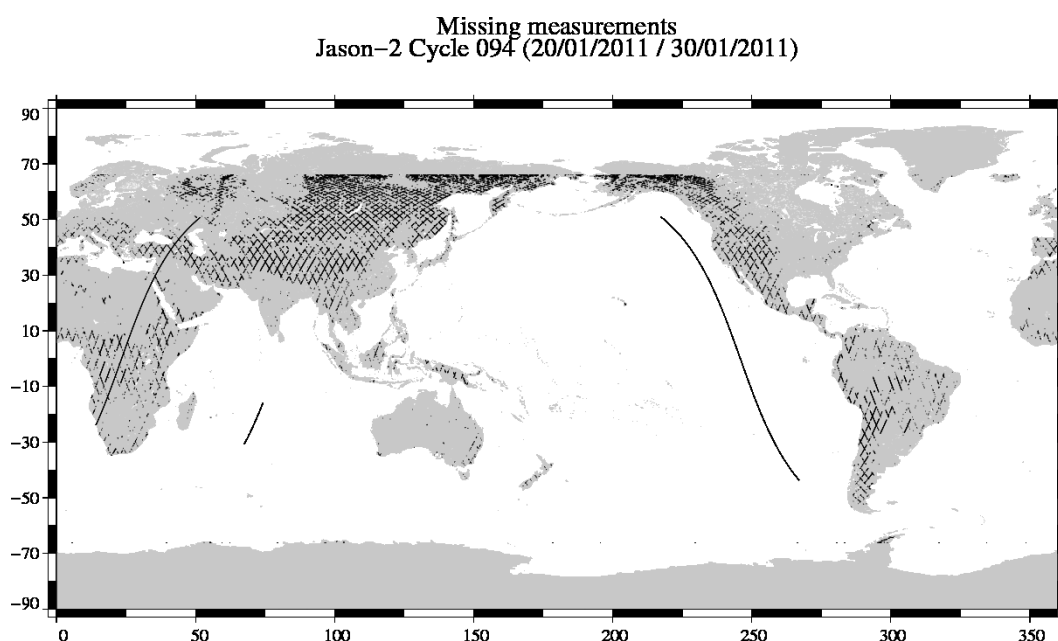
FIG. 1 – Missing measurements for cycle 094.
