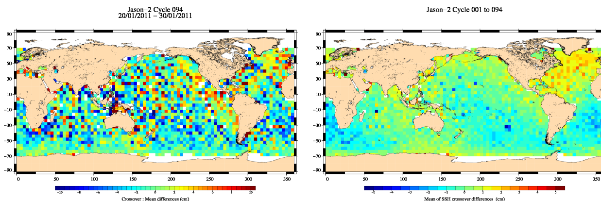
FIG. 13 – Mean SSH at crossovers for cycle 094 (left) and over the whole Jason-2 period (right).
