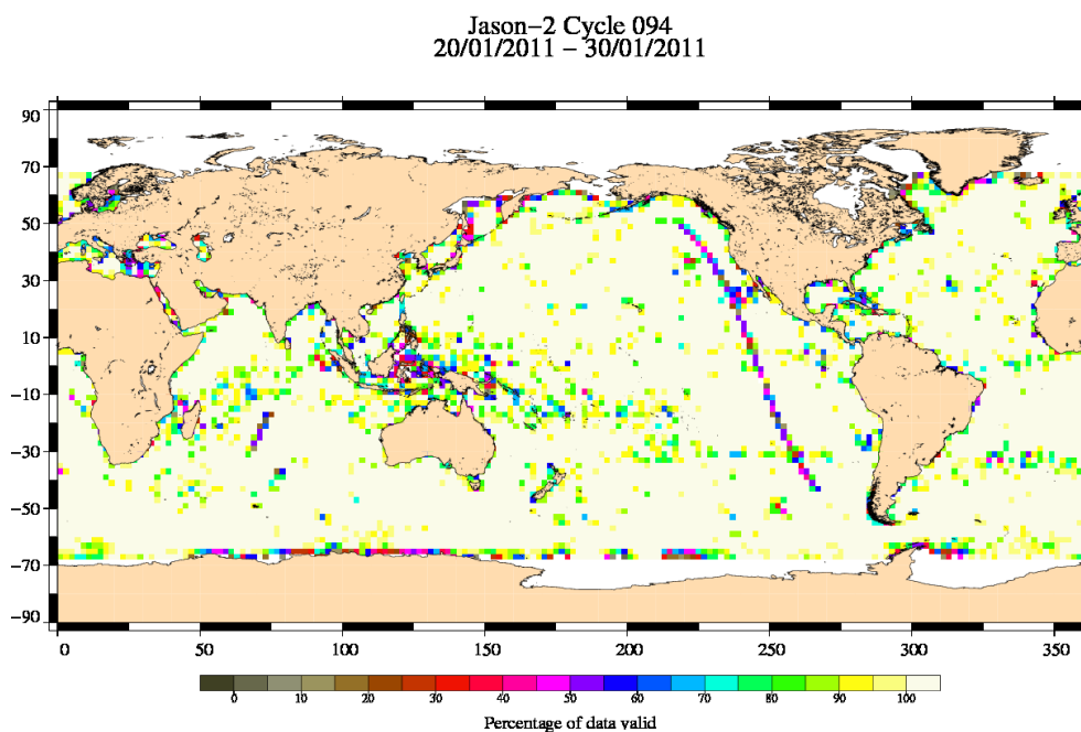
FIG. 3 – Percentage of valid measurements for cycle 094.
