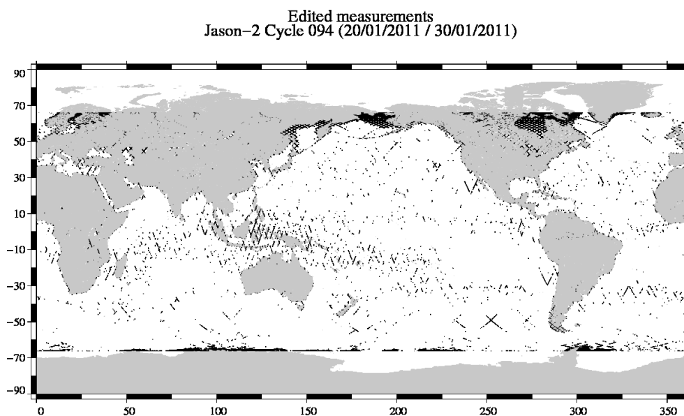
FIG. 2 – Edited measurements for cycle 094.
