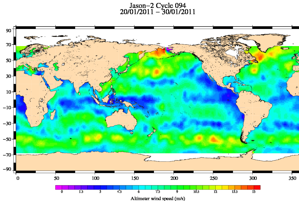
FIG. 9 – Altimeter wind speed for cycle 094.
