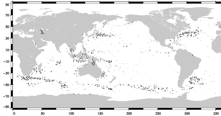
Valid data: (SSH – MSS) differences greater than 30 cm Jason-2 Cycle 094 (20/01/2011 / 30/01/2011)
