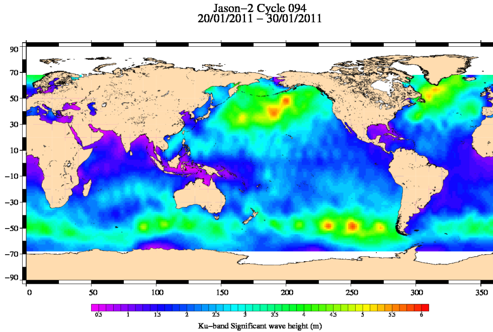
FIG. 5 – Significant wave height for cycle 094.
