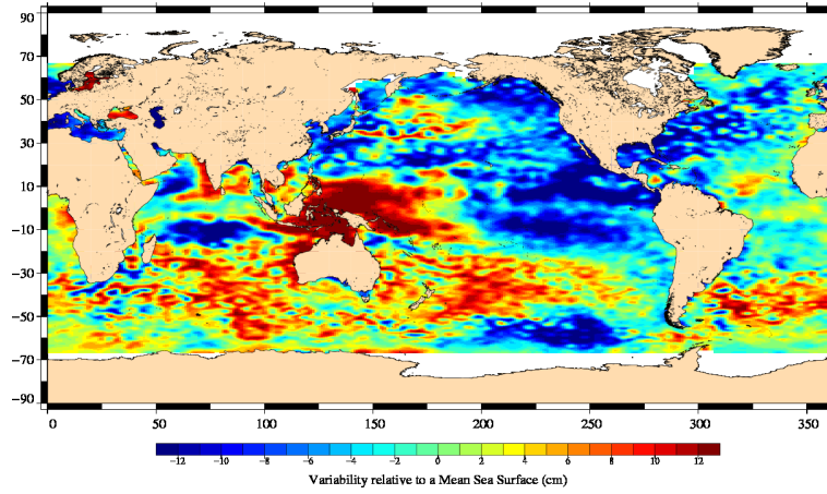
Jason-2 Cycle 096 09/02/2011 – 18/02/2011
