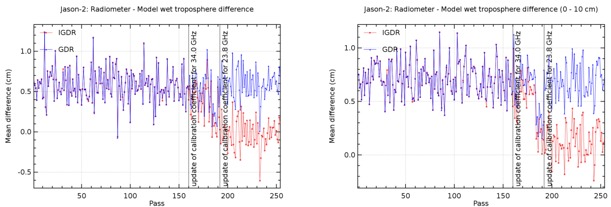
FIG. 12 – Pass monitoring of wet troposphere differences between radiometer and ECMWF model for Jason-2 IGDR and GDR data cycle 096. Right : looking only on dry measurements (wet troposphere correction limited between 0 and 10 cm).
