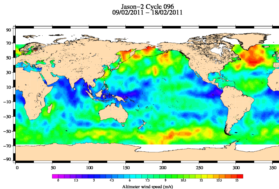
FIG. 9 – Altimeter wind speed for cycle 096.
