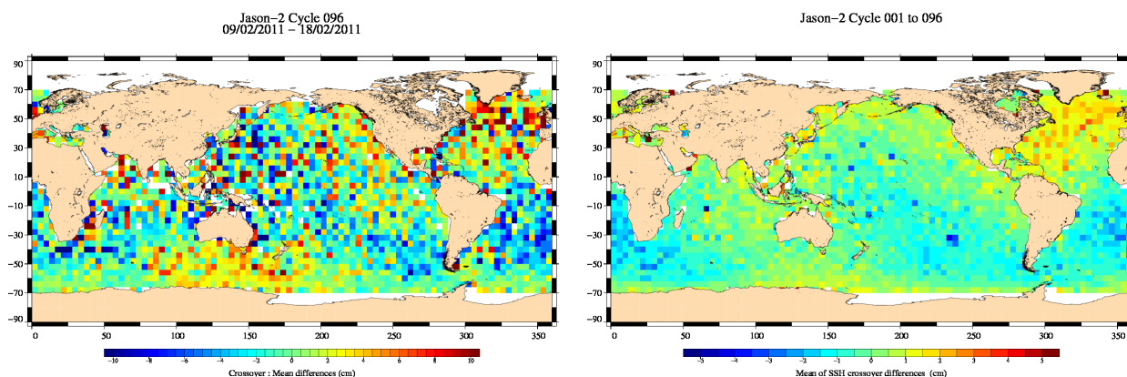
FIG. 14 – Mean SSH at crossovers for cycle 096 (left) and over the whole Jason-2 period (right).
