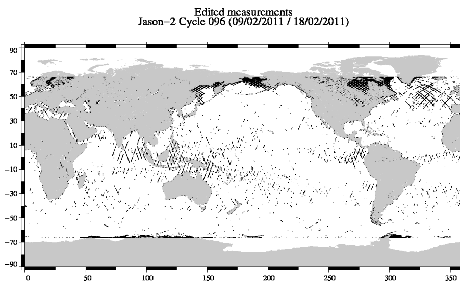
FIG. 2 – Edited measurements for cycle 096.
