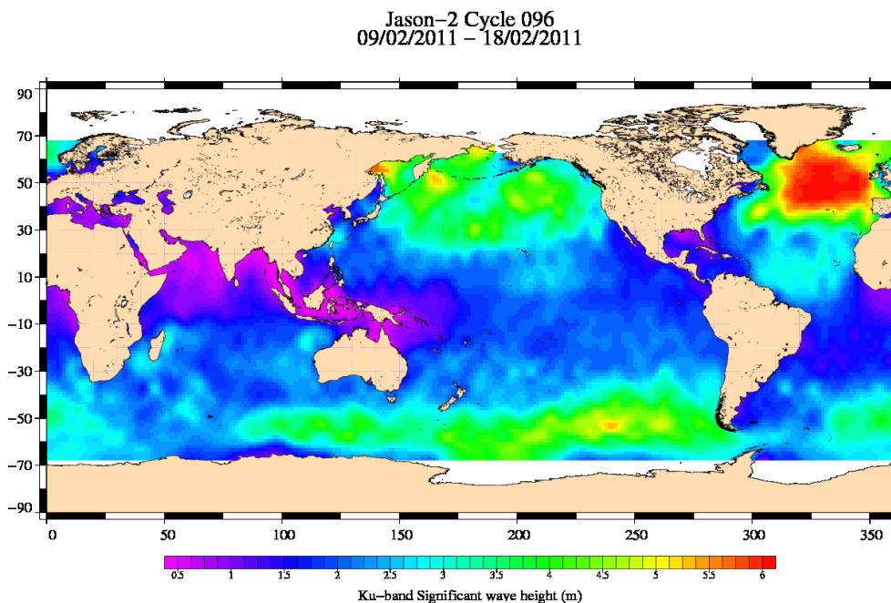
FIG. 5 – Significant wave height for cycle 096.
