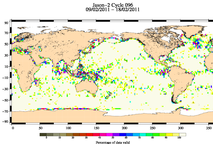
FIG. 3 – Percentage of valid measurements for cycle 096.
