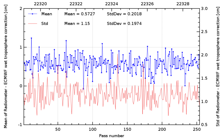
FIG. 11 – Pass monitoring of wet troposphere differences between radiometer and ECMWF model for Jason-2 cycle 096.
