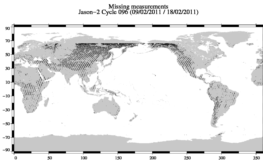
FIG. 1 – Missing measurements for cycle 096.
