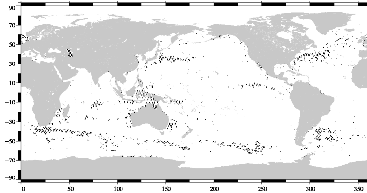
Valid data: (SSH – MSS) differences greater than 30 cm Jason-2 Cycle 096 (09/02/2011 / 18/02/2011)
