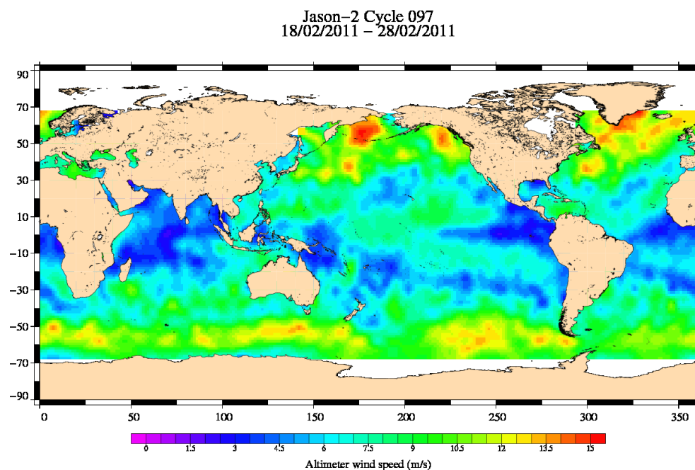
FIG. 9 – Altimeter wind speed for cycle 097.
