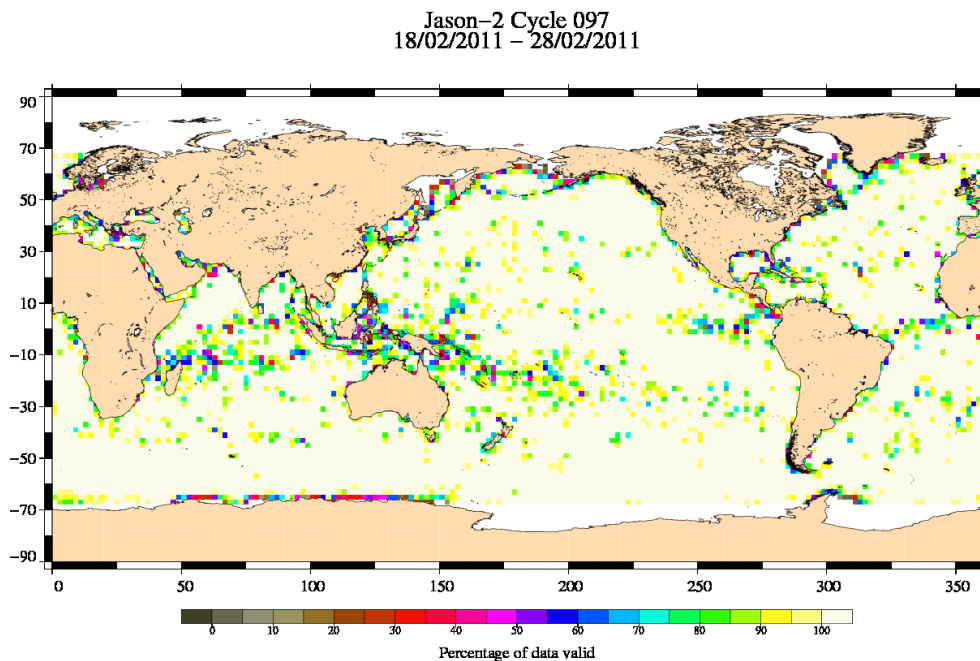
FIG. 3 – Percentage of valid measurements for cycle 097.
