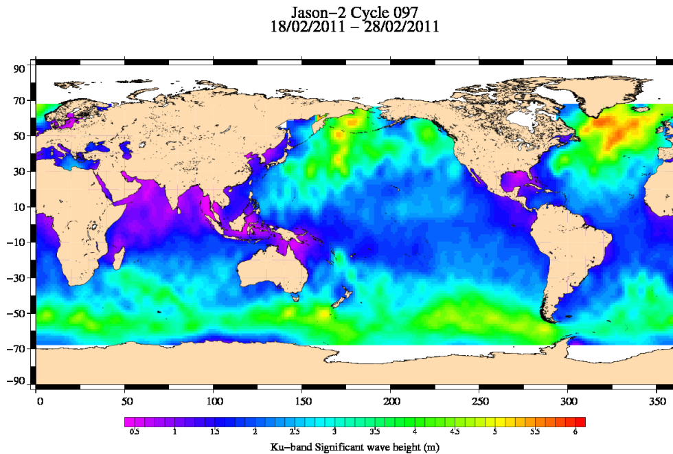
FIG. 5 – Significant wave height for cycle 097.
