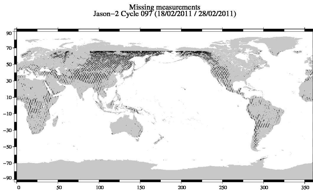
FIG. 1 – Missing measurements for cycle 097.
