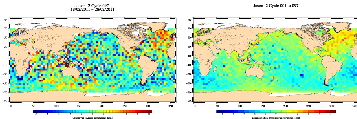
FIG. 13 – Mean SSH at crossovers for cycle 097 (left) and over the whole Jason-2 period (right).
