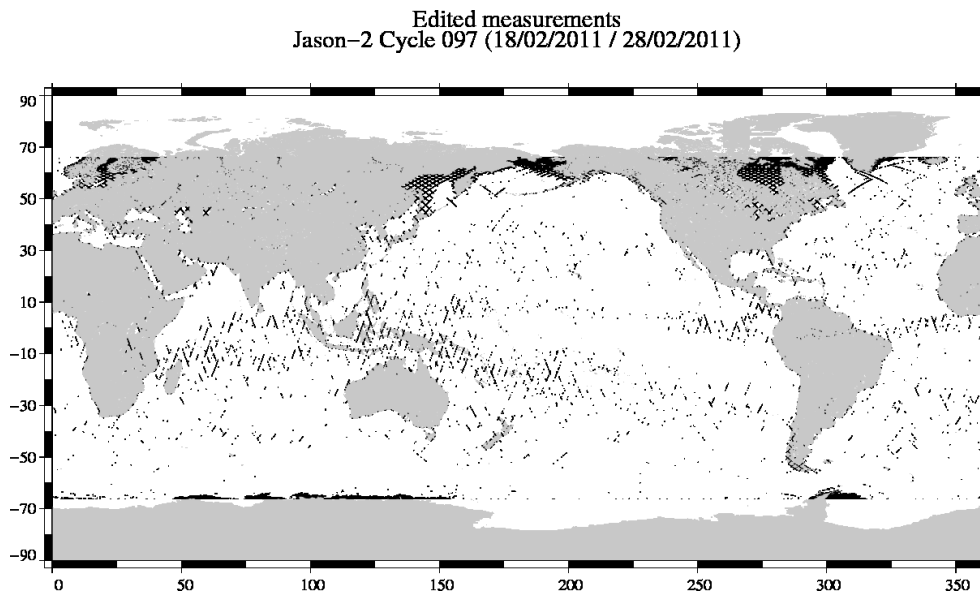
FIG. 2 – Edited measurements for cycle 097.
