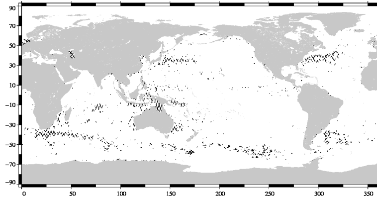
Valid data: (SSH – MSS) differences greater than 30 cm Jason-2 Cycle 097 (18/02/2011 / 28/02/2011)
