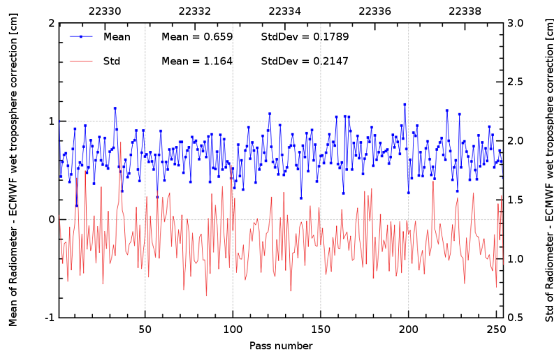
FIG. 11 – Pass monitoring of wet troposphere differences between radiometer and ECMWF model for Jason-2 cycle 097.
