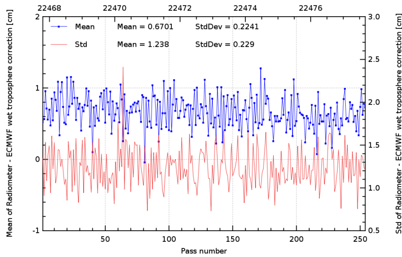
FIG. 12 – Pass monitoring of wet troposphere differences between radiometer and ECMWF model for Jason-2 cycle 111.
