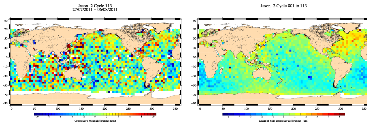
FIG. 14 – Mean SSH at crossovers for cycle 113 (left) and over the whole Jason-2 period (right).
