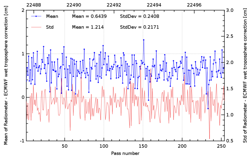
FIG. 11 – Pass monitoring of wet troposphere differences between radiometer and ECMWF model for Jason-2 cycle 113.
