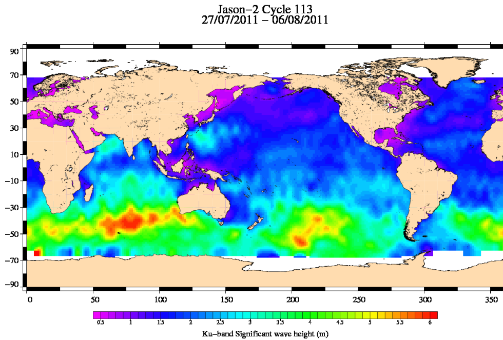
FIG. 5 – Significant wave height for cycle 113.
