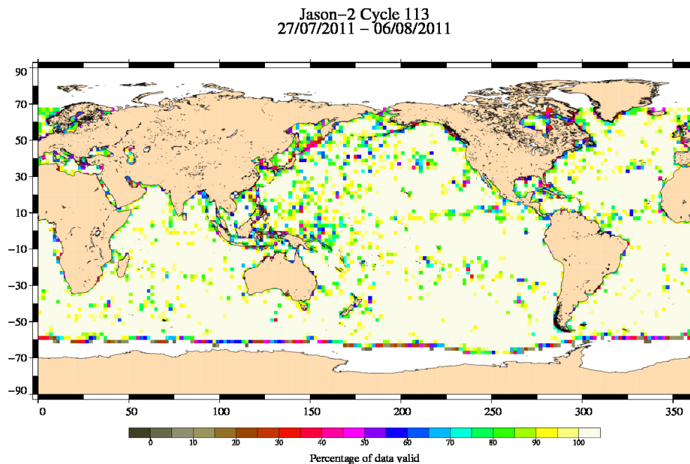
FIG. 3 – Percentage of valid measurements for cycle 113.
