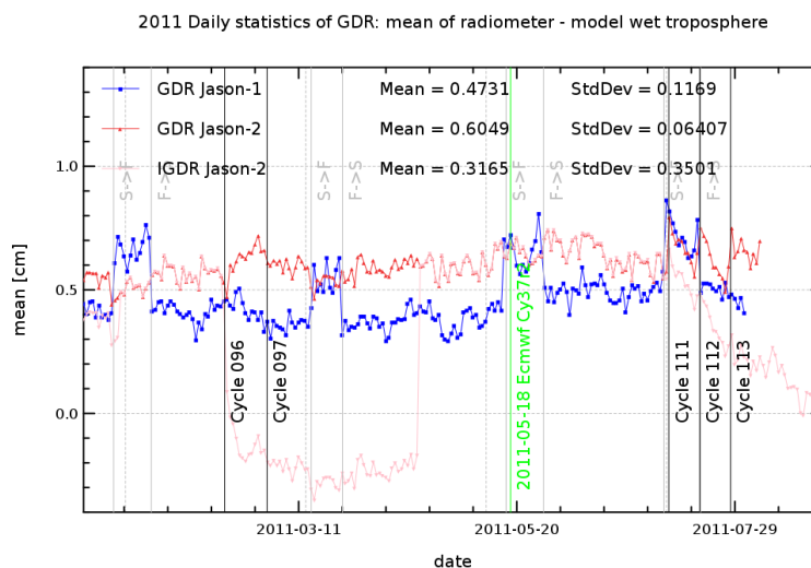
FIG. 13 – Daily monitoring of wet troposphere differences between radiometer and ECMWF model for 2011 for Jason-2 GDR (red), Jason-2 IGDR (pink), Jason-1 GDR (blue). Ecmwf model version changes are indicated by green lines, yaw ramps are indicated by gray lines and black lines indicate new calibration coefficients for AMR.
