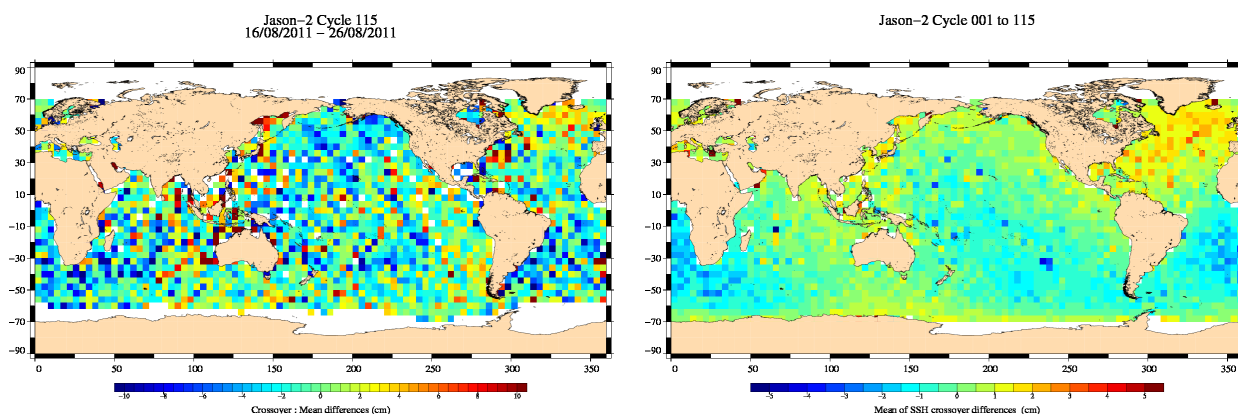
FIG. 13 – Mean SSH at crossovers for cycle 115 (left) and over the whole Jason-2 period (right).
