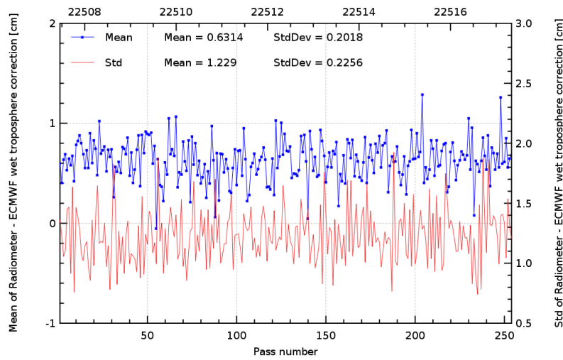
FIG. 11 – Pass monitoring of wet troposphere differences between radiometer and ECMWF model for Jason-2 cycle 115.
