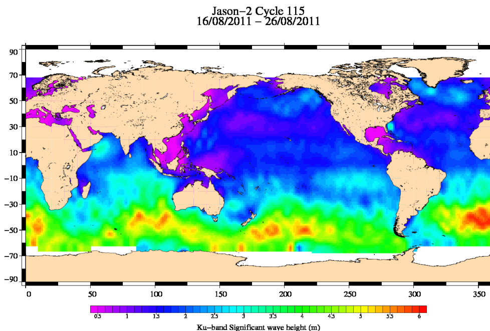
FIG. 5 – Significant wave height for cycle 115.
