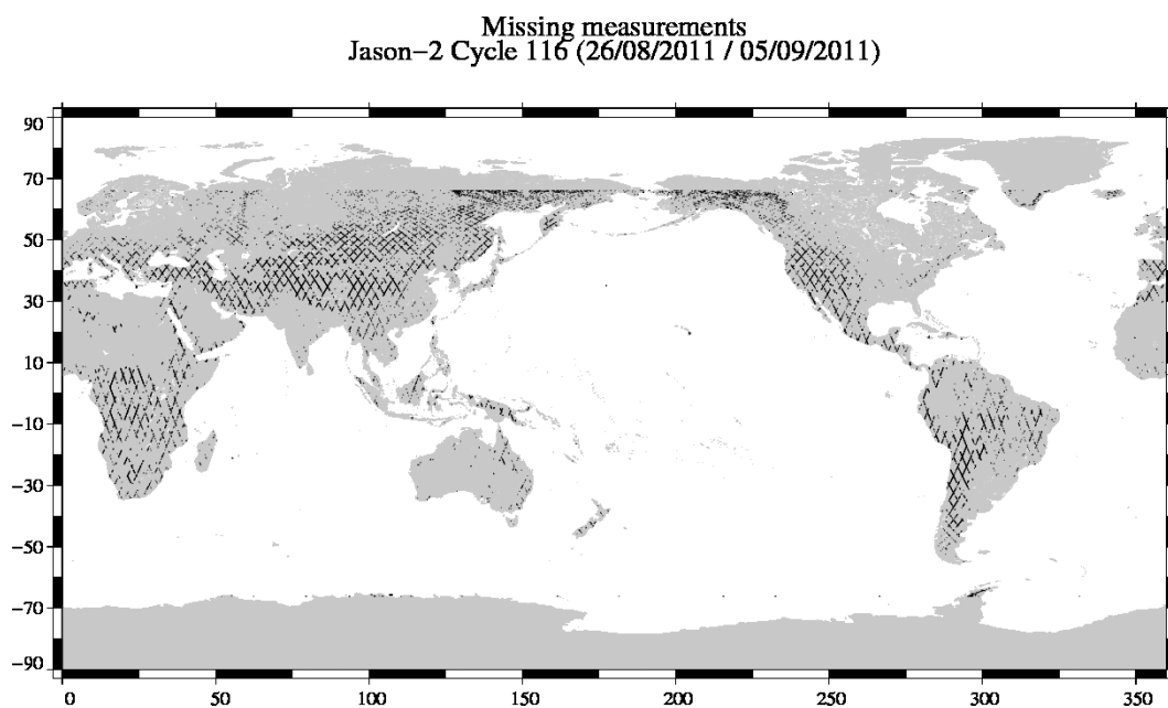
FIG. 1 – Missing measurements for cycle 116.
