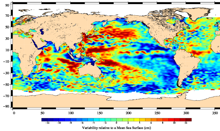
FIG. 19 – Sea level anomaly relative to MSS for cycle 116.
