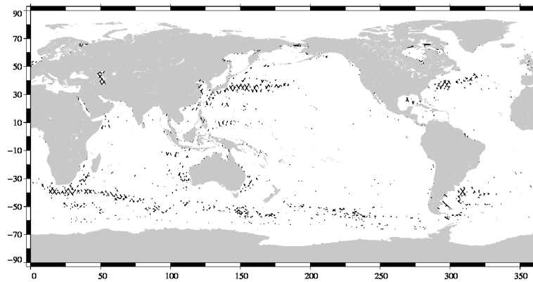
FIG. 20 – Differences higher than a 30 cm threshold for cycle 116.
