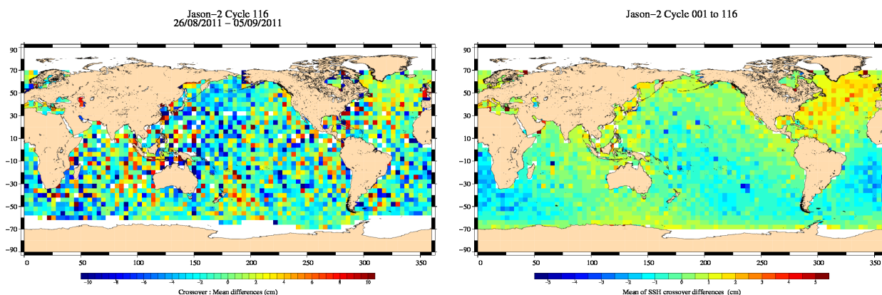
FIG. 14 – Mean SSH at crossovers for cycle 116 (left) and over the whole Jason-2 period (right).
