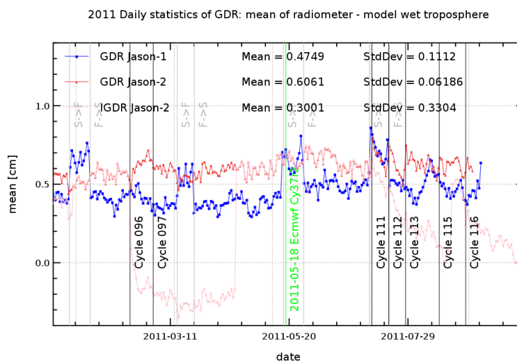
FIG. 13 – Daily monitoring of wet troposphere differences between radiometer and ECMWF model for 2011.
