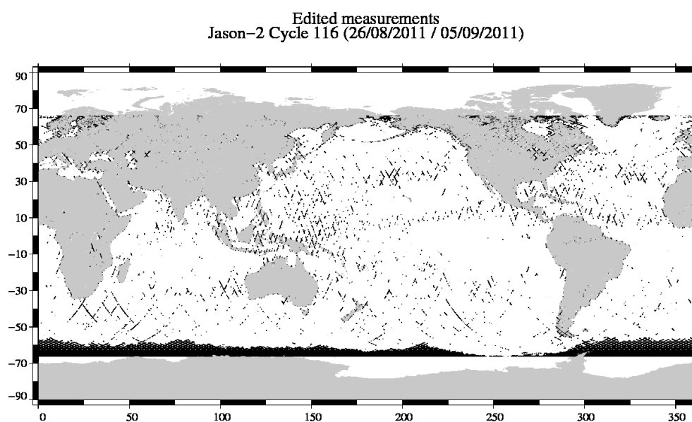
FIG. 2 – Edited measurements for cycle 116.
