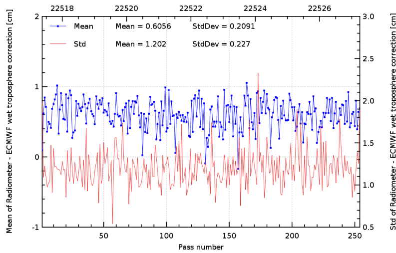
FIG. 11 – Pass monitoring of wet troposphere differences between radiometer and ECMWF model for Jason-2 cycle 116.
