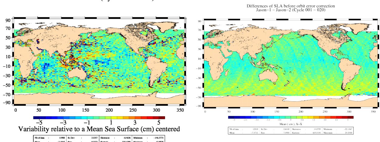
FIG. 21 – Jason-1 – Jason-2 SLA differences averaged over whole Jason-2 period since cycle 022 (left), and for flight formation phase (cycle 001 to 020) (right).
