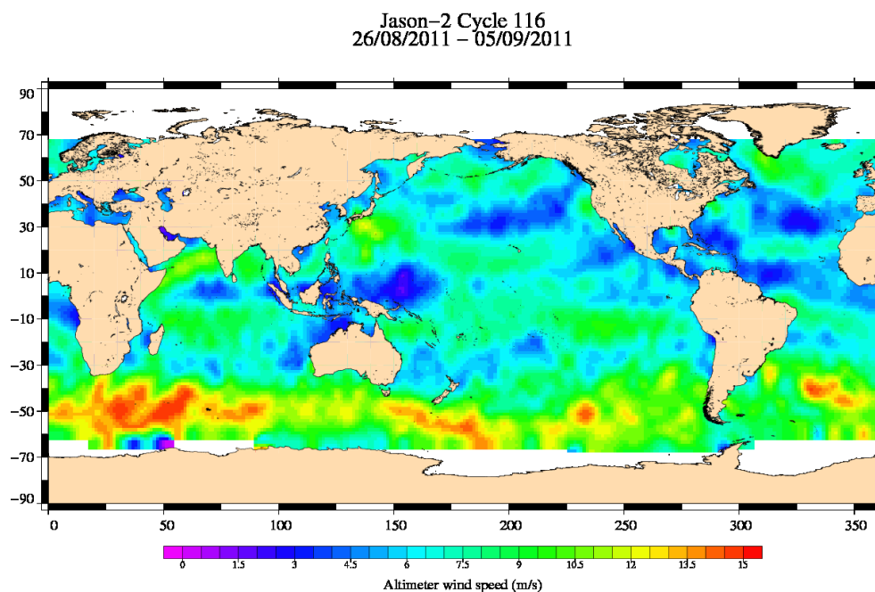
FIG. 9 – Altimeter wind speed for cycle 116.
