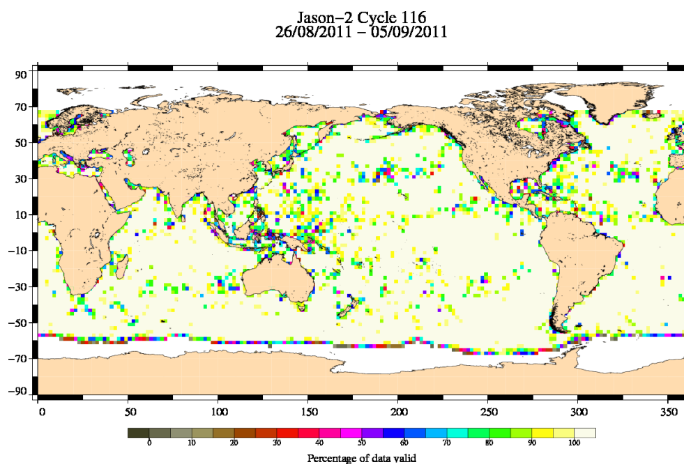
FIG. 3 – Percentage of valid measurements for cycle 116.
