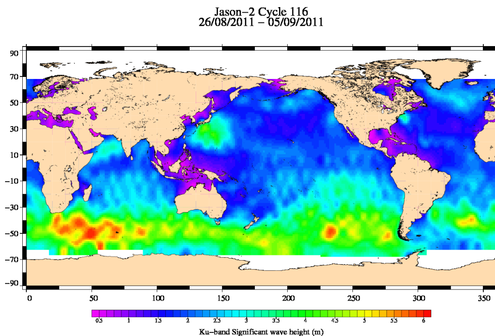
FIG. 5 – Significant wave height for cycle 116.
