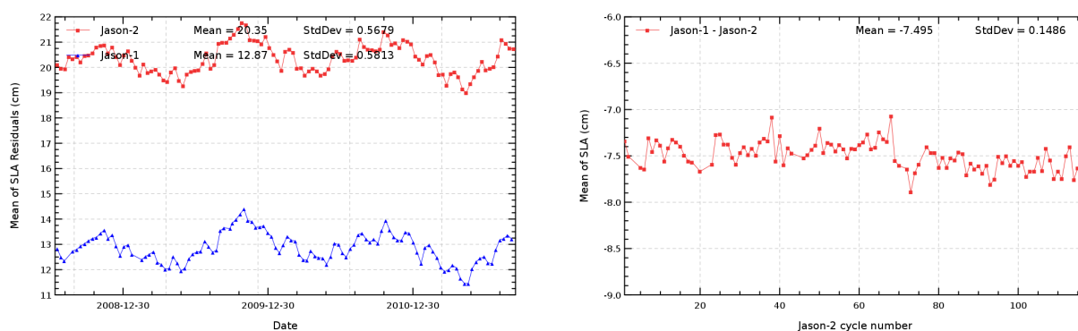
FIG. 17 – Cyclic monitoring of mean SLA for Jason-1 and Jason-2 (left) and differences of (Jason-1 – Jason-2) mean SLA (right).
