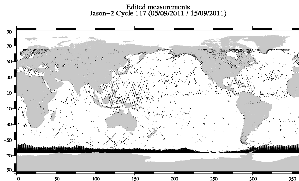
FIG. 2 – Edited measurements for cycle 117.
