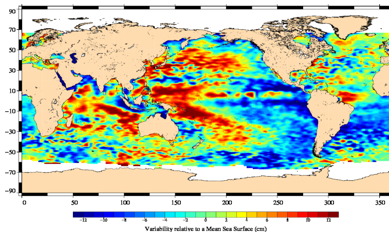
FIG. 18 – Sea level anomaly relative to MSS for cycle 117.
