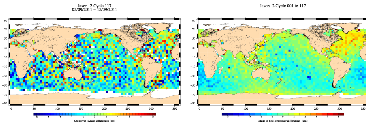
FIG. 13 – Mean SSH at crossovers for cycle 117 (left) and over the whole Jason-2 period (right).
