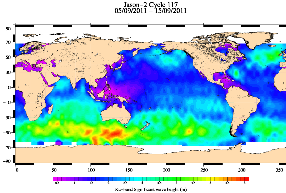
FIG. 5 – Significant wave height for cycle 117.
