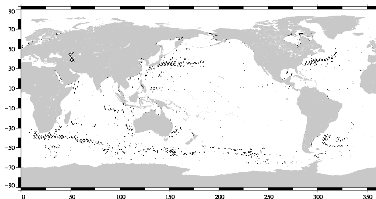
FIG. 19 – Differences higher than a 30 cm threshold for cycle 117.
