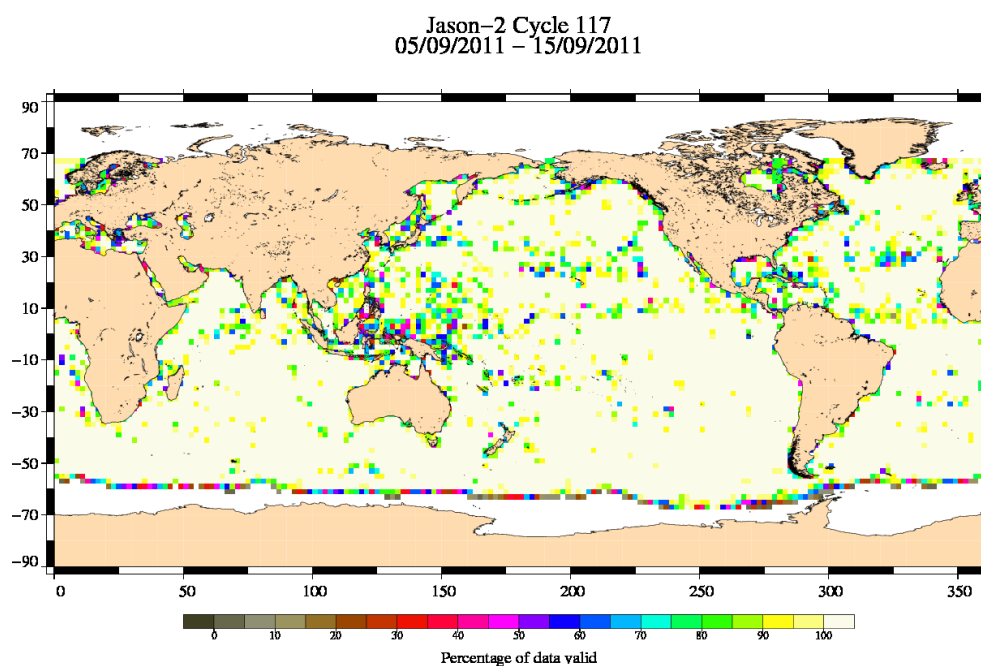
FIG. 3 – Percentage of valid measurements for cycle 117.
