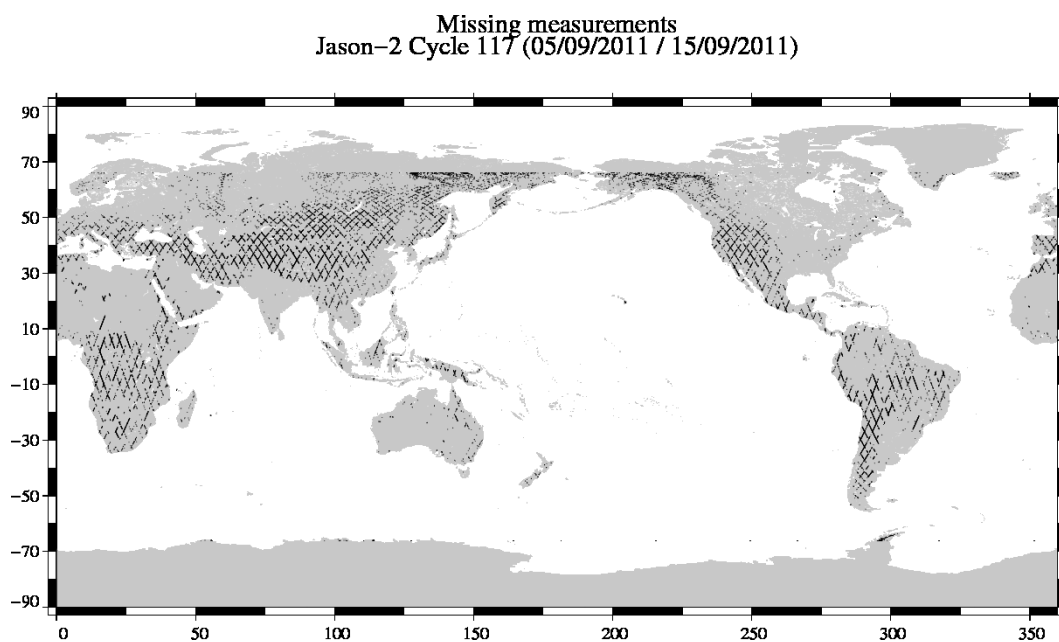
FIG. 1 – Missing measurements for cycle 117.
