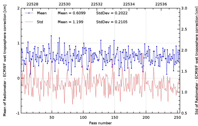
FIG. 11 – Pass monitoring of wet troposphere differences between radiometer and ECMWF model for Jason-2 cycle 117.
