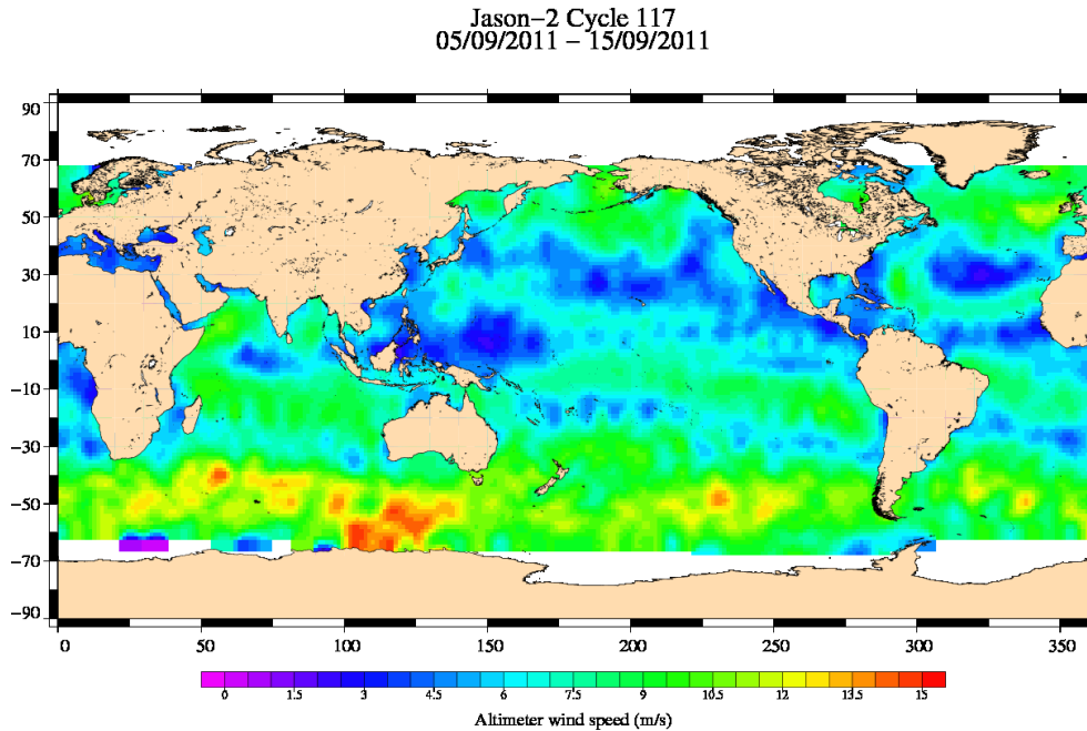
FIG. 9 – Altimeter wind speed for cycle 117.
