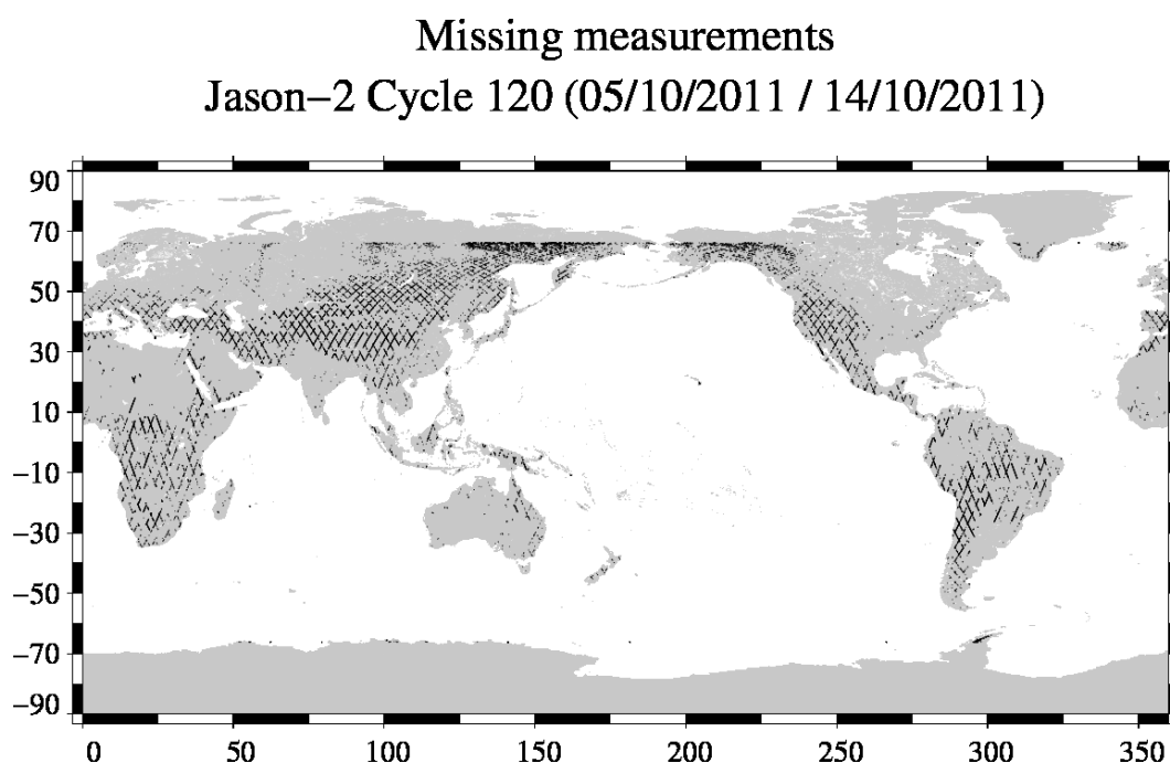
FIG. 1 – Missing measurements for cycle 120.
