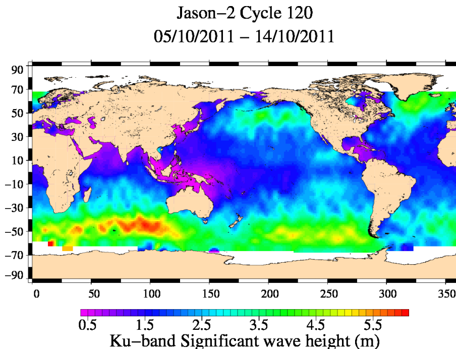
FIG. 5 – Significant wave height for cycle 120.
