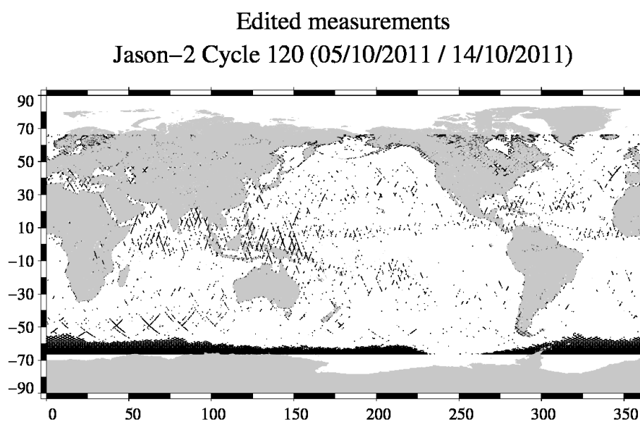
FIG. 2 – Edited measurements for cycle 120.
