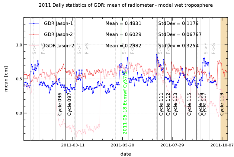
FIG. 13 – Daily monitoring of wet troposphere differences between radiometer and ECMWF model for year 2011.
