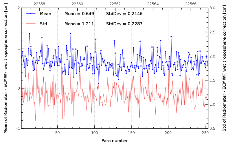
FIG. 11 – Pass monitoring of wet troposphere differences between radiometer and ECMWF model for Jason-2 cycle 120.
