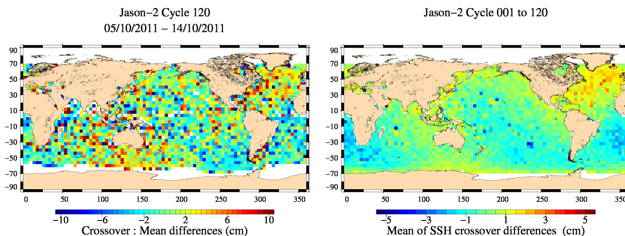
FIG. 14 – Mean SSH at crossovers for cycle 120 (left) and over the whole Jason-2 period (right).
