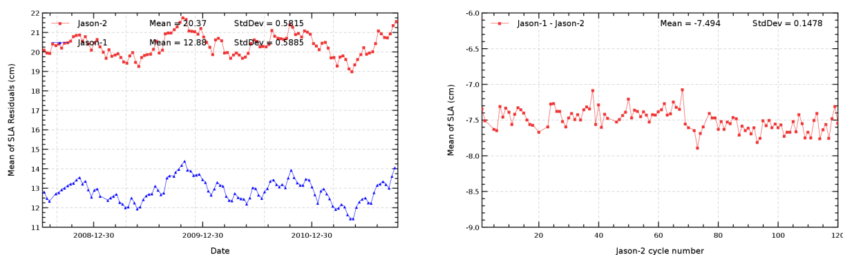
FIG. 18 – Cyclic monitoring of mean SLA for Jason-1 and Jason-2 (left) and differences of (Jason-1 – Jason-2) mean SLA (right).
