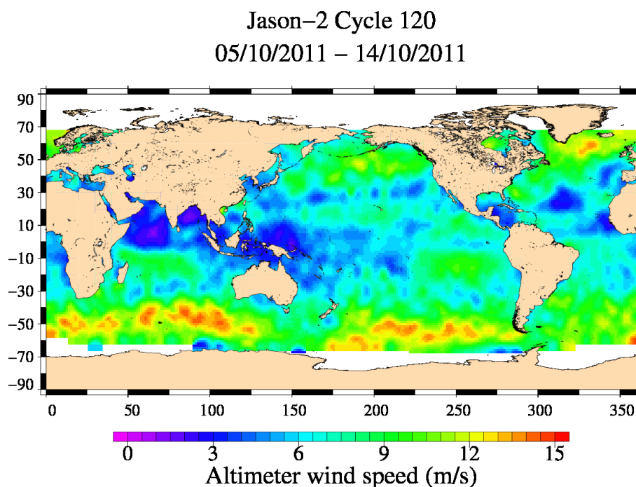
FIG. 9 – Altimeter wind speed for cycle 120.
