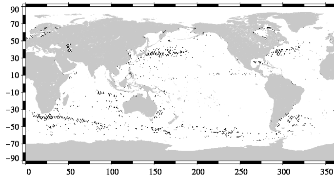
FIG. 20 – Differences higher than a 30 cm threshold for cycle 120.
