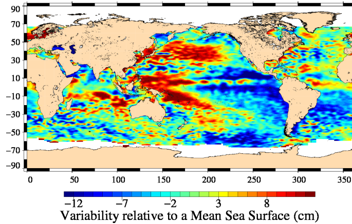
FIG. 19 – Sea level anomaly relative to MSS for cycle 120.
