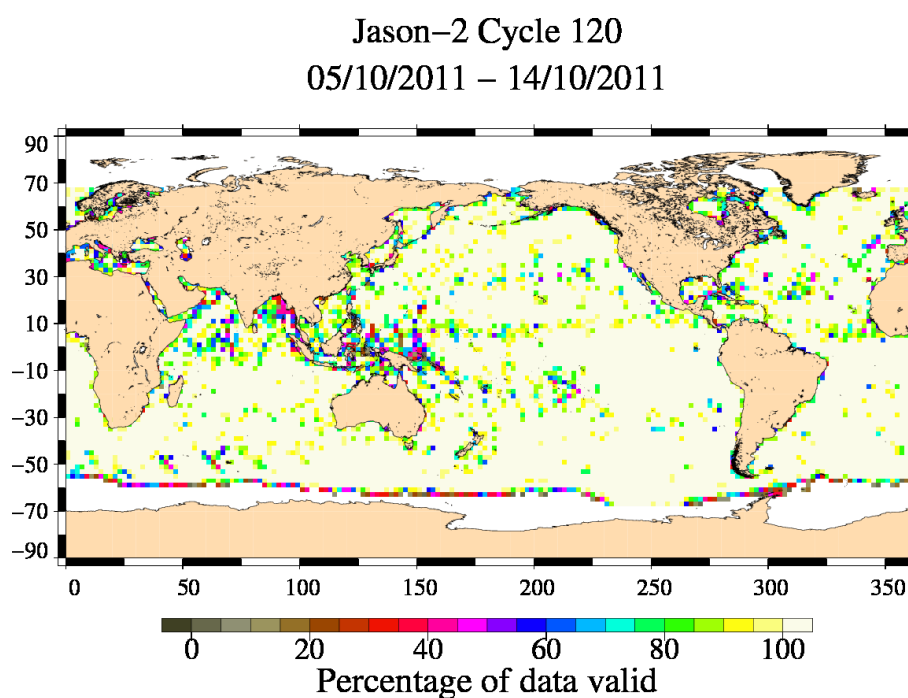
FIG. 3 – Percentage of valid measurements for cycle 120.
