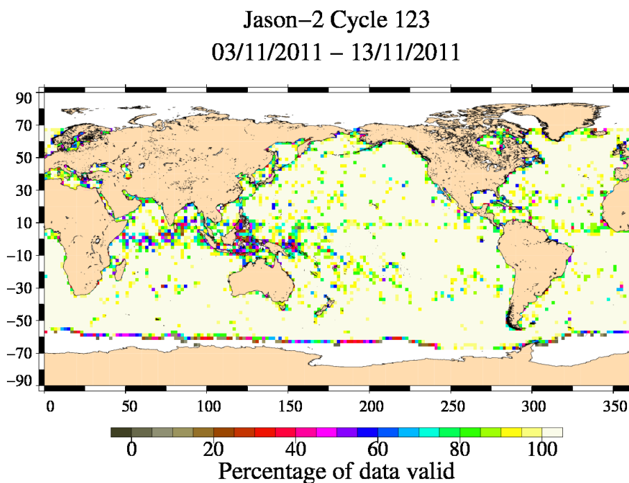
FIG. 3 – Percentage of valid measurements for cycle 123.
