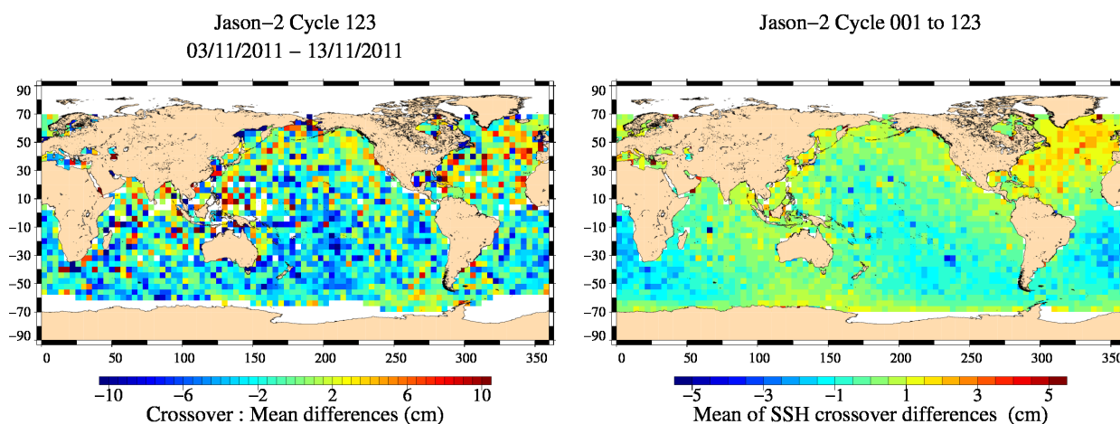
FIG. 13 – Mean SSH at crossovers for cycle 123 (left) and over the whole Jason-2 period (right).
