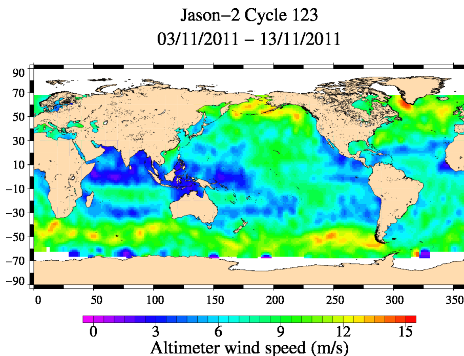
FIG. 9 – Altimeter wind speed for cycle 123.
