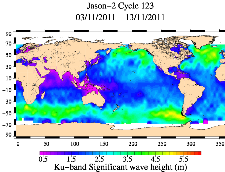
FIG. 5 – Significant wave height for cycle 123.
