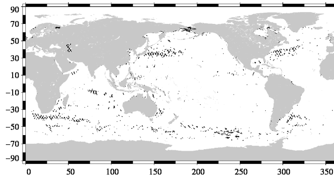
FIG. 19 – Differences higher than a 30 cm threshold for cycle 123.
