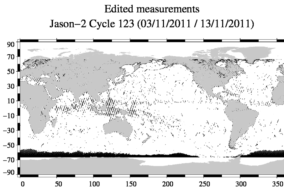
FIG. 2 – Edited measurements for cycle 123.
