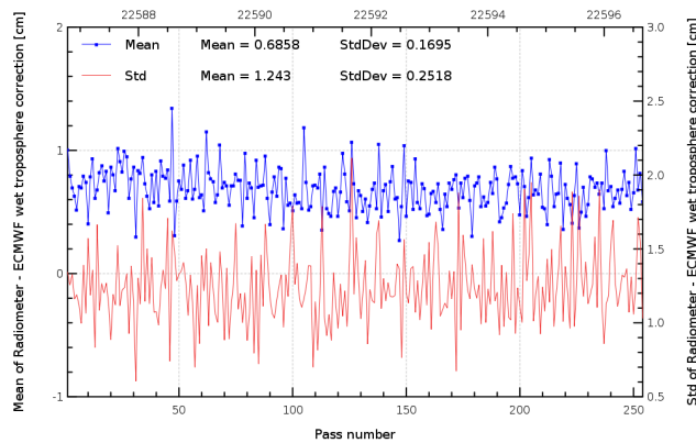
FIG. 11 – Pass monitoring of wet troposphere differences between radiometer and ECMWF model for Jason-2 cycle 123.
