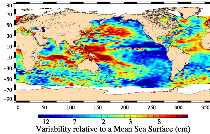
FIG. 18 – Sea level anomaly relative to MSS for cycle 123.
