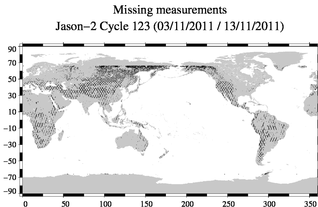
FIG. 1 – Missing measurements for cycle 123.
