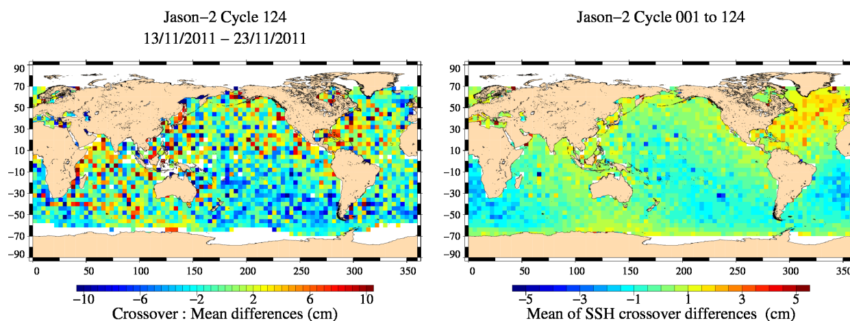
FIG. 14 – Mean SSH at crossovers for cycle 124 (left) and over the whole Jason-2 period (right).
