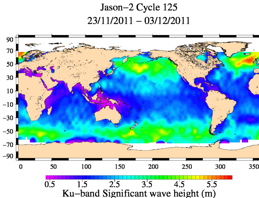
FIG. 5 – Significant wave height for cycle 125.
