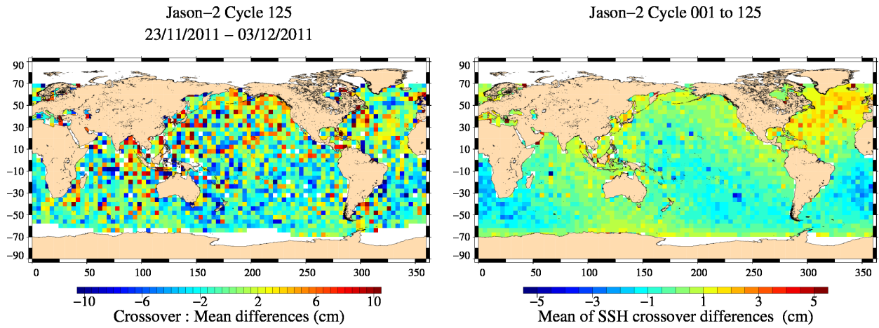
FIG. 13 – Mean SSH at crossovers for cycle 125 (left) and over the whole Jason-2 period (right).
