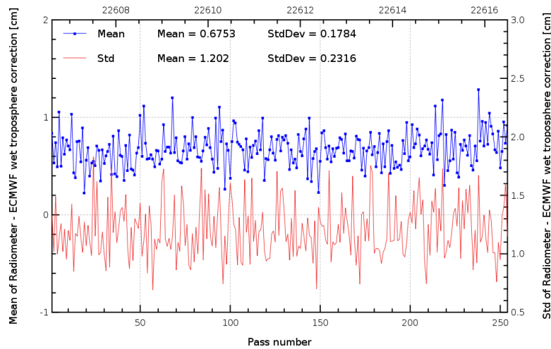
FIG. 11 – Pass monitoring of wet troposphere differences between radiometer and ECMWF model for Jason-2 cycle 125.
